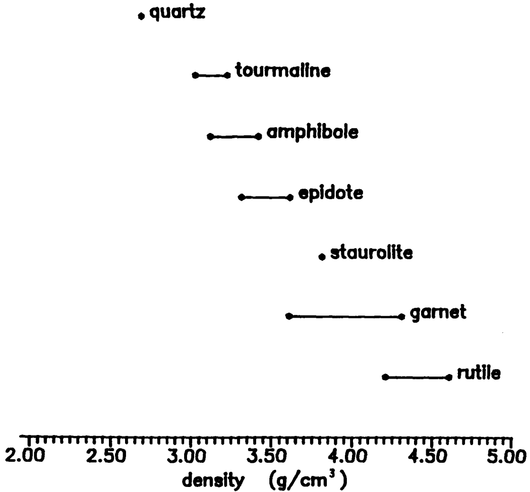
Figure 10. Approximate specific gravity ranges for mineral species considered in this report
