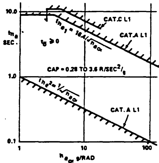
FIGURE 9 \tau_{n_z} vs. n/\alpha (Reference d)
