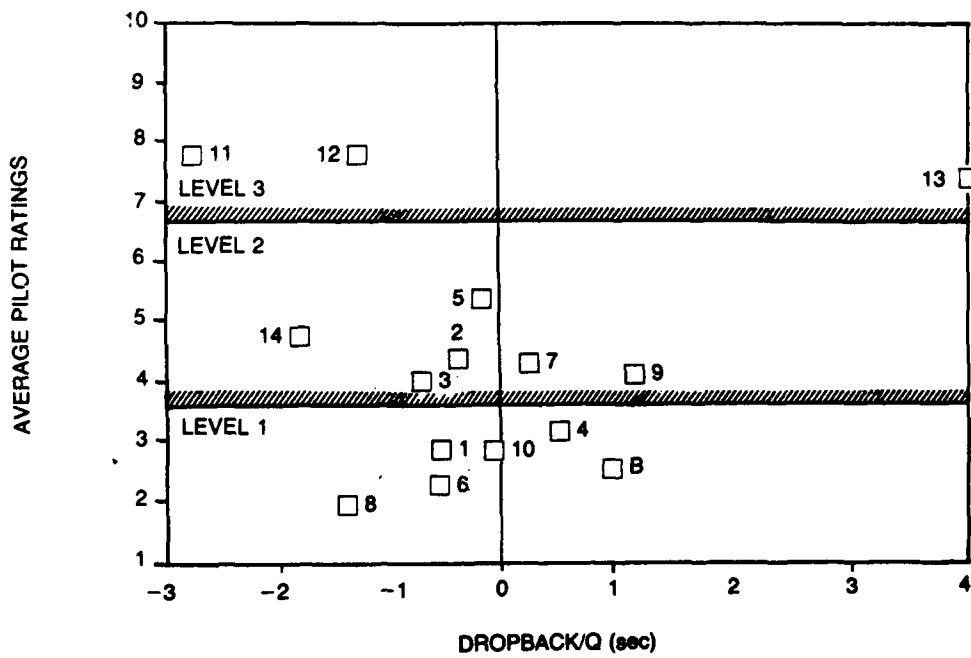
FIGURE 32 AVERAGE FLARED LANDING PILOT RATING vs DROPBACK/q
