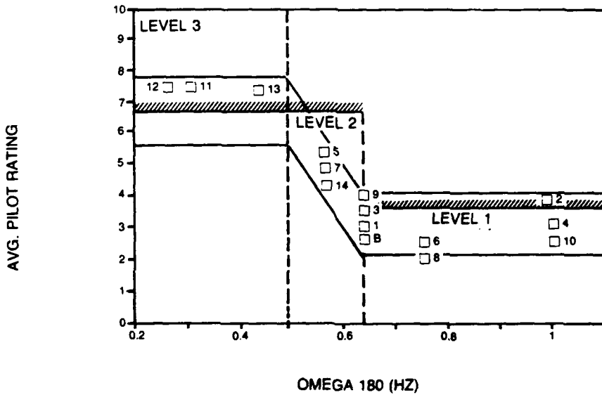
FIGURE 40 AVERAGE FLARED LANDING PILOT RATINGS VS \omega_{180}
