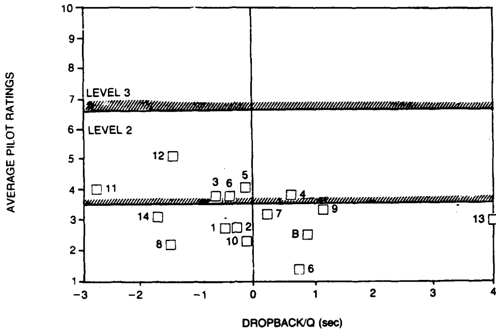
FIGURE 31 AVERAGE APPROACH PILOT RATING vs DROPBACK/q
