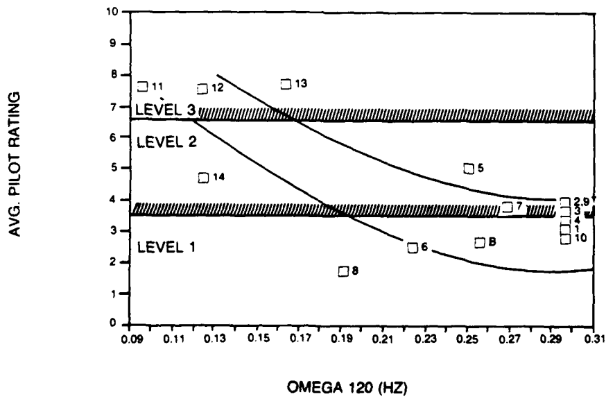
FIGURE 38 AVERAGE FLARED LANDING PILOT RATINGS VS \omega_{120}
