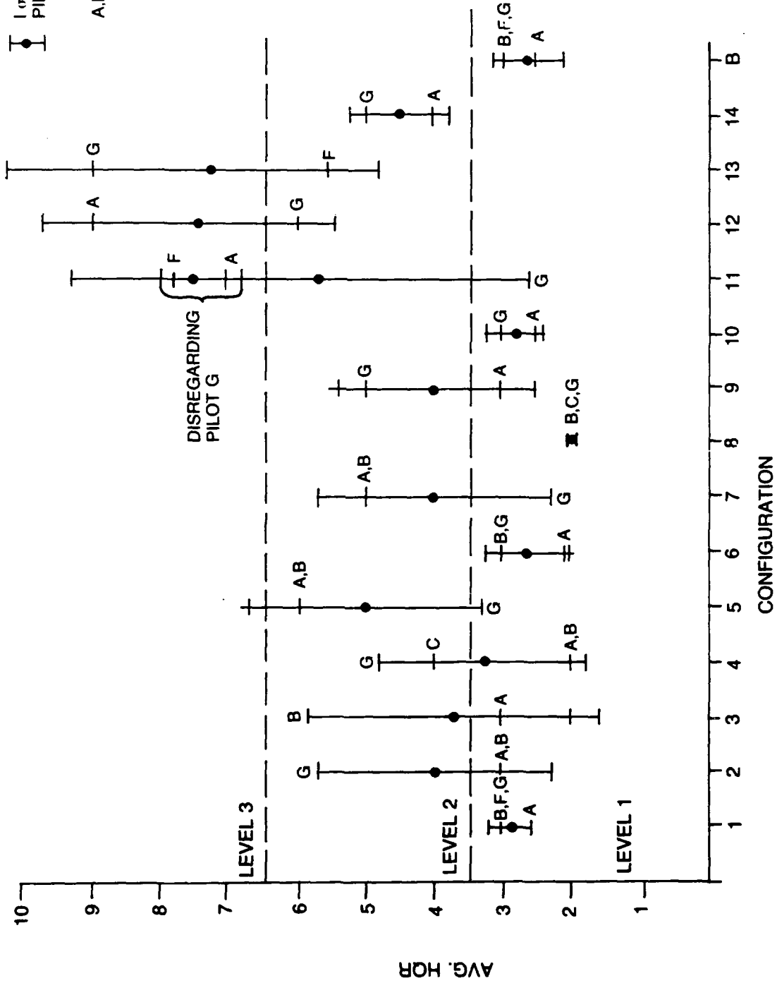
FIGURE 20 AVERAGE FLARED LANDING PILOT RATINGS
