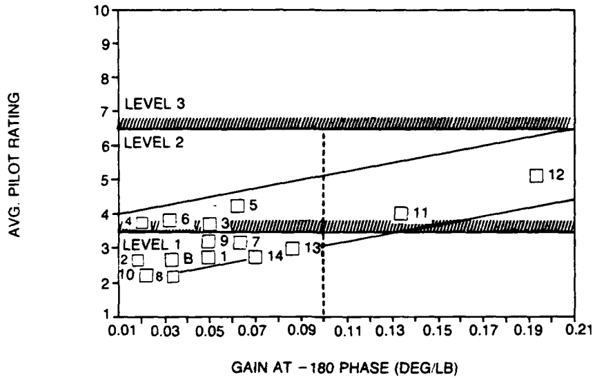
FIGURE 43 AVERAGE APPROACH PILOT RATINGS vs CROSSOVER GAIN
