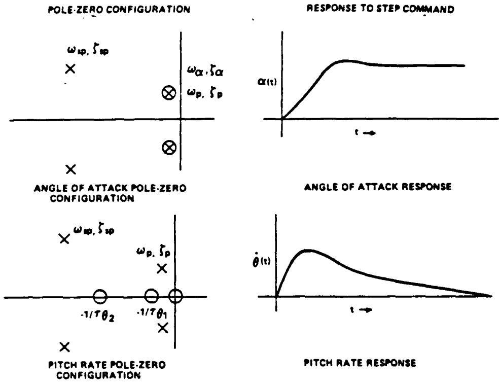
FIGURE 14 ANGLE OF ATTACK COMMAND SYSTEM (Reference b)
