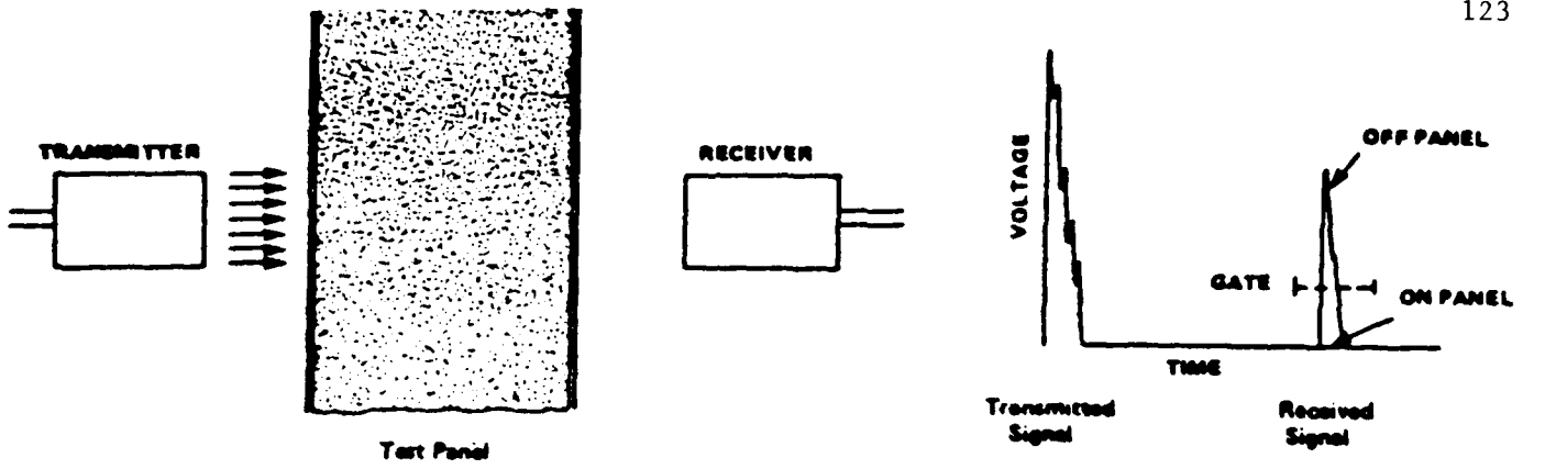
(a) THROUGH-TRANSMISSION
