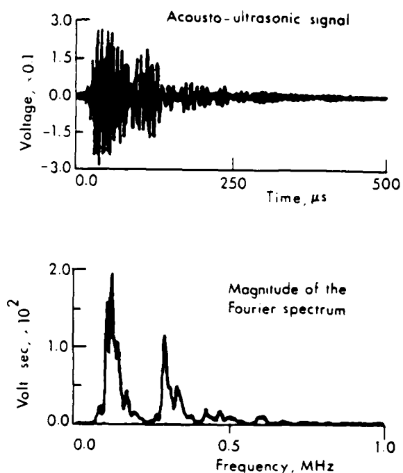
Fig. 2 Acousto-ultrasonic signal and the magnitude of its Fourier spectrum for a typical specimen.
