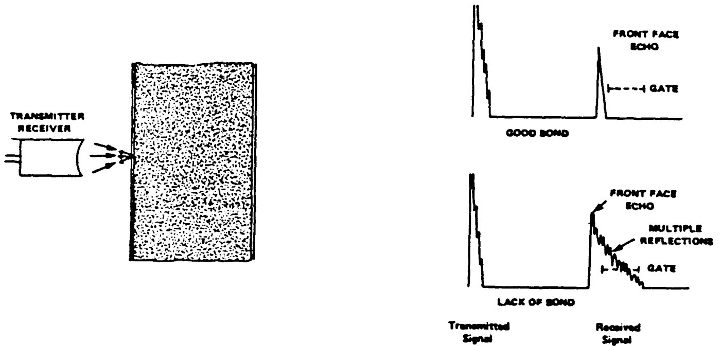
(b) PULSE-ECHO
