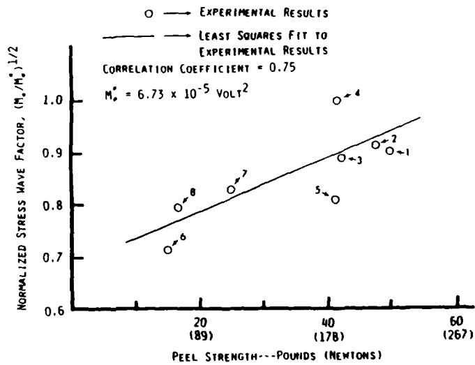
Fig. 4 Normalized stress wave factor, (M/M_0)^{1/2} , vs. peel strength for rubber sheet bonded to steel.
