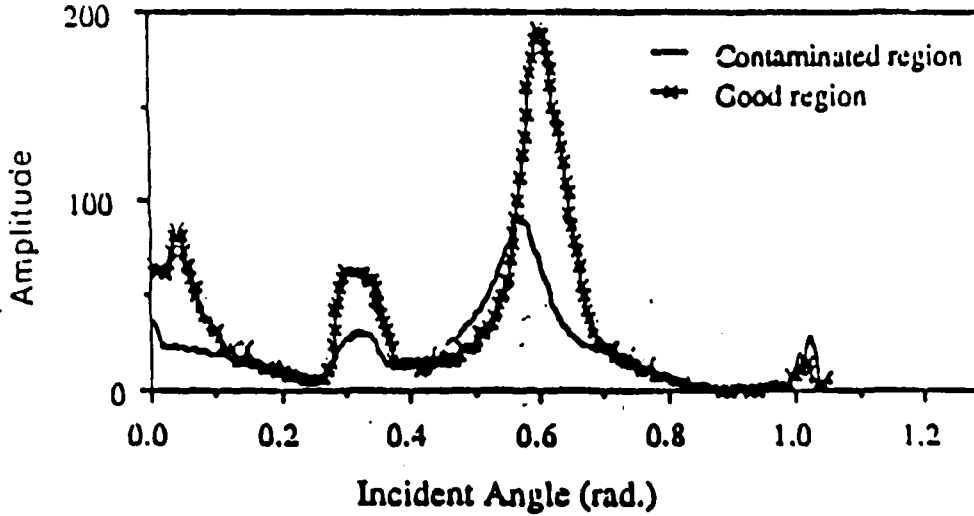
Fig 3b. The amplitude of the double through transmitted signal .vs. angle of incidence for a Al - Ep - Al problem with two different interfacial conditions. The maxima's represent the critical angles.
