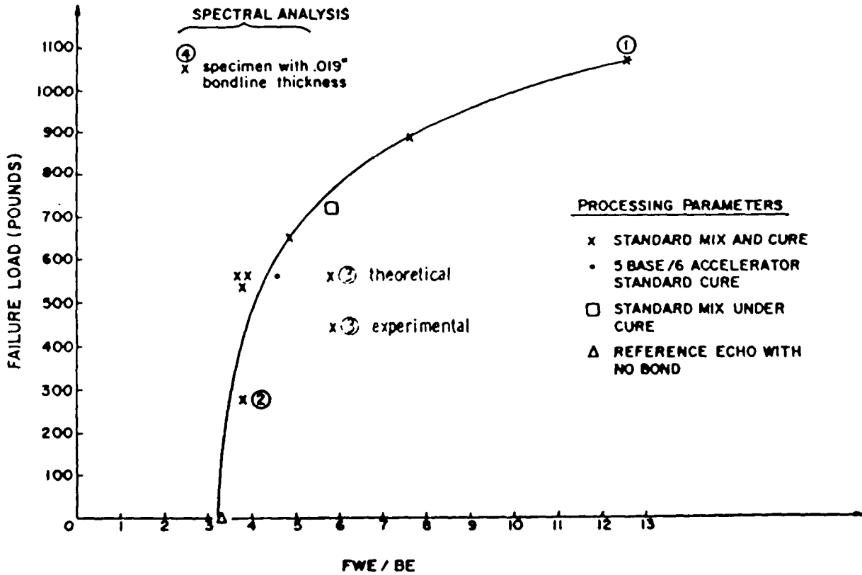
Fig. 3-Curve showing failure load versus FWE/BE for an aluminum-to-aluminum step-lap joint with 0.012 in. Scotch-Weld bondline thickness. (1 in. = 25.4 mm)
