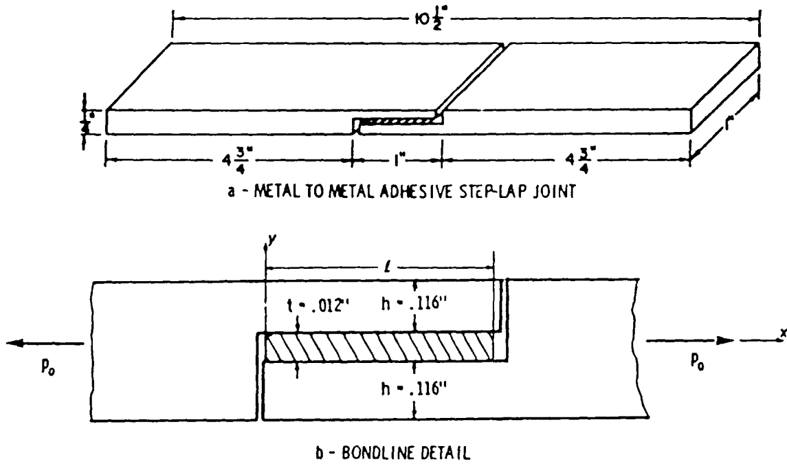
Fig. 1-Step-lap joint test specimen. (SI conversion: 1 in. = 25.4 mm)
