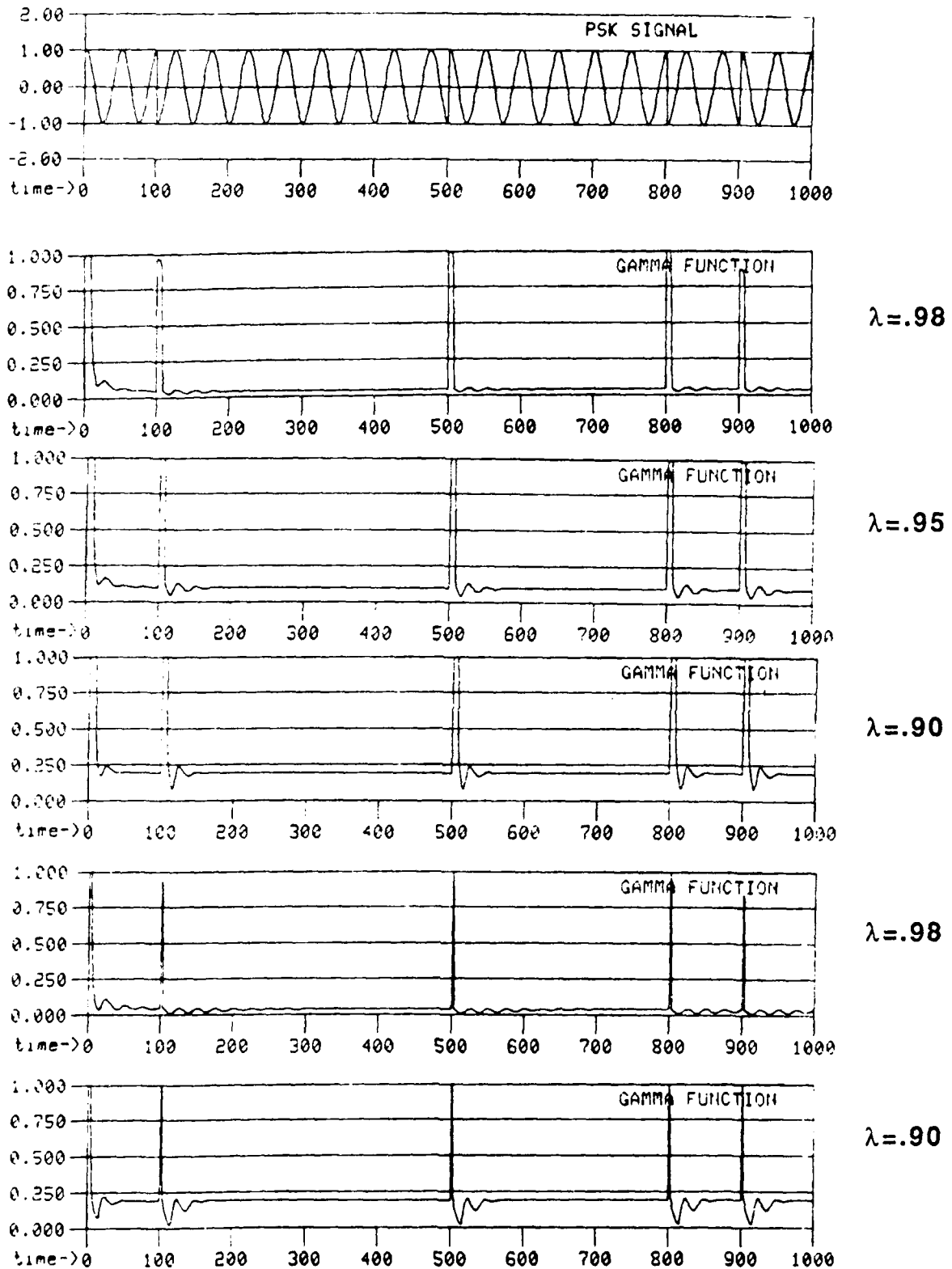
FIGURE 8: THE CARRIER FREQUENCY EFFECT. THE PSK SIGNAL AT THE TOP IS FOLLOWED BY THREE GAMMA FUNCTIONS FOR N=9 AND TWO GAMMA FUNCTIONS FOR N=3 FOR THE LAMBDA VALUES SHOWN.
