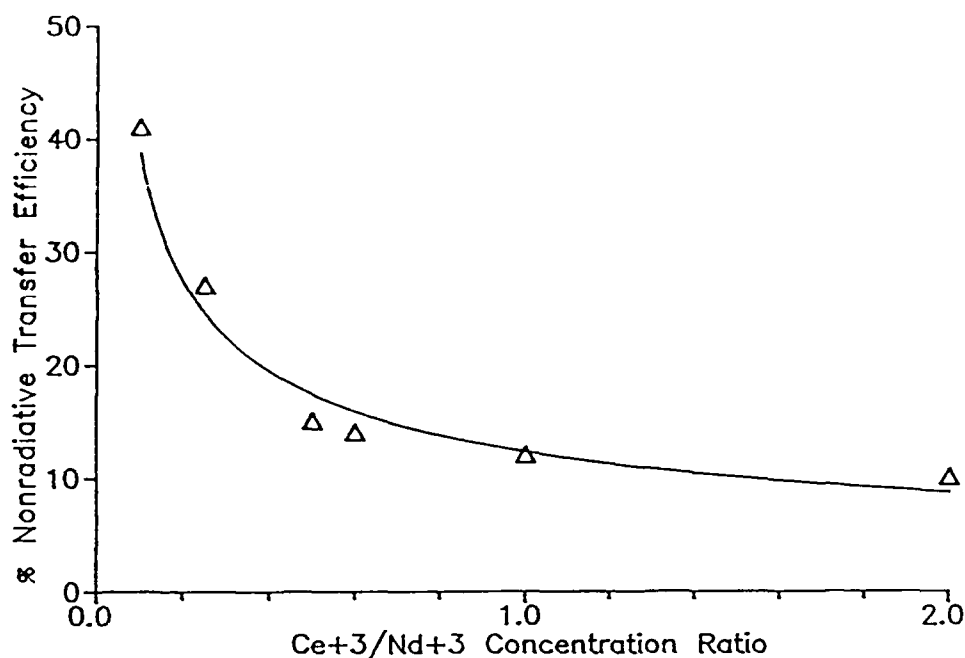
FIG. 3 Energy transfer efficiency as a function of Ce 3+ /Nd 3+ concentration ratio for Ce 3+ /Nd 3+ -β"-alumina.
