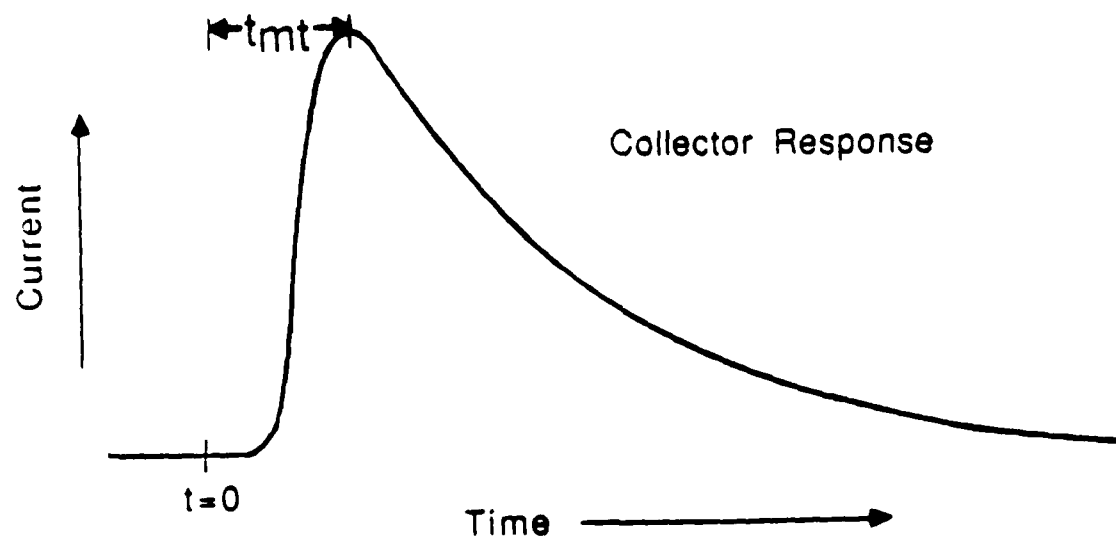
Scheme I. Experiment to measure diffusivity of electrogenerated species using a microelectrode array
