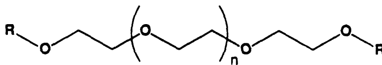
Poly(ethylene oxide)
