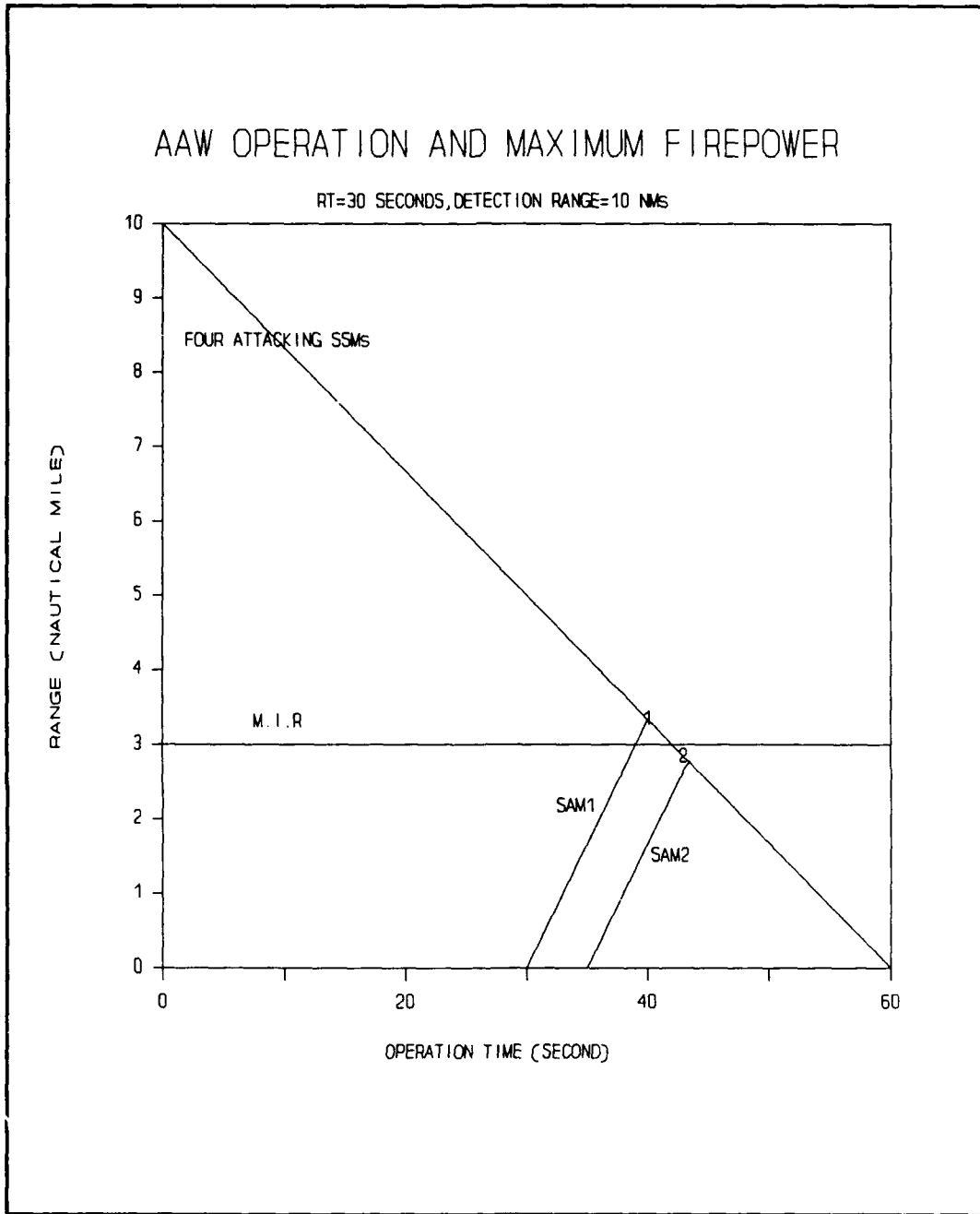
Figure 8. The AAW operation and maximum firepower at 10 NMs detection range. Impact point: "1"=(40, 3.33), "2"=(43.33, 2.78). Maximum firepower is one.
