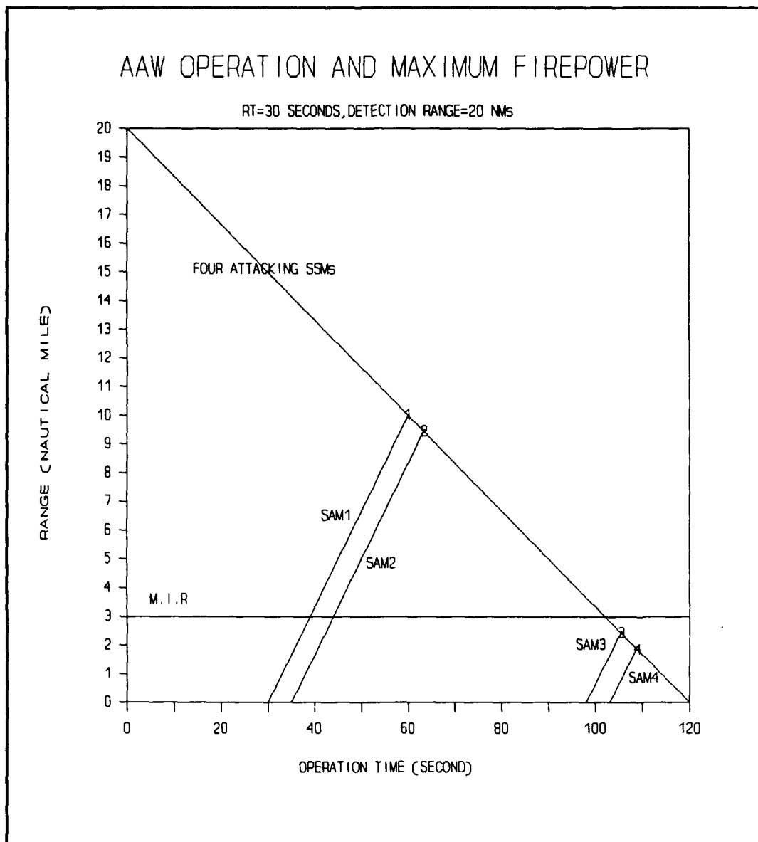
Figure 6. The AAW operation and maximum firepower at 20 NMs detection range. Impact point: "1"=(60, 10), "2"=(63.33, 9.44), "3"=(105.33, 2.44), "4"=(108.67, 1.89). "3" and "4" are not effective, thus the maximum firepower is two.
