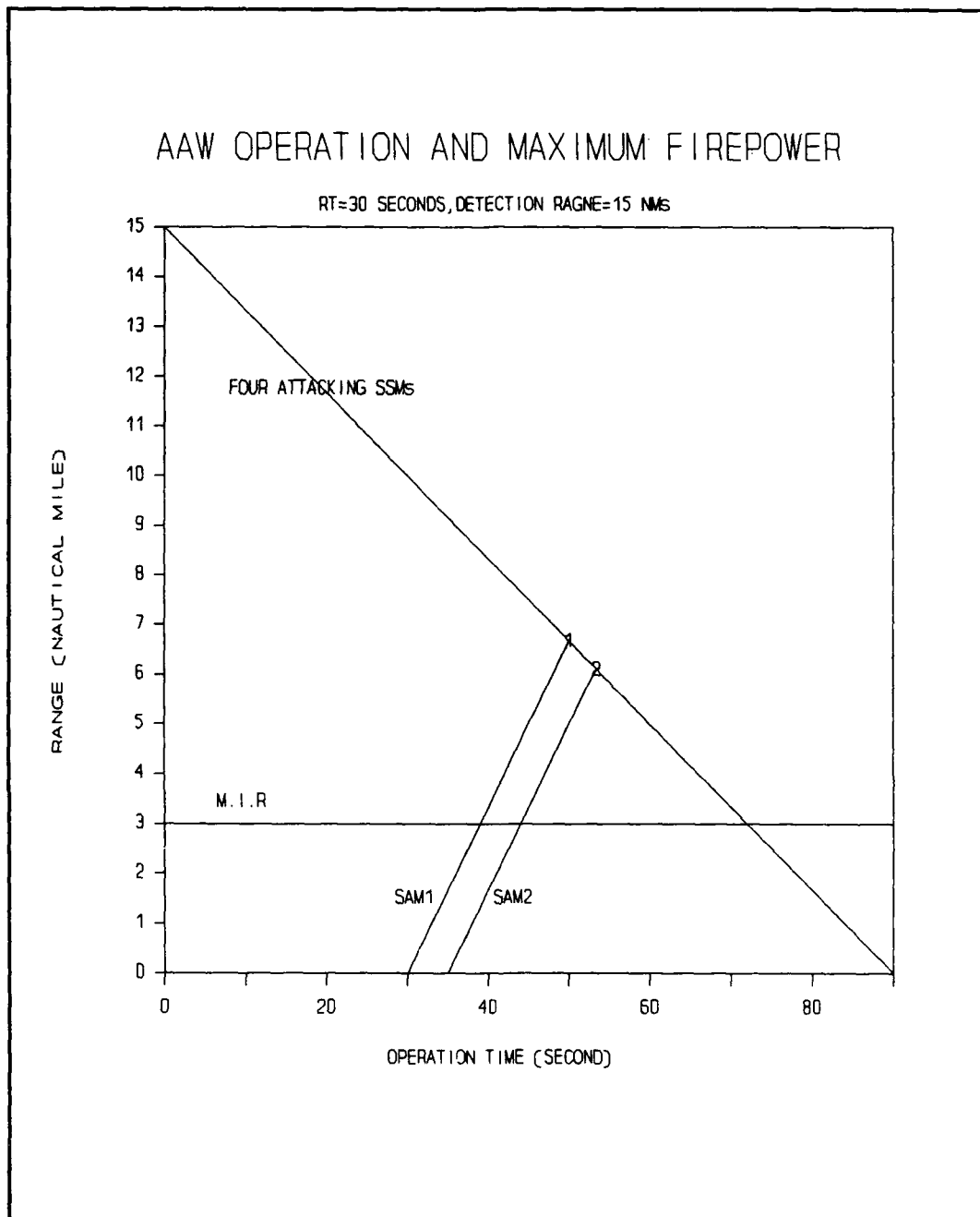
Figure 7. The AAW operation and maximum firepower at 15 NMs detection range. Impact point: "1"=(50, 6.67), "2"=(53.33, 6.11). Maximum firepower is two.
