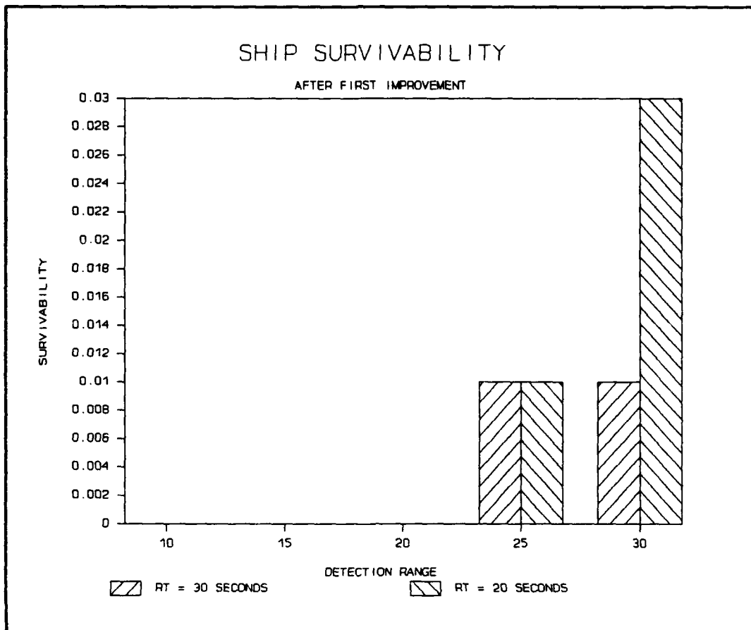
Figure 13. Ship survivability at the first two states.
