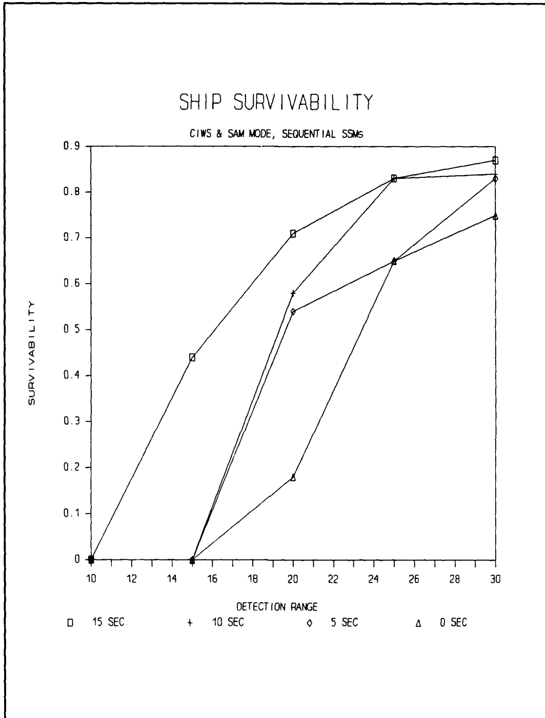
Figure 28. The improved weapon system vs. four sequential attacking SSMS.
