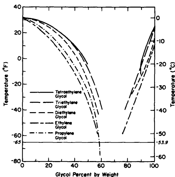
Figure 3. Comparison of freezing points of various glycols.
