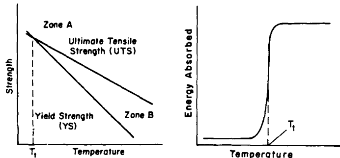
a. Ultimate tensile and yield strength vs temperature. T_t = transition temperature (see Fig. 2c and d for zone A and B).
