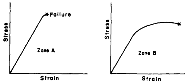
c. Stress-strain curve for material near or below transition temperature. Failure mode is brittle fracture.
