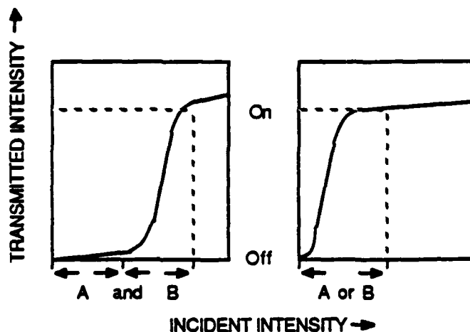
Fig. 8 Implementing Boolean Connectives
