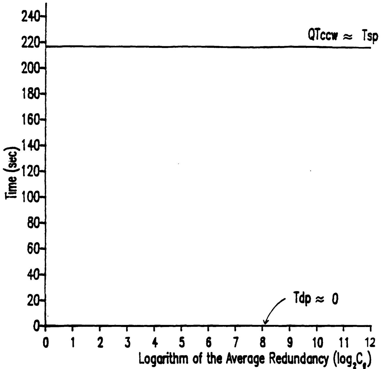
Figure 9.3.4 Components of the SCW Query Response Time ( S_{db}=10^8 bytes, A_r=6 , R_q=2 , F_D=9 )
