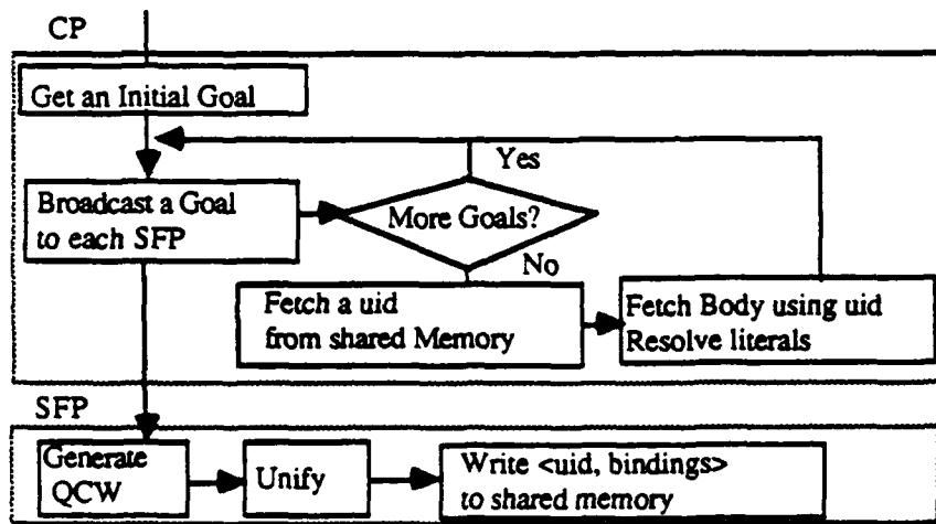
Fig. 5 Logic Programming Evaluation based on Surrogate Files
