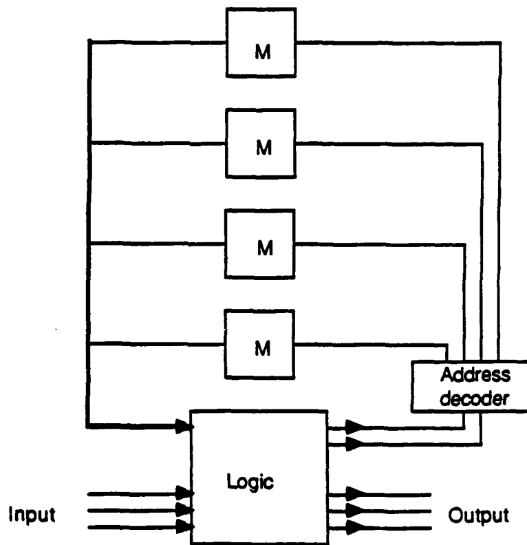
Fig. 9 Finite State Machine with von Neumann bottleneck
