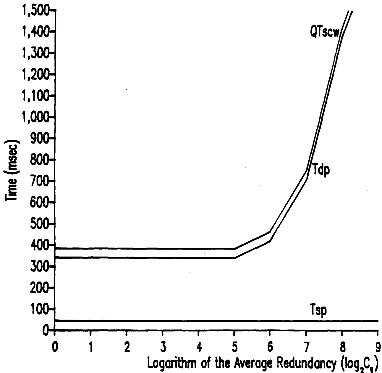
Figure 9.3.3 Components of the SCW Query Response Time ( S_{db}=10^5 bytes, A_r=6 , R_q=2 , FD=9 )
