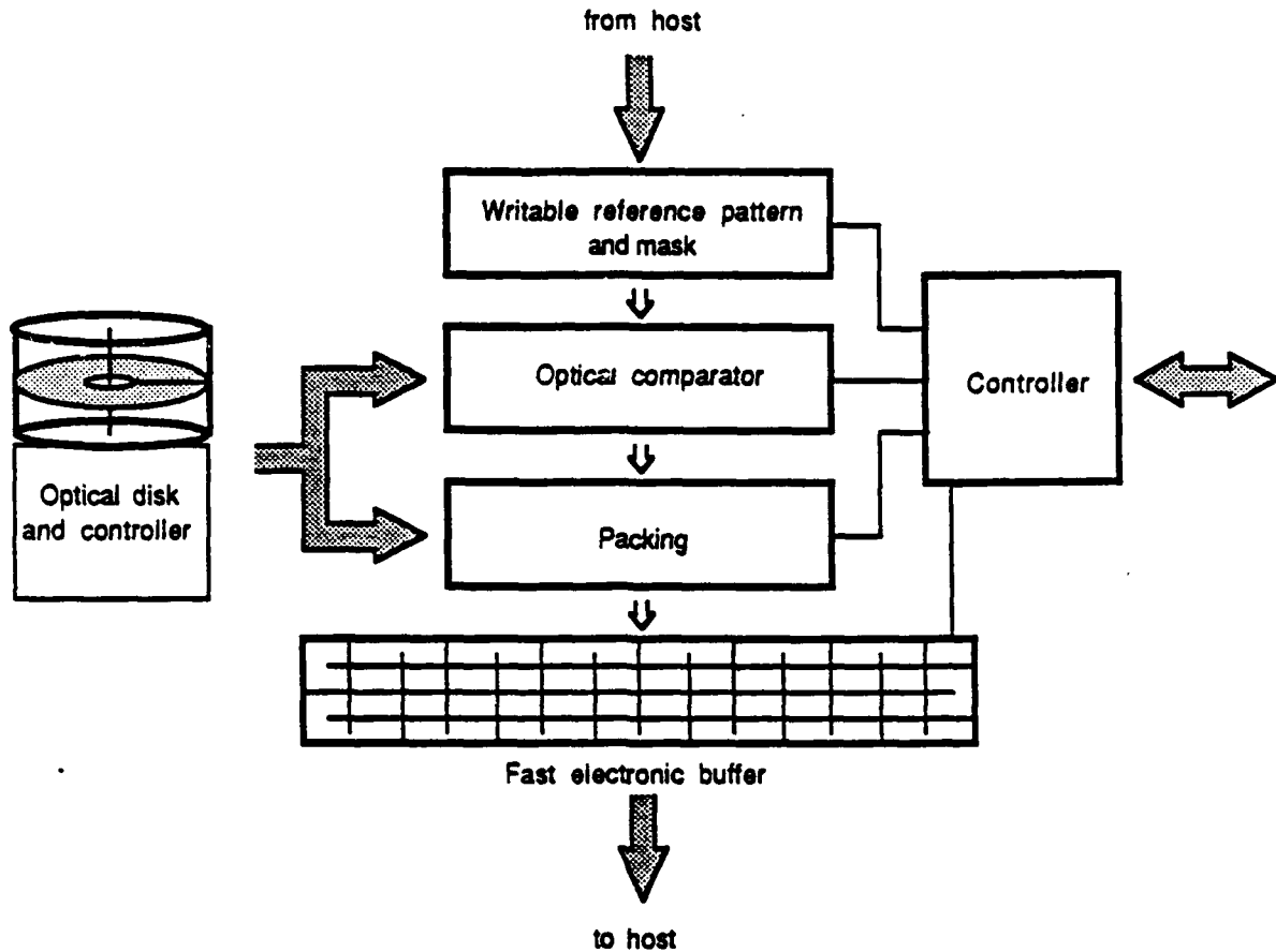
Fig 13 Block diagram of a hybrid opto-electronic preprocessor
