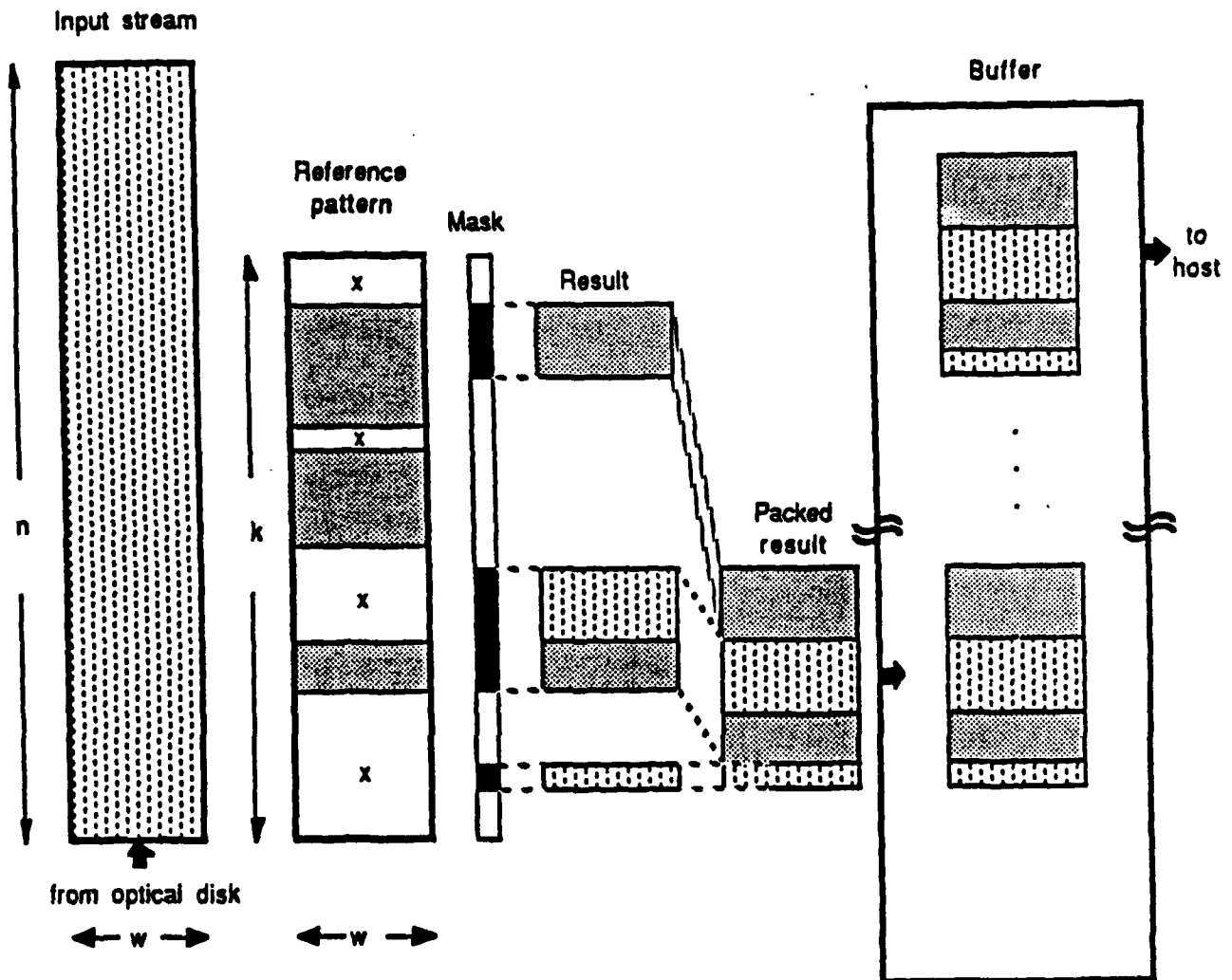
Figure 9.7.4 Processing sequence. Input data from the optical disk is filtered and the results are placed in a large, fast electronic buffer.
