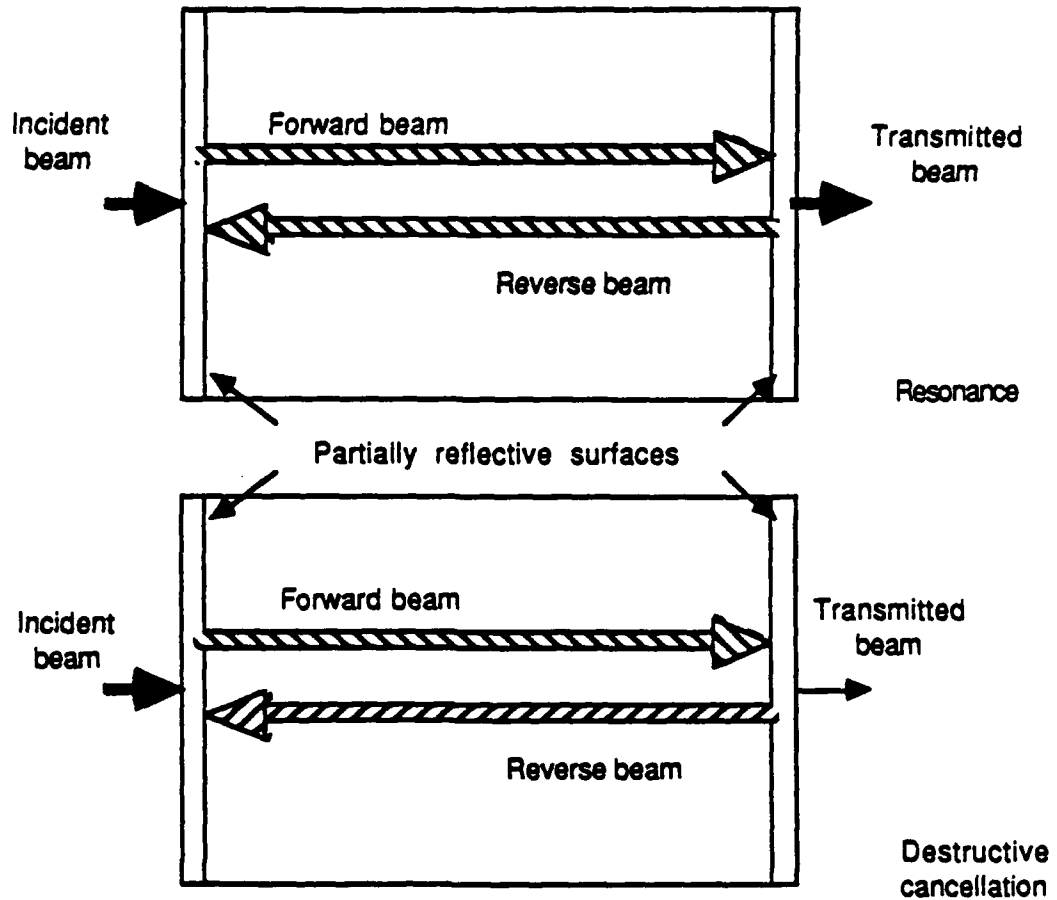
Fig. 5 Fabry-Perot cavity
