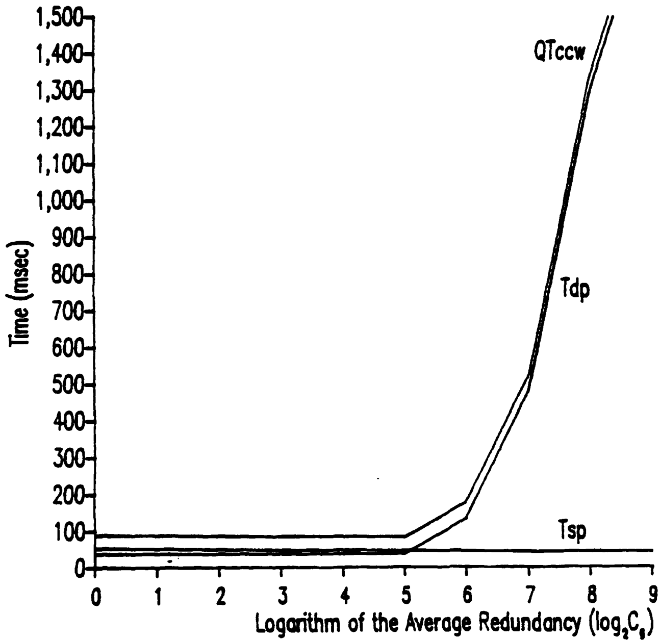
Figure 9.3.5 Components of the CCW Query Response Time ( S_{db}=10^3 bytes, A_r=6 , R_q=2 )
