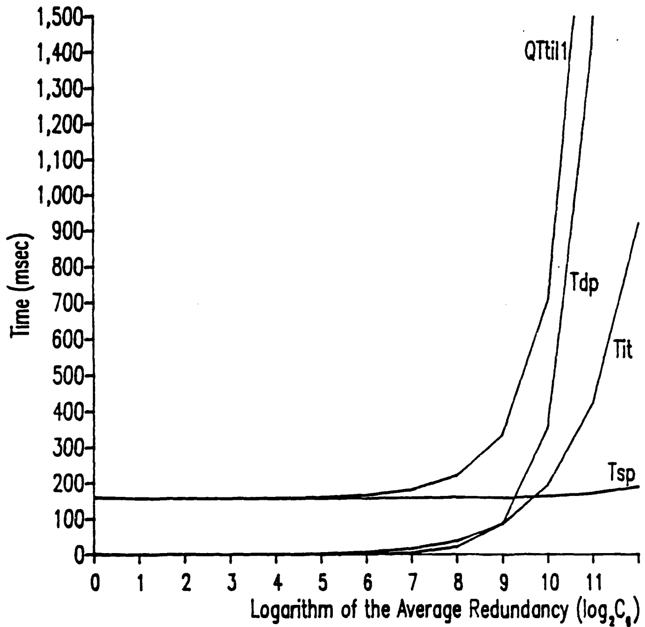
Figure 9.5.5 Components of the TL1 Query Response Time (Sdb=10 bytes, Ar=6, Rq=2).
