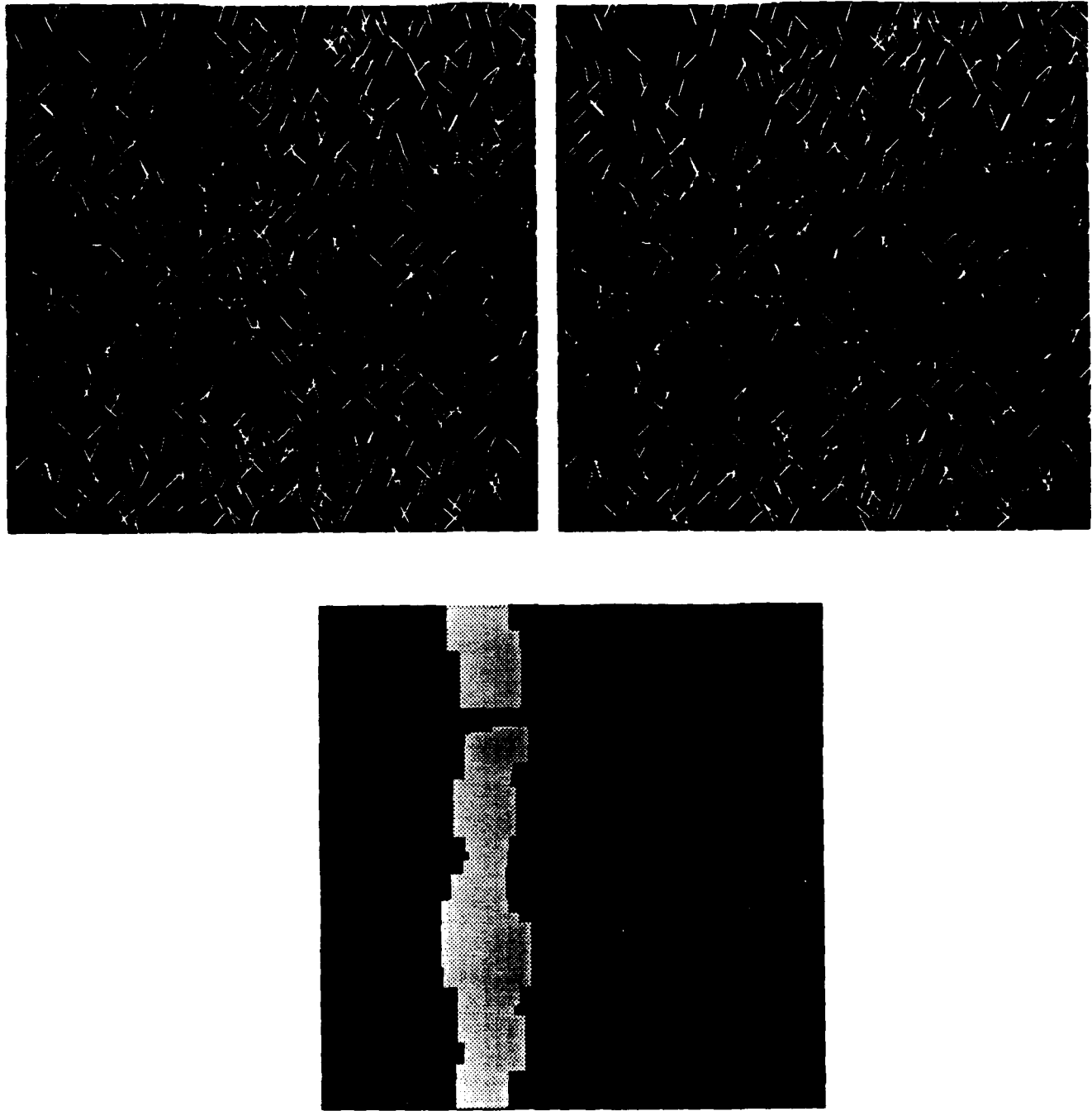
Figure 2.8: Results of a computer experiment with the proposed method for recovering the discontinuities of planar surfaces. The top half of the figure displays a random line stereogram corresponding to the input disparity information. The disparity corresponds to a central planar region that has been rotated about a vertical axis by 45^\circ . The bottom half of the figure shows the recovered regions of discontinuity. The recovered depth from the viewer is displayed in terms of grey levels with black the furthest and white the closest.
