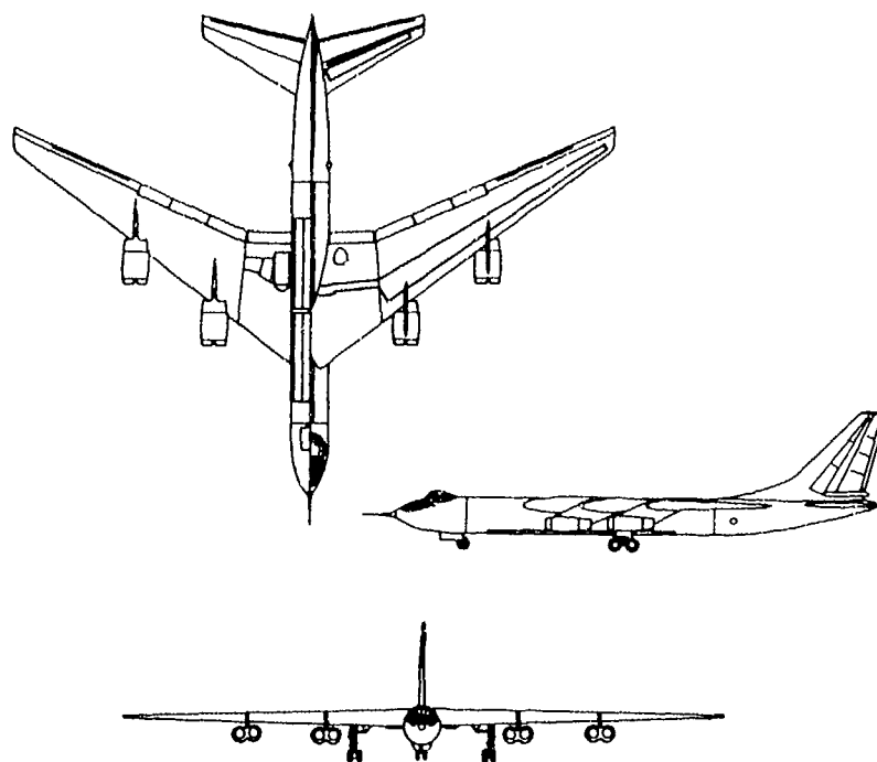
The prototype YB-60, a reconfigured B-36 with jet engines and swept-back wings.
