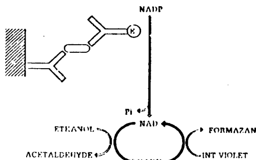
Figure 11. NAD/NADH cycle.
