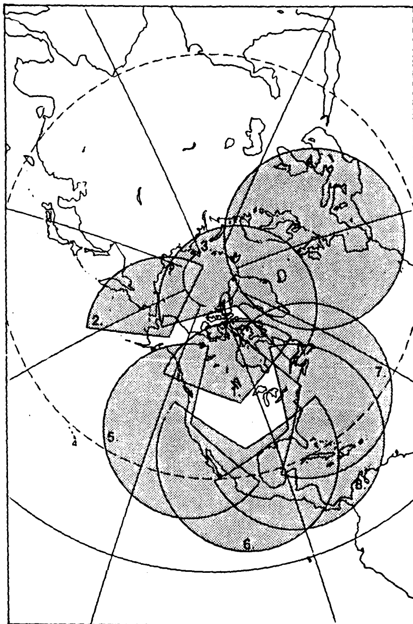
1. PARCS; 2. BMEWS, Clear, Alaska; 3. BMEWS, Thule, Greenland; 4. BMEWS, Fylingdales, England; 5. PAVE PAWS, Beale AFB, California; 6. PAVE PAWS, Goodfellow AFB, Texas; 7. PAVE PAWS, Cape Cod AFS, Massachusetts; 8. PAVE PAWS Robins AFB, Georgia. Figure shows 1,000-km altitude detection contours.
