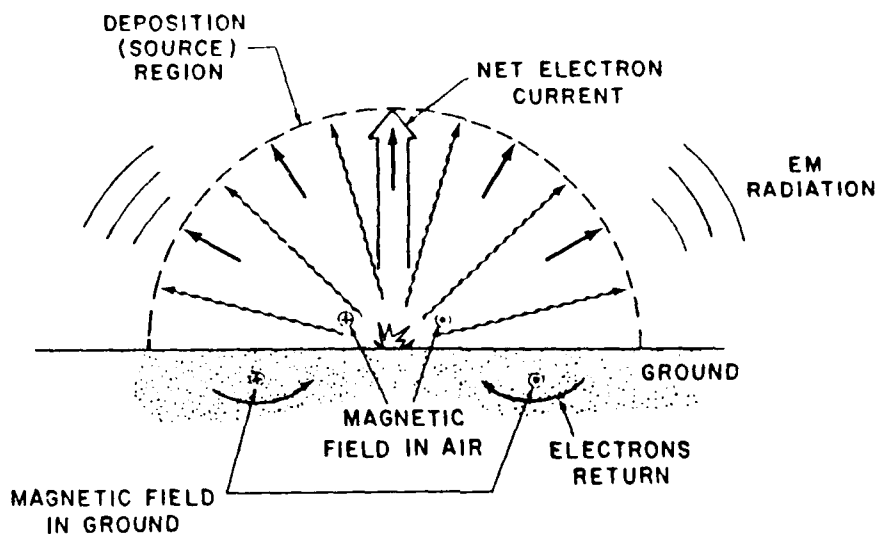
Figure 5-4. Surface Burst Deposition Region
