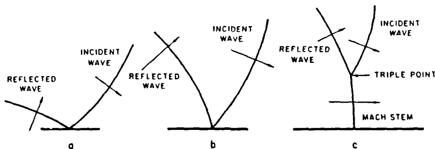
Figure 5-3. Triple Point Shock Wave or "Mach Y"
