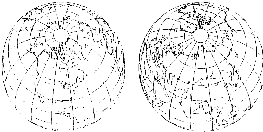
Figure 4-4. Coverage Area As Observed From A Satellite In A Molniya Orbit
