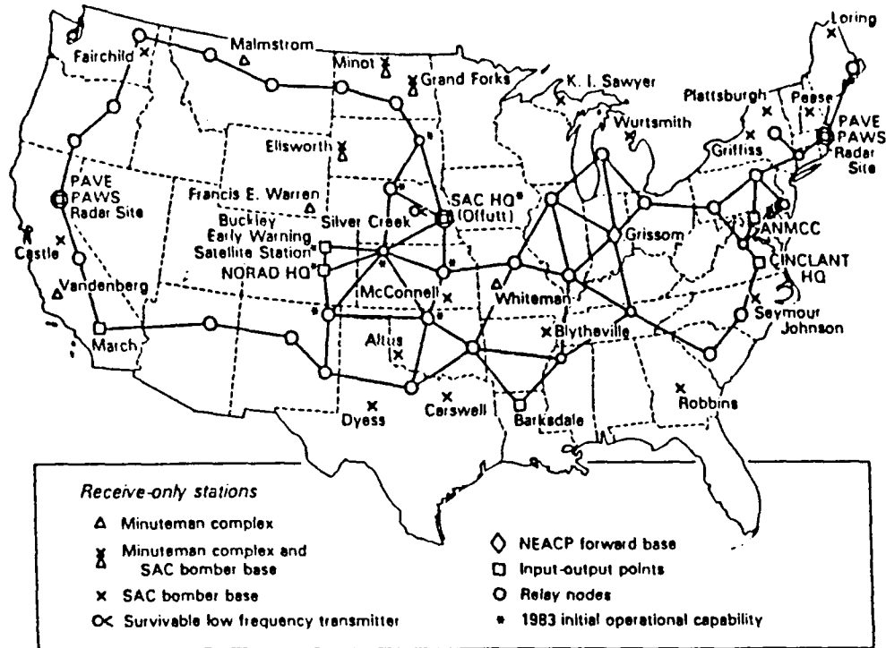
Figure 3-5. Ground Wave Emergency Network (GWEN) Thin-Line System
