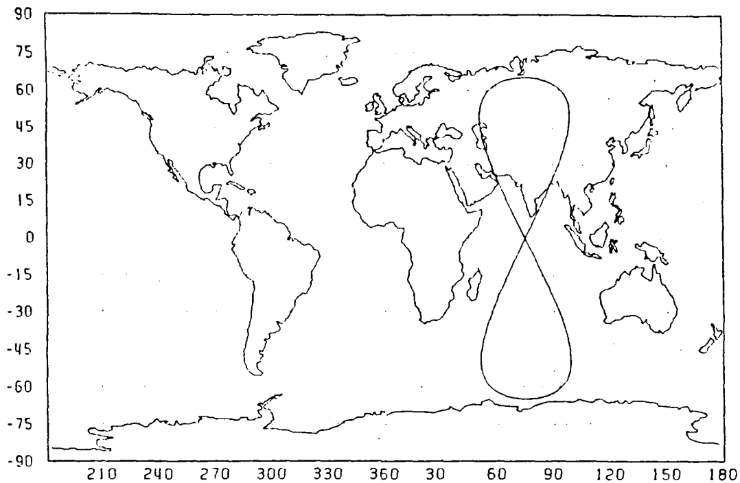
Figure 4-5. Ground Trace Path of a Geosynchronous Satellite
