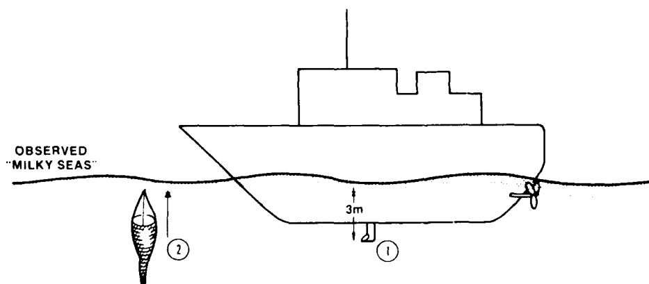
Fig. 2. Seawater sampling schemes used for onboard photometer system and collecting luminous plankton in this study: (1) sea-chest intake 3 m below sea surface, and (2) 53\text{-}\mu\text{m} plankton net pulled up from below and through sea surface collecting surface populations.
