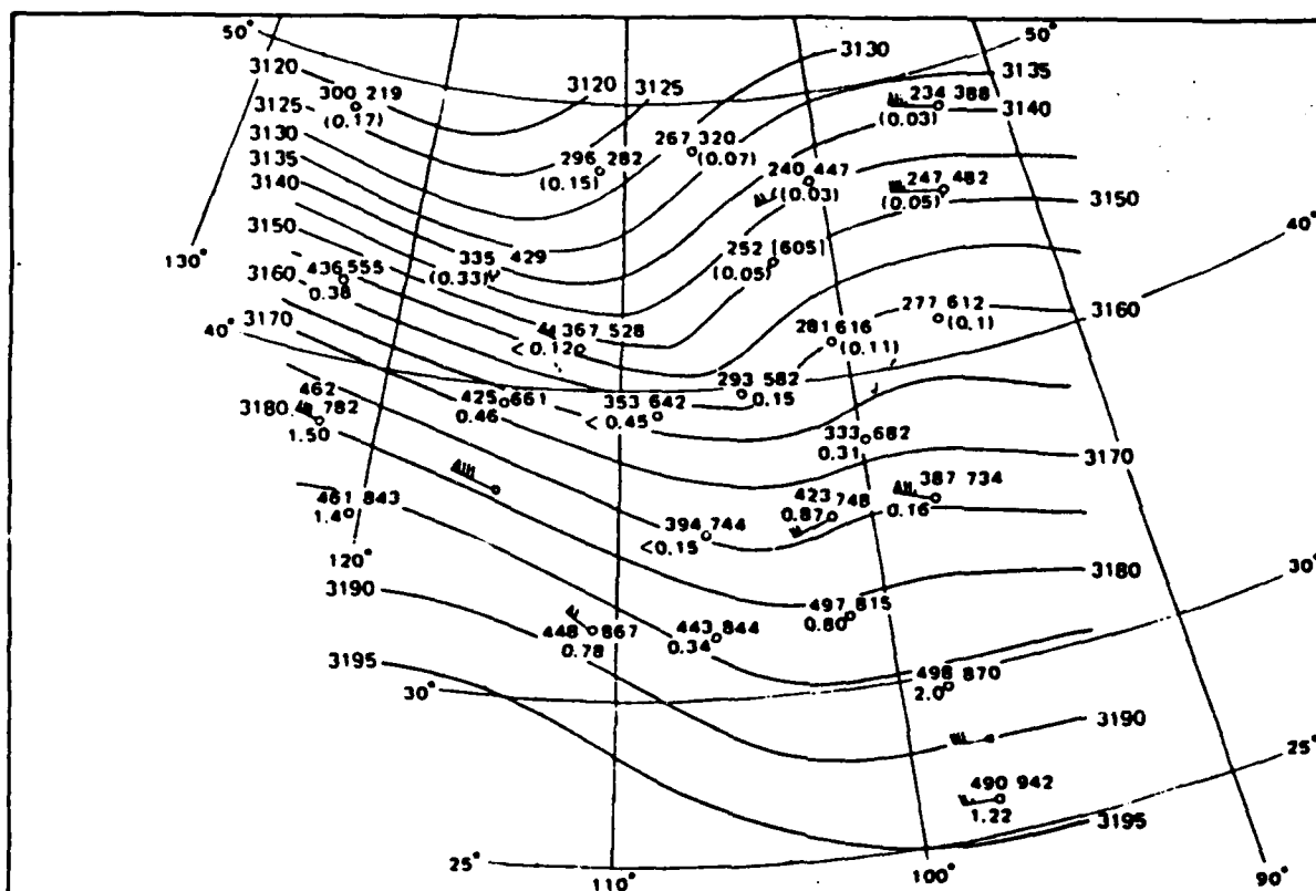
Figure 26a. Isentropic surface, \theta=45^{\circ}\text{C} , 0300 GMT 8 January 1953. Numerical values to the left of each station indicate pressure (mb) and specific humidity (gm/kg); to the right are the last three digits of the Montgomery streamfunction (M). Isolines of M are labeled in units of 10^6 \text{ m}^2 \text{ s}^{-2} (Danielsen and Reiter, 1960).
