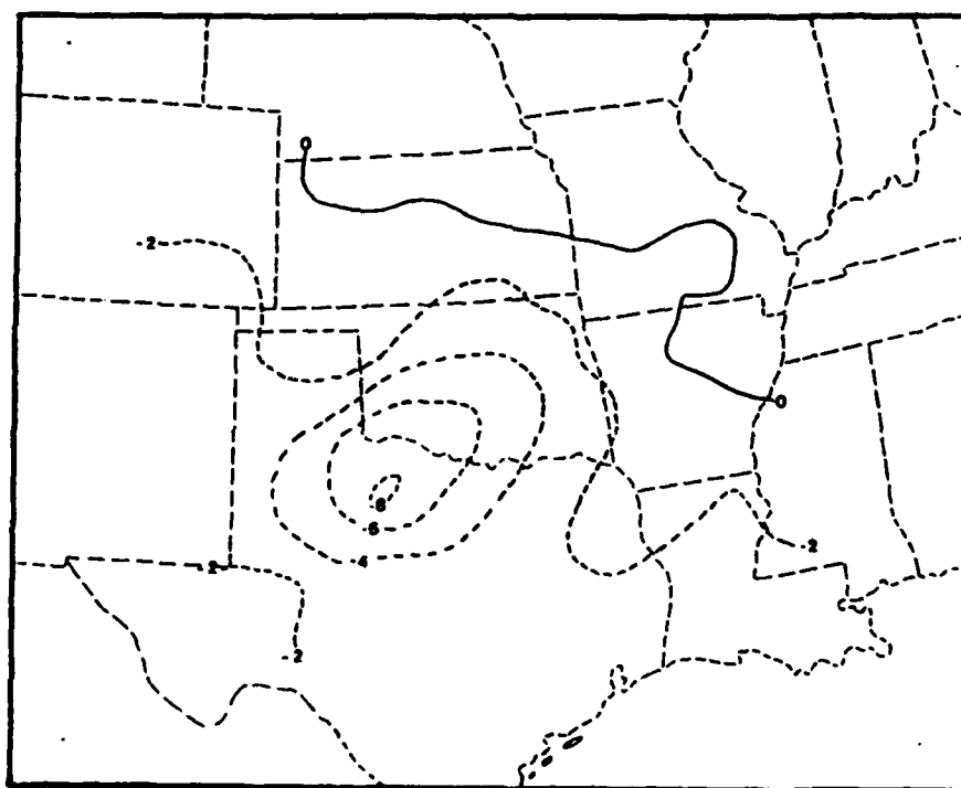
Figure 28b. 312 K 3-hour delta M field for 1700-2000 GMT 10 April 1979 (Rubino, 1986). Units are \text{J/kg} \times 10^5 .
