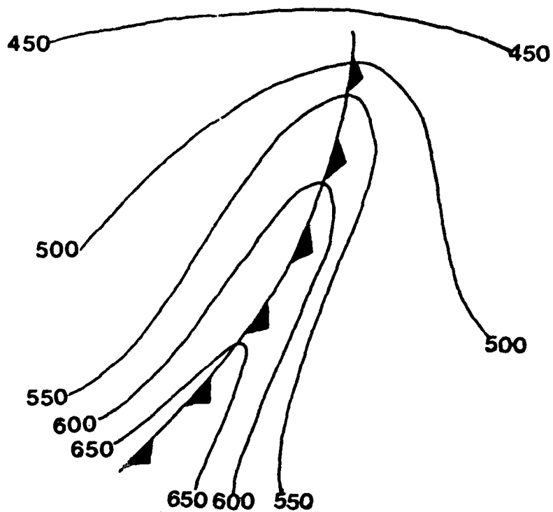
Figure 23a. Isentropic condensation pressure pattern over a mature, strong cold front (Anderson, 1984).
