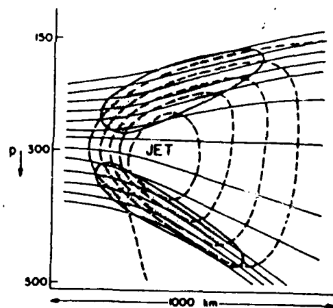
Figure 32. Schematic illustration of regions of clear-air turbulence (stippled) in the vicinity of an upper-level jet core and frontal zone. Solid and dashed lines respectively indicate potential temperature and wind speed (Shapiro, 1976).
