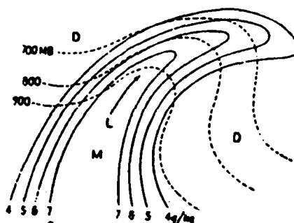
Figure 13. Illustrating probable upslope motion of a moist current as deduced from the relation of the moisture lines to the isobars on an isentropic surface (Namias, 1940).
