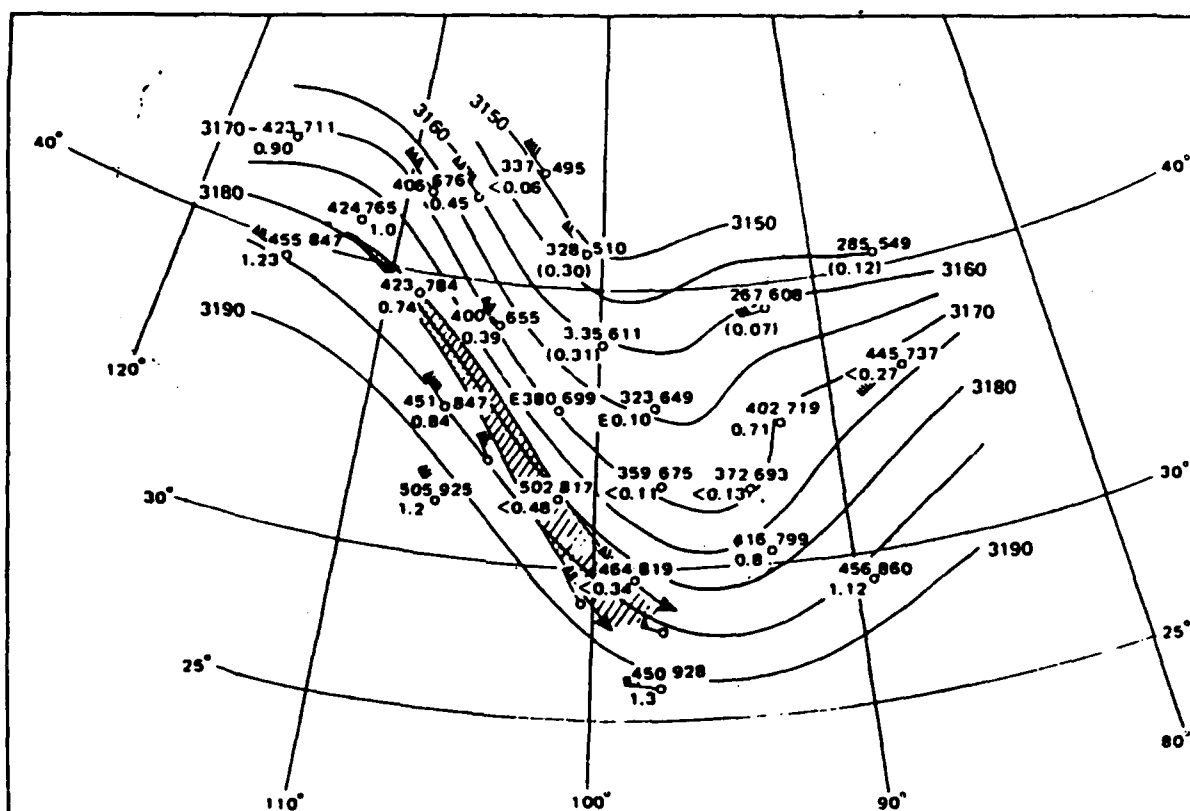
Figure 26b. Isentropic surface, \theta=45^{\circ}\text{C} , 1500 GMT 8 January 1953. Trajectories are shown for the time period 0300-1500 GMT on that day. The spread between the two trajectories allows for inaccuracies in wind reports (Danielsen and Reiter, 1960).
