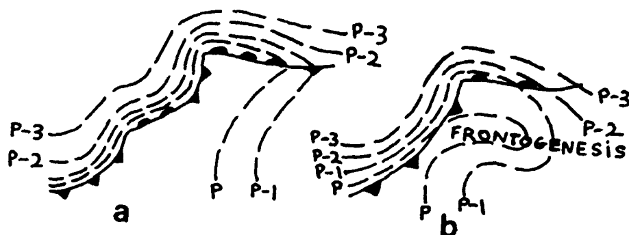
Figure 10. Isobaric topography in the vicinity of fronts (a) and isobaric topography associated with frontogenesis in the warm sector (b) (Namias, 1940).
