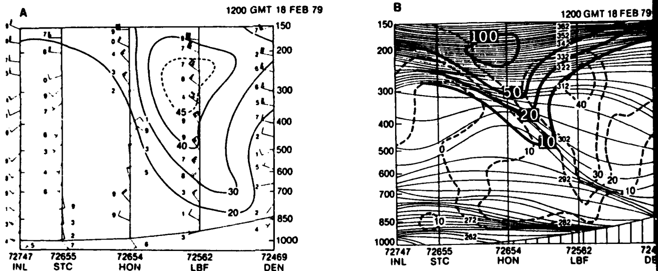
Figure 30a-b. Vertical cross section from International Falls, MN (INL) to Denver, CO (DEN) for 1200 GMT 18 February 1979. The left panel (A) is an isobach analysis for total wind speed ( \text{m s}^{-1} ); wind barbs plotted with last digit of wind observation. The right panel (B) shows isentropes (solid, K); geostrophic wind (dashed, \text{m s}^{-1} ) computed from the horizontal thermal gradient in the plane of the cross section; potential vorticity, -(\zeta + f)/(\partial\theta/\partial p) , heavy solid, where 10 = 10 \times 10^{-6} \text{ K mb}^{-1} \text{ s}^{-1} . Potential vorticity analysis is only shown for upper portion of frontal zone and stratosphere (Uccellini, et al. , 1985).
