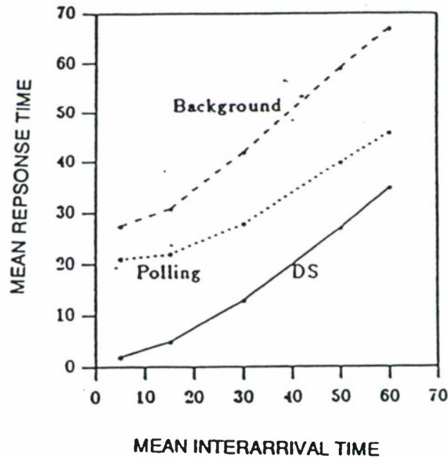
Figure 4-1: Scheduling Both Aperiodic and Periodic Tasks
