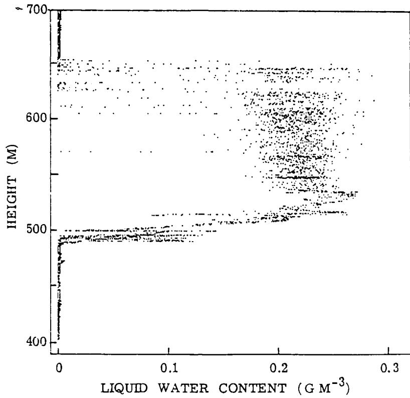
Fig.10 Liquid water content on the ascent of flight 239 during strato-cumulus dissipation.
