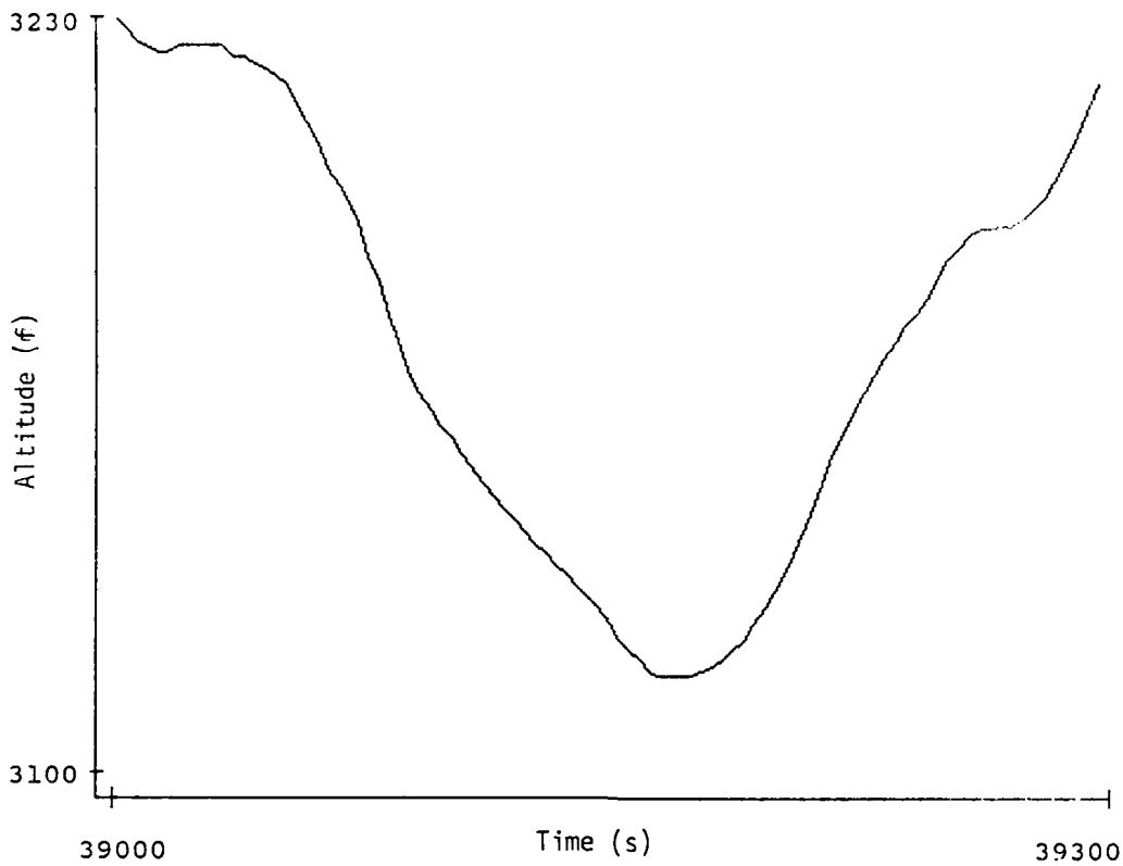
Fig. 9 Data in figure 8 smoothed with a five point running average.
