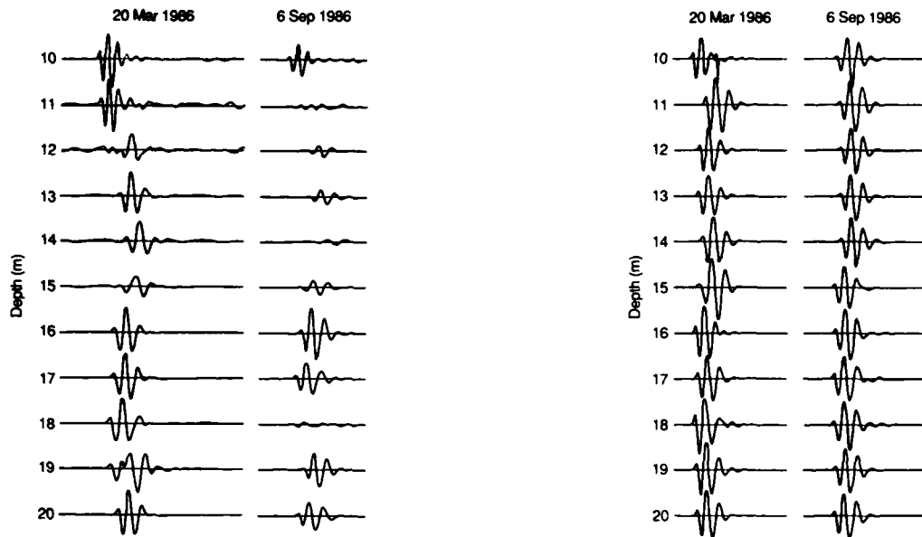
a. Waveforms transmitted between holes F2 and F6 (805 cm).
