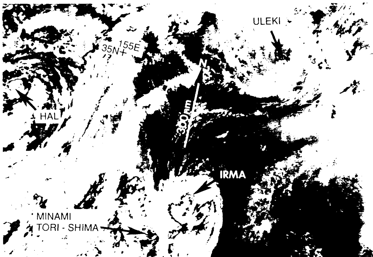
Figure 3-01C-3. Uleki dissipating over water (142247Z September DMSP infrared imagery).
