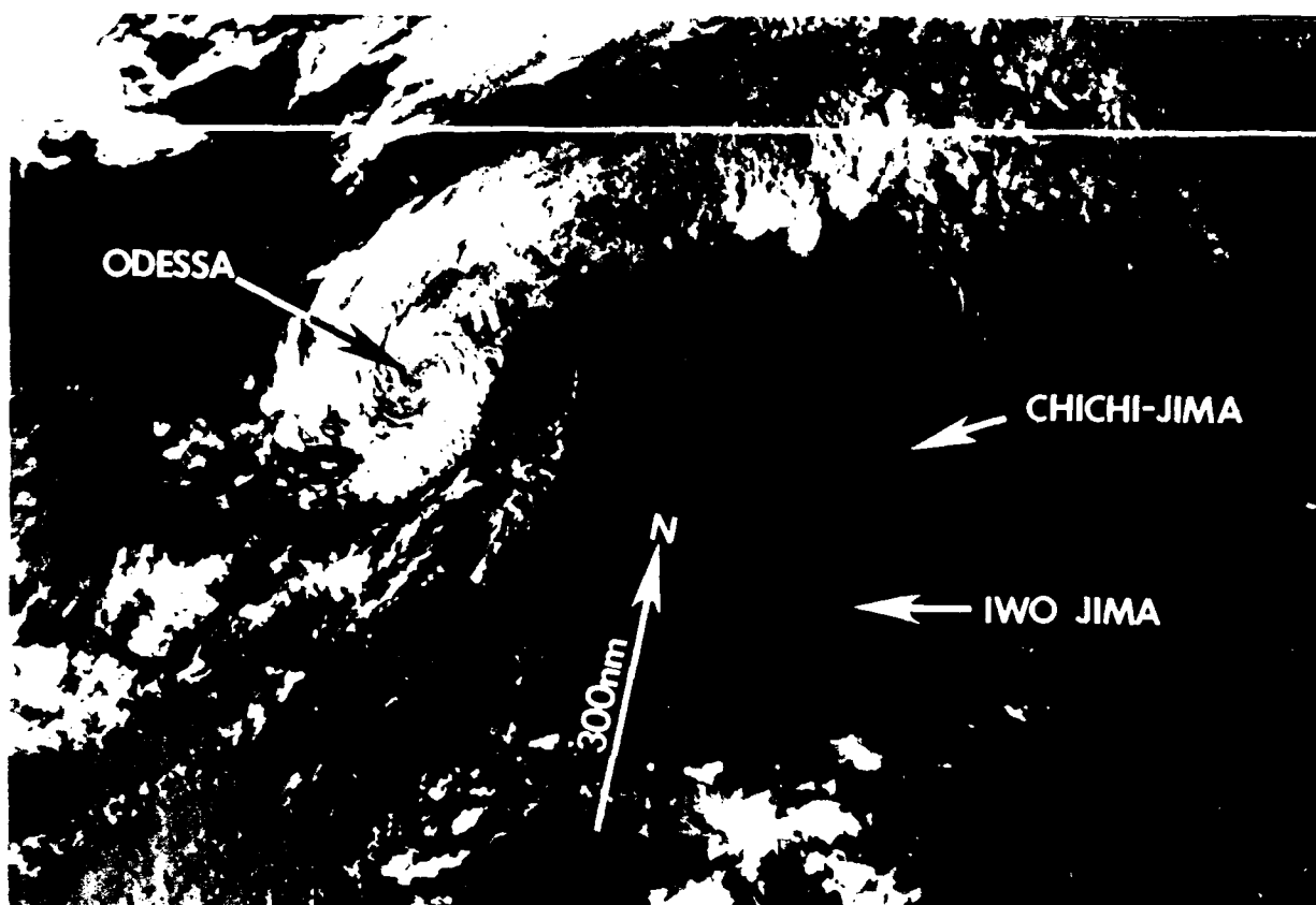
Figure 3-21-3. Odessa's well organized low-level circulation persists (170627Z October NOAA visual imagery).
