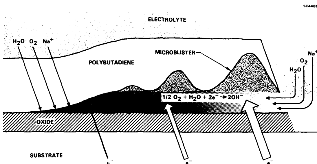
Fig. 6 Model for the polymer degradation process.
