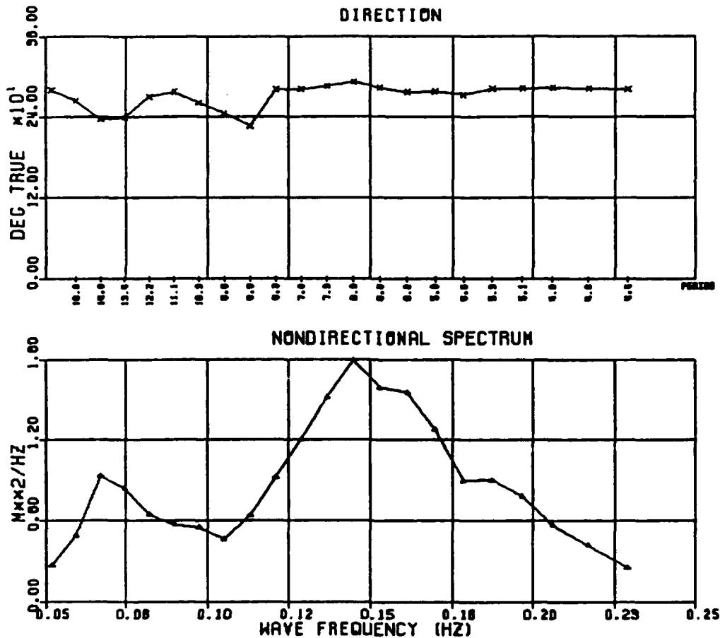
Figure 8. Typical information from CODAR (lower plot, nondirectional wave height spectrum; upper plot, mean wave direction)
