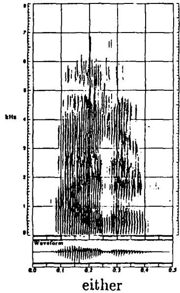
Figure 4.6: Spectra of / \delta / clusters.
