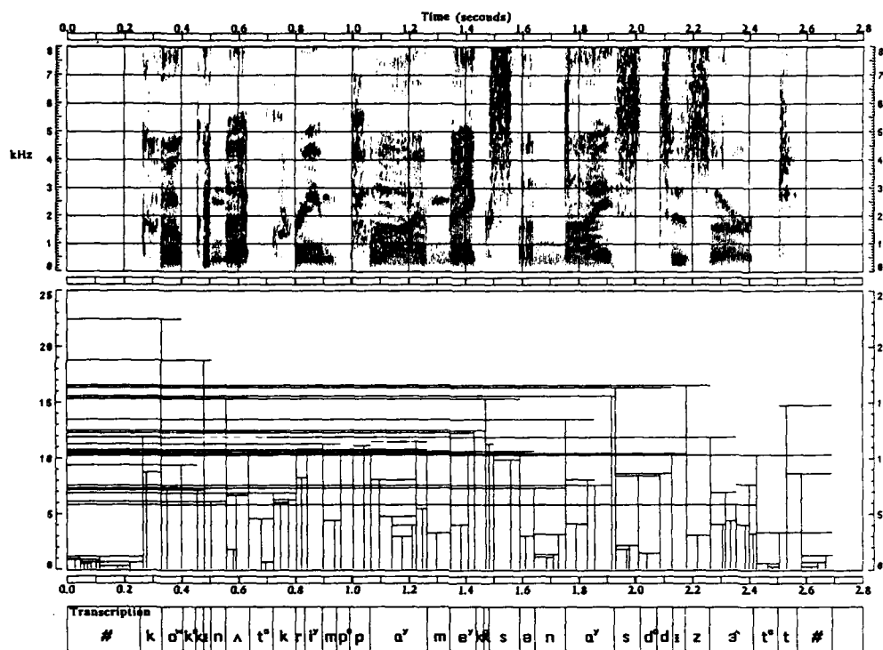
Figure 3.5: A non-monotonically increasing dendrogram.
