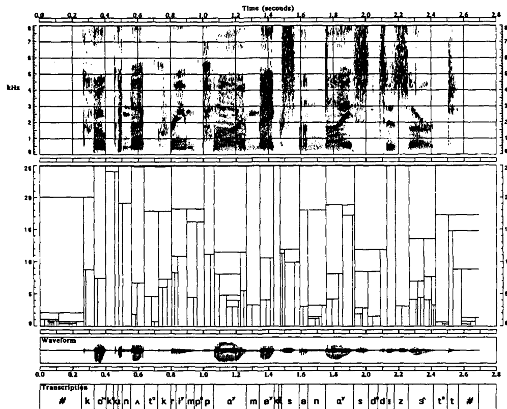
Figure 3.4: Multi-level description using a hierarchical structure.
