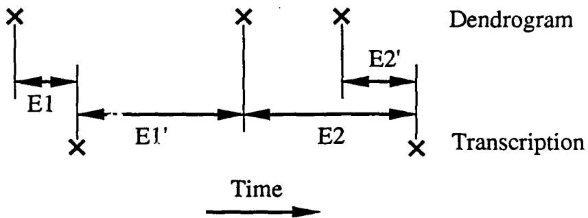
Figure 3.7: Dendrogram alignment procedure.
