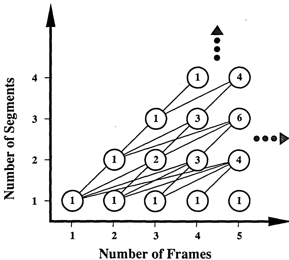
Figure B.1: Stochastic segmentation computation.
