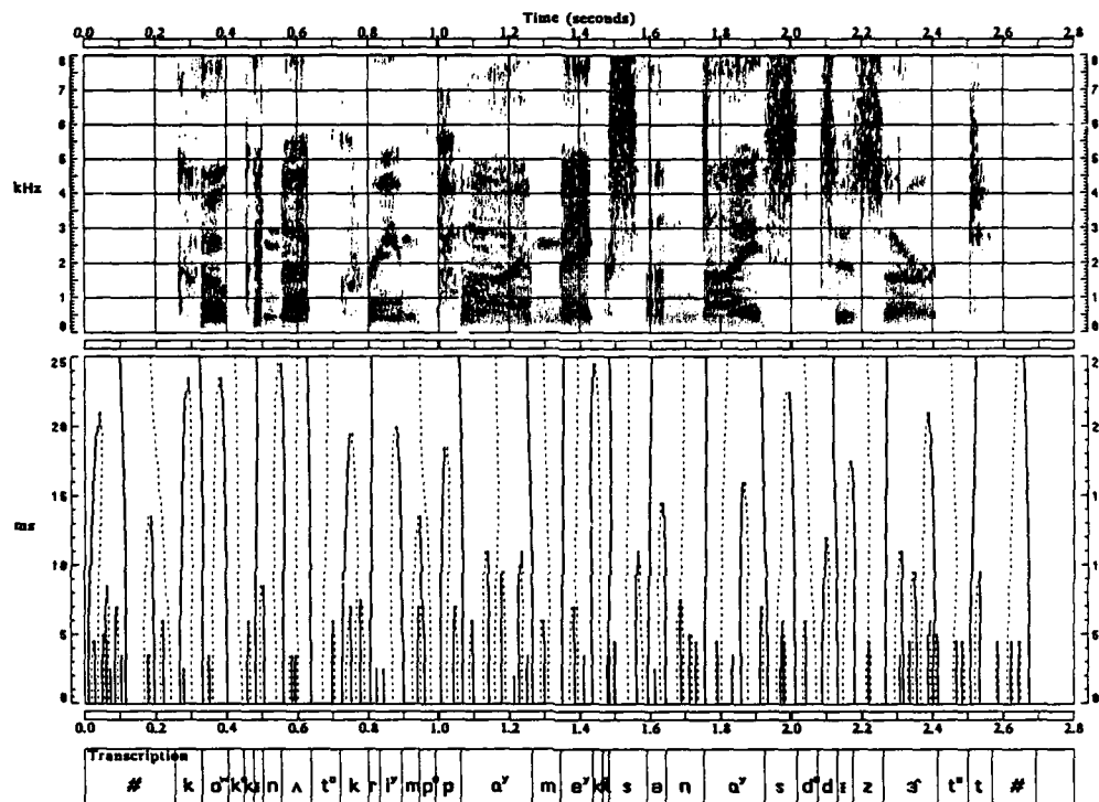
Figure 3.3: Multi-level description using scale-space filtering.
