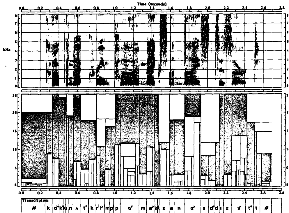
Figure 3.8: An aligned dendrogram.
