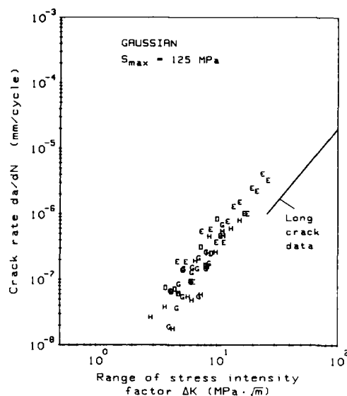
Figure 34.- GAUSSIAN results at S_{max} = 125 MPa after "non-interaction" analysis.
