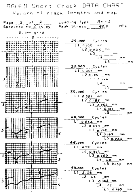
Figure 14.- Example of Data Chart for multi-cracks.
