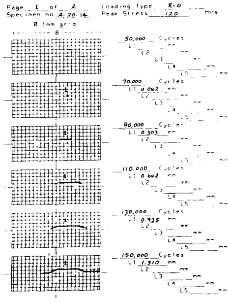
Figure 12.- Example of Data Chart for single crack.
