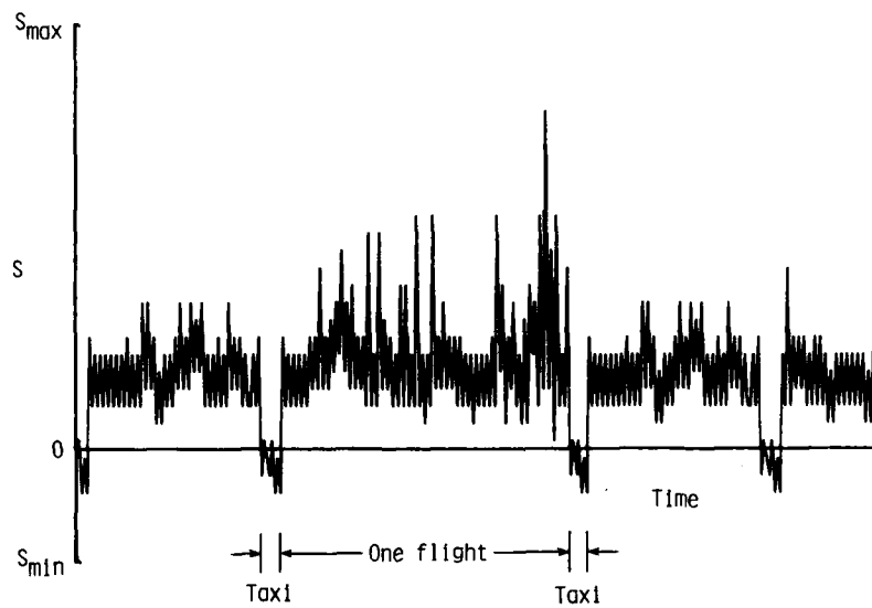
Figure 8(b).- Typical flights in FALSTAFF sequence.
