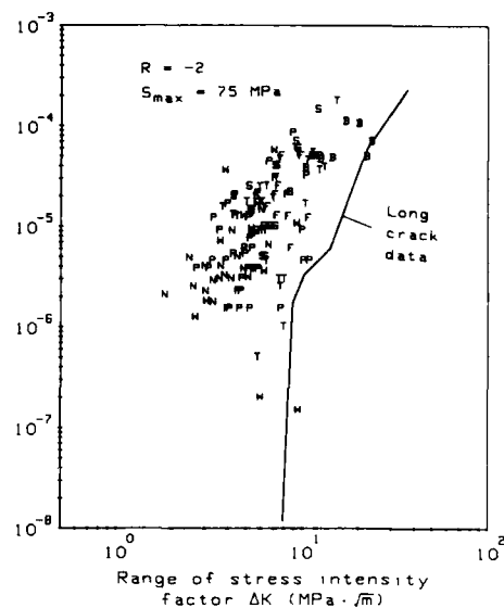
Figure 35.- Constant-amplitude ( R = -2 ) results at S_{max} = 75 MPa after "non-interaction" analysis.
