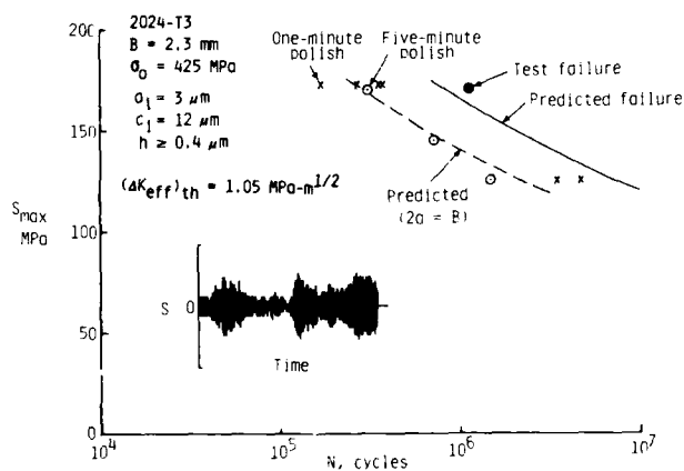
Figure B7.- Experimental and predicted fatigue life to breakthrough and failure under GAUSSIAN loading.
