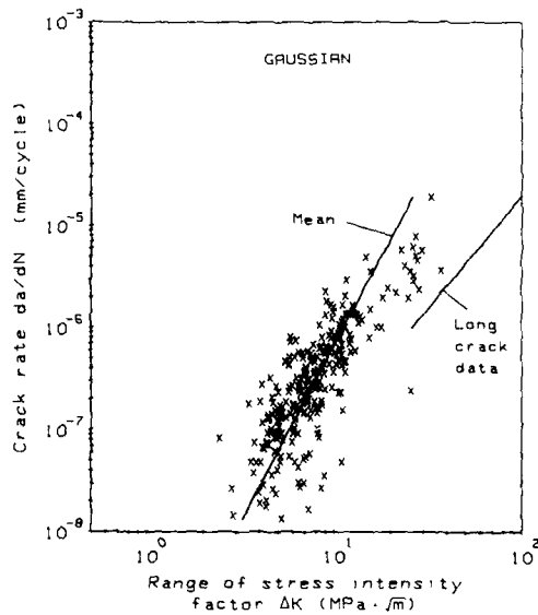
Figure 24.- All GAUSSIAN results after "non-interaction" analysis (4 laboratories).
