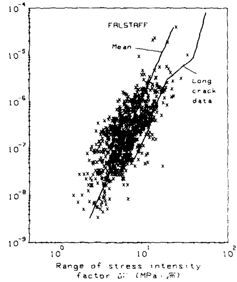
Figure 23.- All FALSTAFF results after application of "non-interaction" analysis (8 laboratories).
