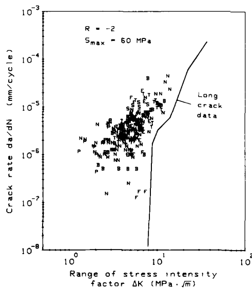
Figure 36.- Constant-amplitude ( R = -2 ) results at S_{max} = 60 MPa after "non-interaction" analysis.
