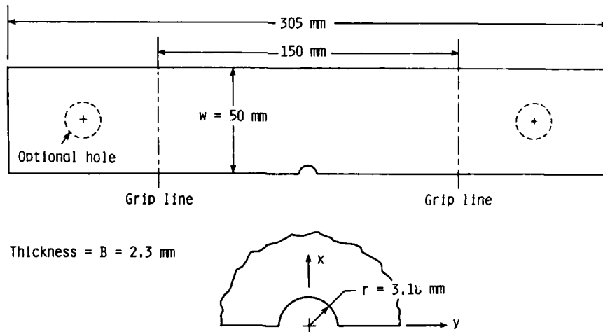
Figure 2.- Single-edge notched tension (SENT) fatigue specimen.
