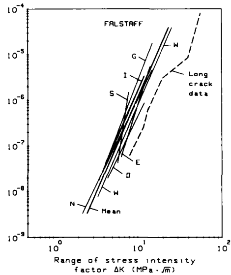
Figure 47.- Least-squares-fit straight lines for FALSTAFF short-crack data from different laboratories.
