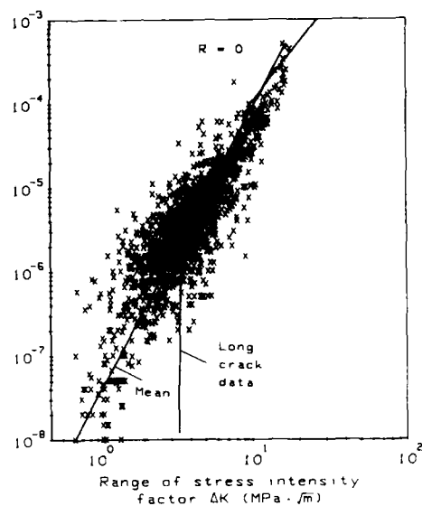
Figure 27.- All R = 0 results after "non-interaction" analysis (9 laboratories).
