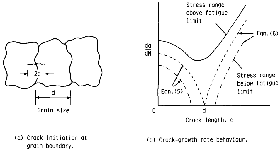
Figure 72.- Schematic of "micro-structural barrier" influence on crack-growth rates.
