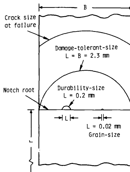
Figure 53.- Schematic of various surface cracks to define grain-size, durability-size, and damage-tolerant size defect.
