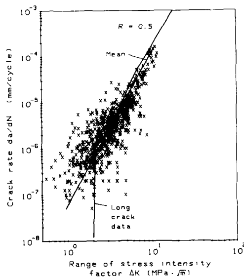
Figure 28.- All R = 0.5 results after "non-interaction" analysis (6 laboratories).
