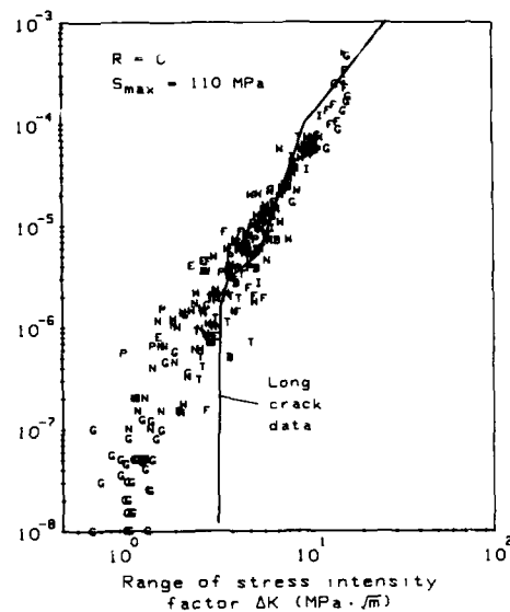
Figure 43.- Constant-amplitude ( R = 0 ) results at S_{max} = 110 MPa after "non-interaction" analysis.
