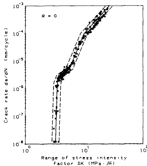
Figure G7.- Long-crack growth rate data from R = 0 tests.
