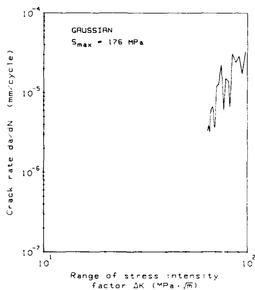
Figure H1.- Long-crack growth rate data from GAUSSIAN loading with S_{max} = 176 MPa.
