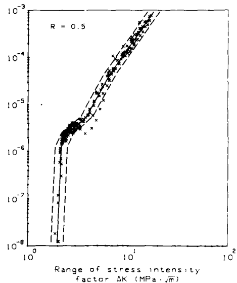
Figure G8.- Long-crack growth rate data from R = 0.5 tests.
