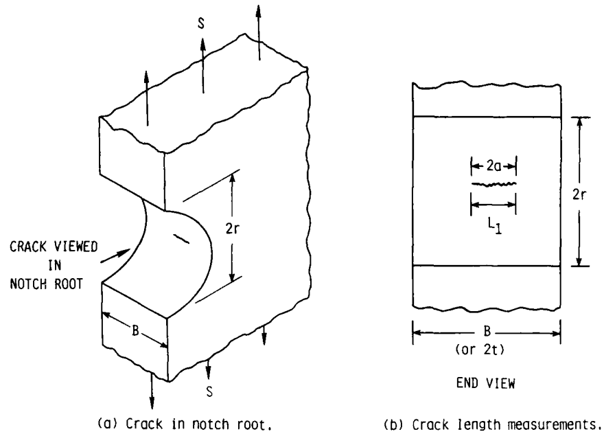
Figure 10.- Notch configuration and crack-length measurement in notch root.
