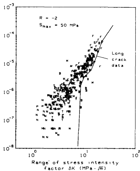
Figure 37.- Constant-amplitude ( R = -2 ) results at S_{max} = 50 MPa after "non-interaction" analysis.
