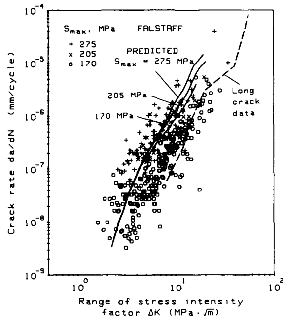
Figure 88.- Experimental and predicted crack-growth rates for short cracks under FALSTAFF loading.
