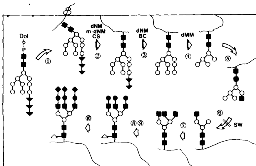
Fig. 1. Proposed sequence for the processing of peptide-bound N-linked glycans. Sites of inhibition by the following drugs are indicated by lines through arrows: dNM, 1-Deoxynorjirimycin; m-dNM, N -methyl-1-deoxynorjirimycin; CS, castanospermine; BC, bromocunduritol; dMM, 1-deoxymannojirimycin; SW, swainsonine. The reactions are catalyzed by the following enzymes: (1) oligosaccharyltransferase, (2) RER \alpha -glucosidase I, (3) RER \alpha -glucosidase II, (4) RER \alpha -1,2-mannosidase, Golgi \alpha -mannosidases IA and IB, (5) Golgi N -acetylglucosaminyltransferase I, (6) Golgi \alpha -mannosidase II, (7) N -acetylglucosaminyltransferases II and IV, (8) fucosyltransferase, (9) galactosyltransferase, (10) sialyltransferase. Symbols: ■, N -acetylglucosamine; ○, mannose; ▲, glucose; ▽, fucose; ●, galactose; ▲, sialic acid. Adapted from Kornfeld et al. (1978).
