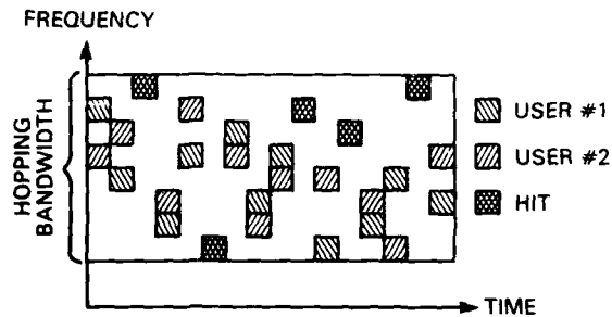
Fig. 4 — Simplified illustration of frequency-hopping CDMA
