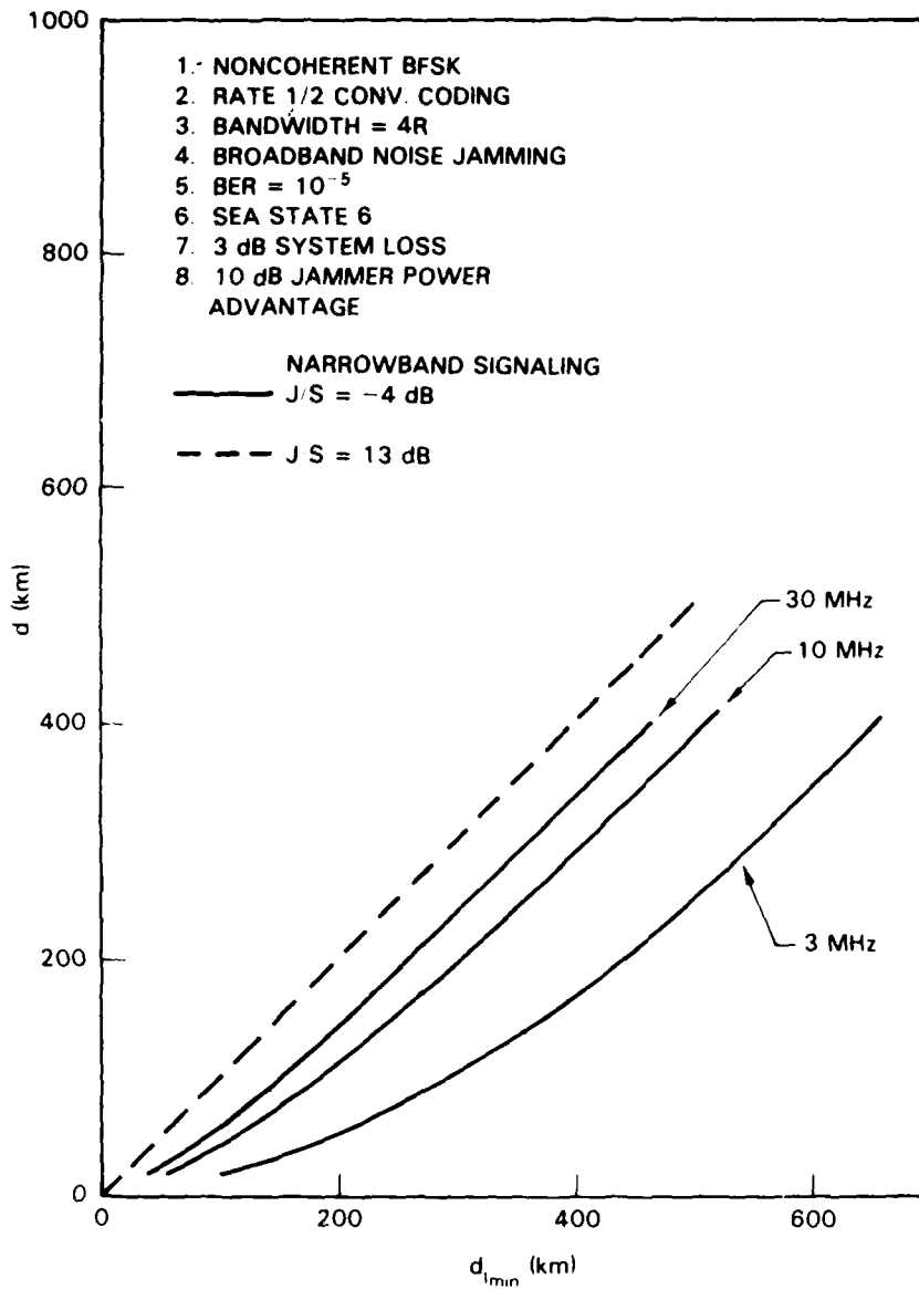
Fig. 7 — d_{min}(d) vs d for HF groundwave model and narrowband signaling
