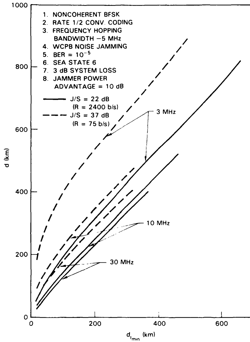
Fig. 6 — d_{min}(d) vs d for HF groundwave model and wideband signaling
