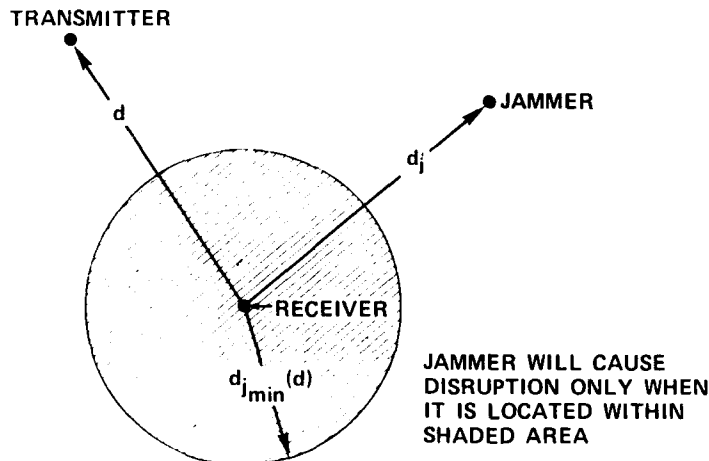
Fig. 5 — Transmitter-receiver-jammer geometry
