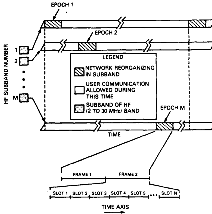
Fig. 3 — Timing for network restructuring
