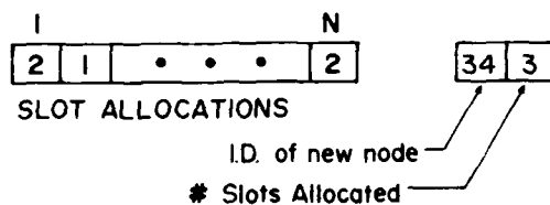
Fig. 10 - Modifications of TSA to allow for new nodes
