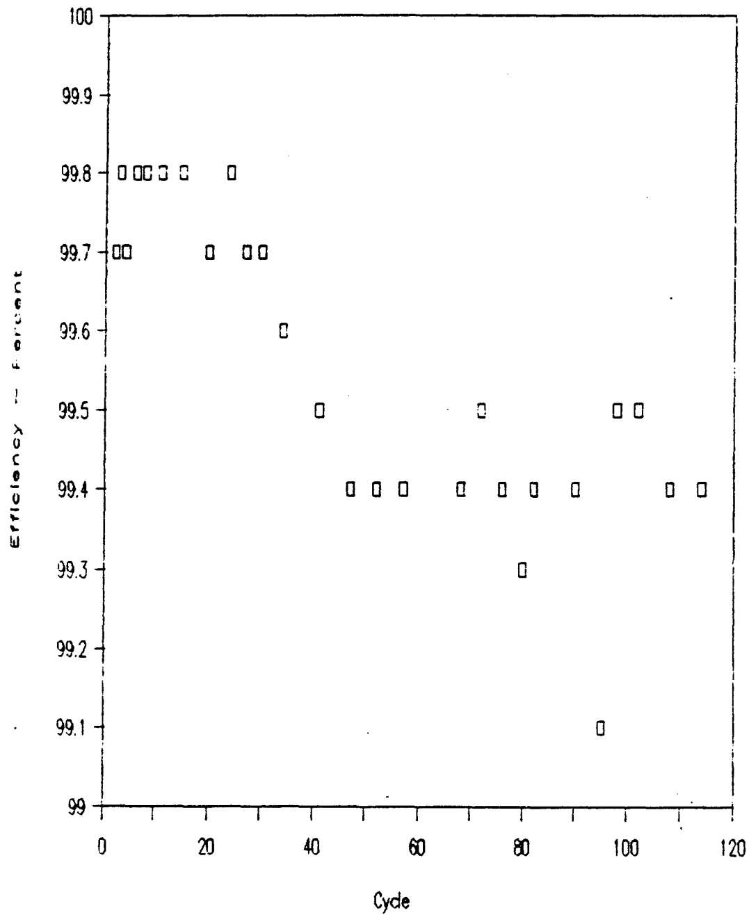
Figure 5-30. Filtration Efficiency
