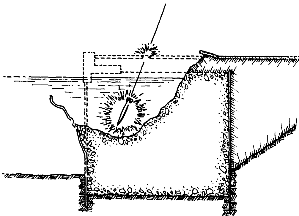
b. Closed construction, cratering of rubble- or sand-filled steel cofferdams or sheet piling walls
