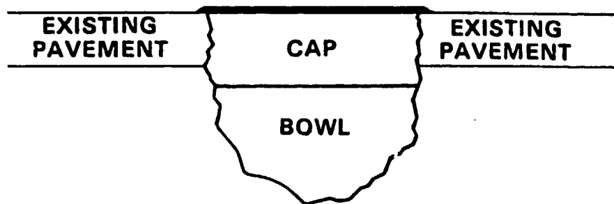
Figure 76. Crater bowl and cap
