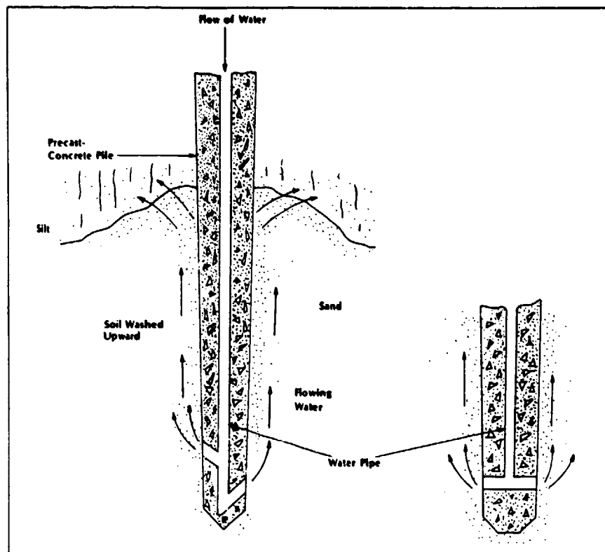
Figure 43. Precast concrete piles with internal jetting pipes
