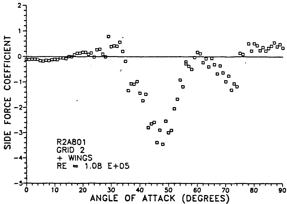
Figure 27. R2A801: Side Force Coefficient.
