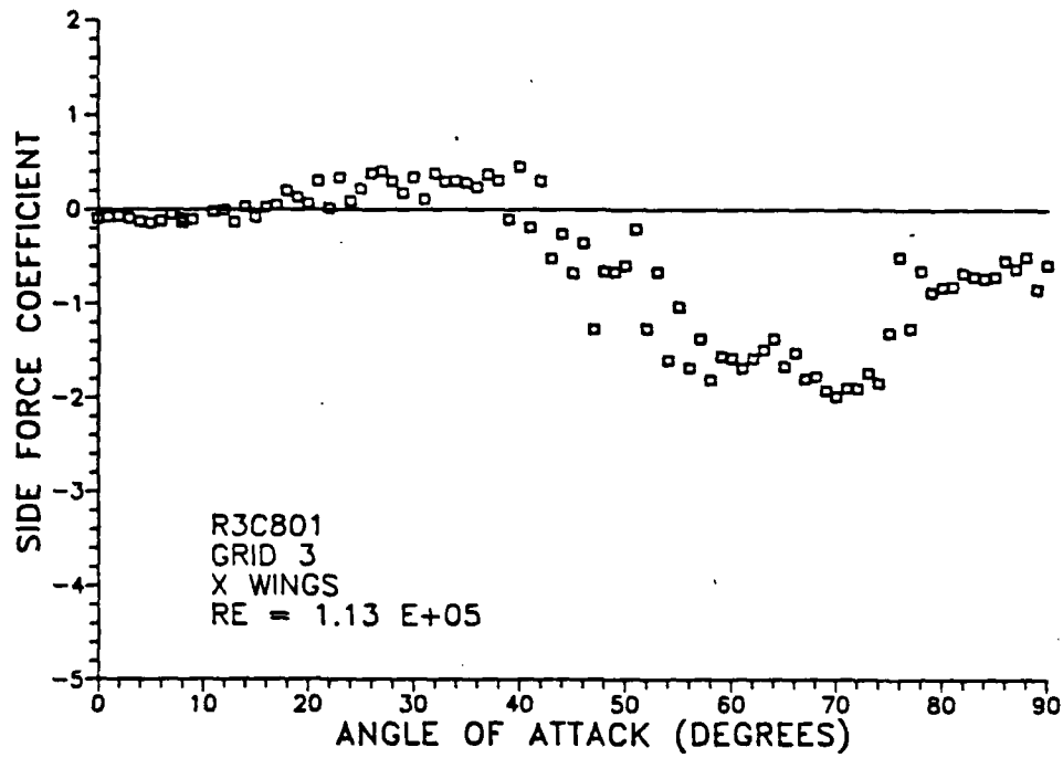
Figure 32. R3C801: Side Force Coefficient.
