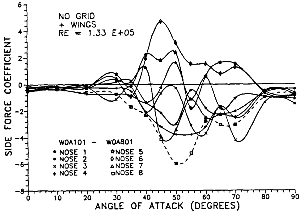
Figure 16. Side force variations with nose roll angle: Runs WOA101 to WOA801.
