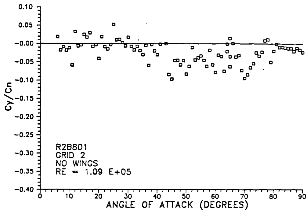
Figure 51. R2B801: Side Force to Normal Force Ratio.
