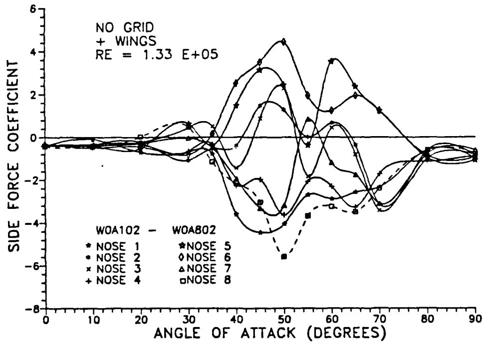
Figure 17. Side force variations with nose roll angle: Runs WOA102 to WOA802.
