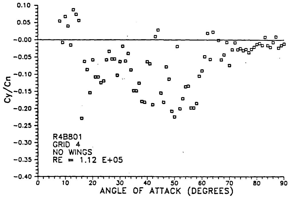
Figure 53. R4B801: Side Force to Normal Force Ratio.
