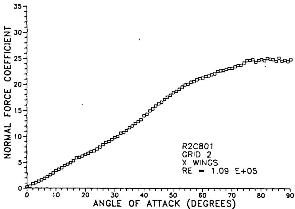
Figure 46. R2C801: Normal Force Coefficient.
