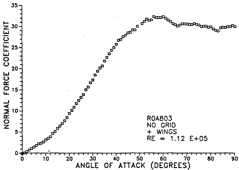
Figure 39. ROA803: Normal Force Coefficient.
