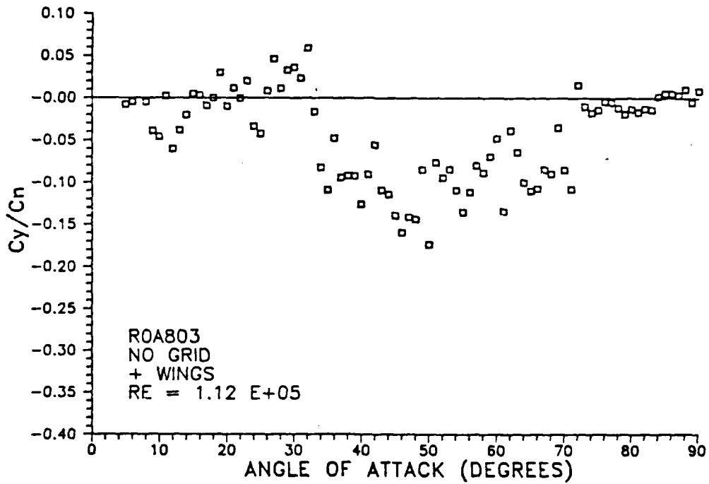
Figure 54. R0A803: Side Force to Normal Force Ratio.
