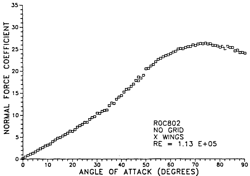
Figure 40. ROC802: Normal Force Coefficient.
