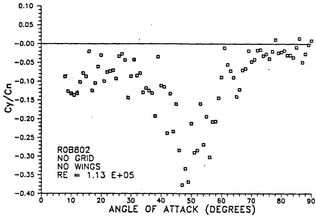
Figure 49. ROB802: Side Force to Normal Force Ratio.
