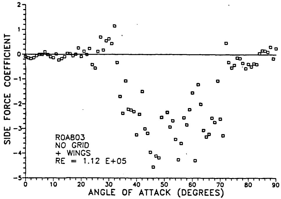
Figure 24. ROA803: Side Force Coefficient.
