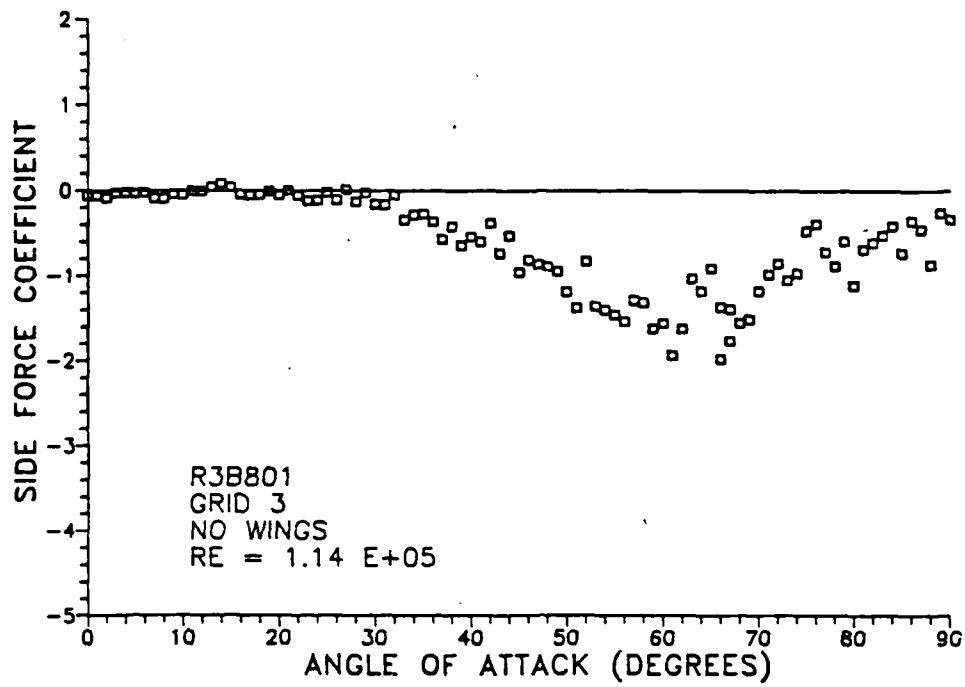
Figure 22. R3B801: Side Force Coefficient.
