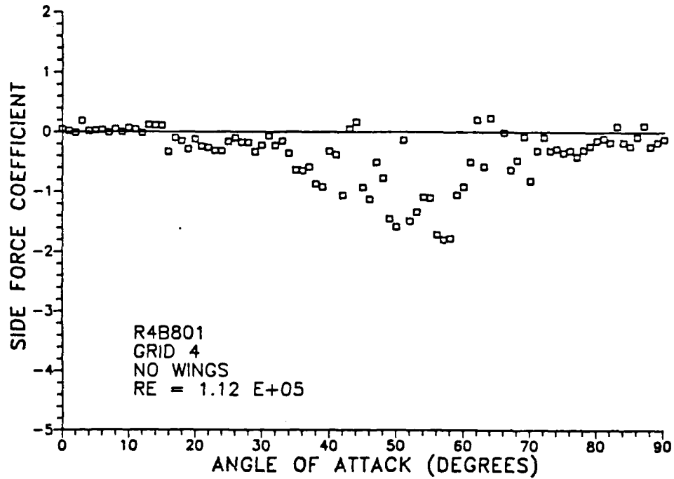
Figure 23. R4B801: Side Force Coefficient.
