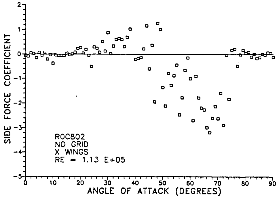
Figure 25. ROC802: Side Force Coefficient.
