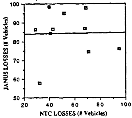
REGRESSION OF TOTAL RED FORCE LOSSES
