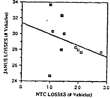
REGRESSION OF TOTAL RED FORCE TANK LOSSES y = 31.3664 - 0.143x R = 0.32
