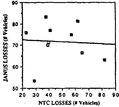
REGRESSION OF TOTAL RED TANK & BMP LOSSES y = 73.2843 - 0.0324x R = 0.07
