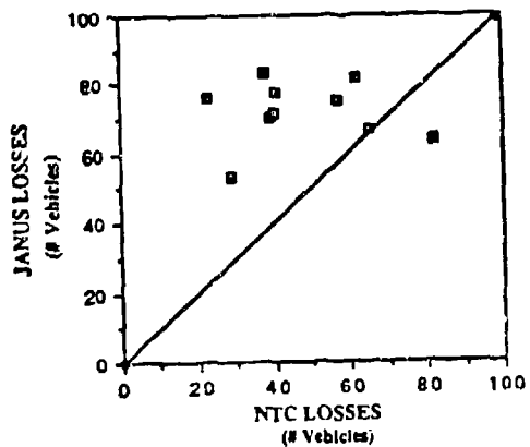
TOTAL RED FORCE TANK & BMP LOSSES
