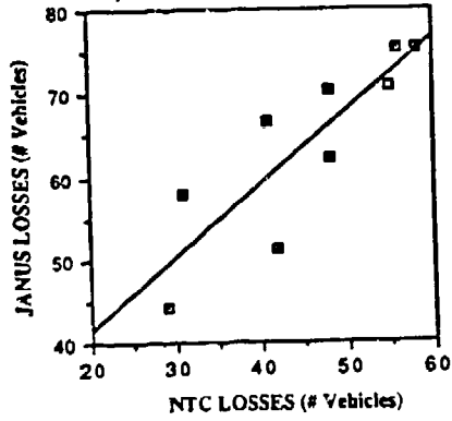
REVISED REGRESSION OF TOTAL BLUE FORCE LOSSES
