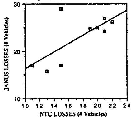
REVISED REGRESSION OF TOTAL BLUE TANK LOSSES
