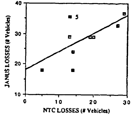
REGRESSION OF TOTAL BLUE FORCE APC LOSSES y = 18.0803 + 0.6006x R = 0.67
