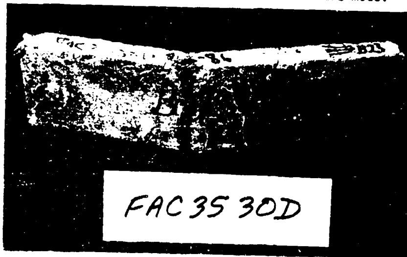
Figure 14. Typical variable depth beam (1 in) failure mode.
