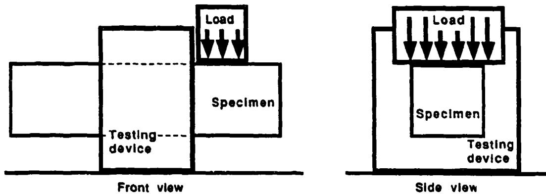
Alternate Shear Test 1
