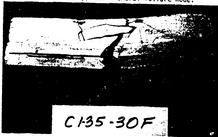
Figure 13. Typical composite beam failure mode.
