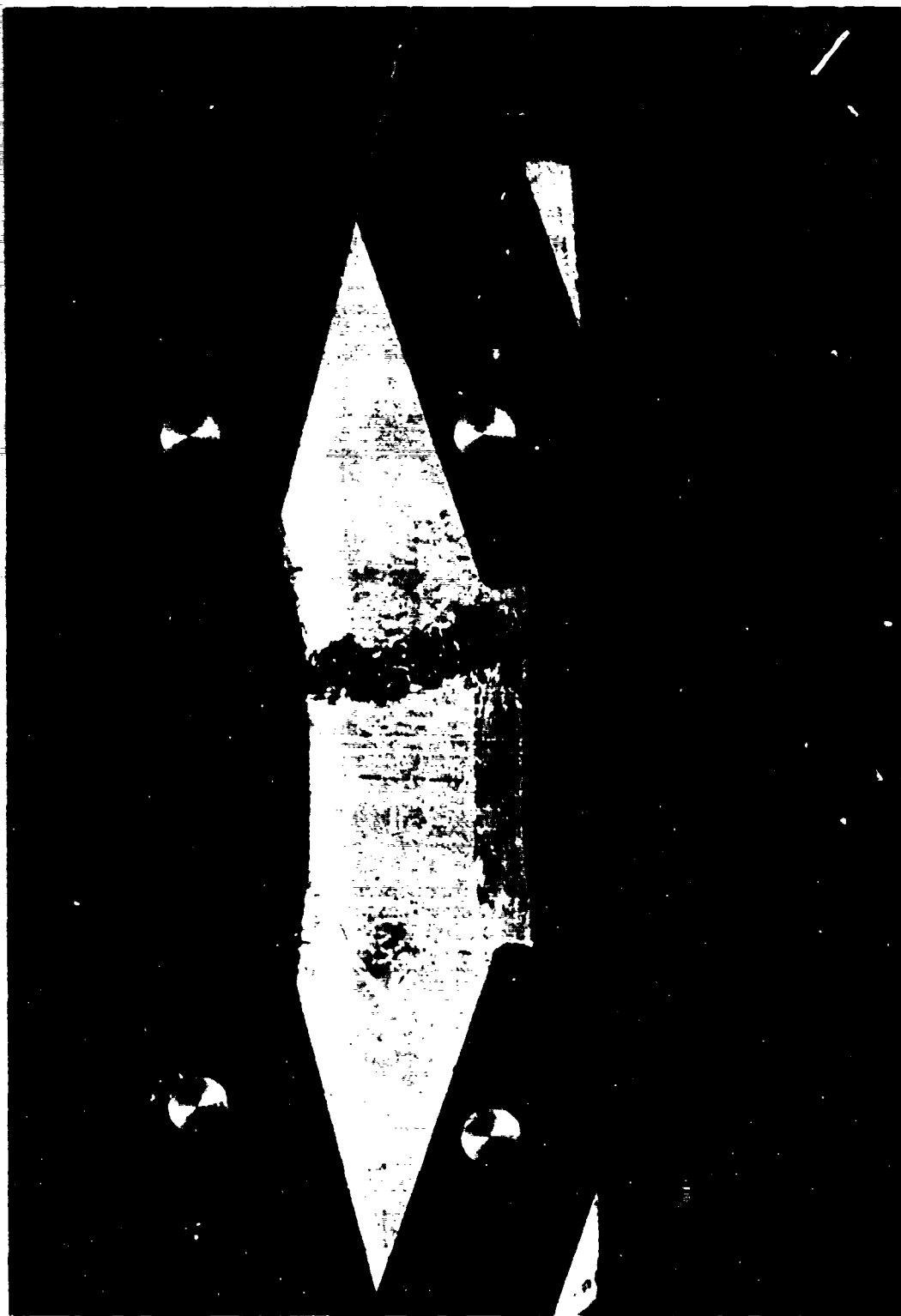
Figure 16. Typical tension failure mode--milled specimen.
