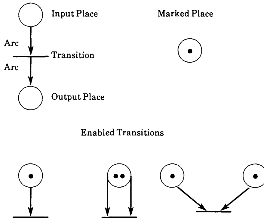
Figure 2.1 Standard Petri Net Symbology
