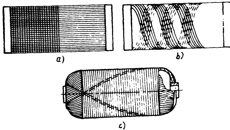
Fig. 23.8. Varieties of methods of coil/winding: a) longitudinal-transverse; b) spiral (oblique); c) transverse spiral.
