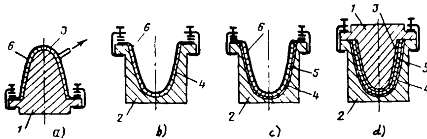
Fig. 23.9. Schematic of basic stages of manufacture of fairing with basing on external contour/outline: a, b, c, d) sequence of stages (1 - male die/punch, 2 - matrix/die, 3 - lower covering, 4 - outer skin, 5 - honeycomb filler, 6 - rubber cover).
