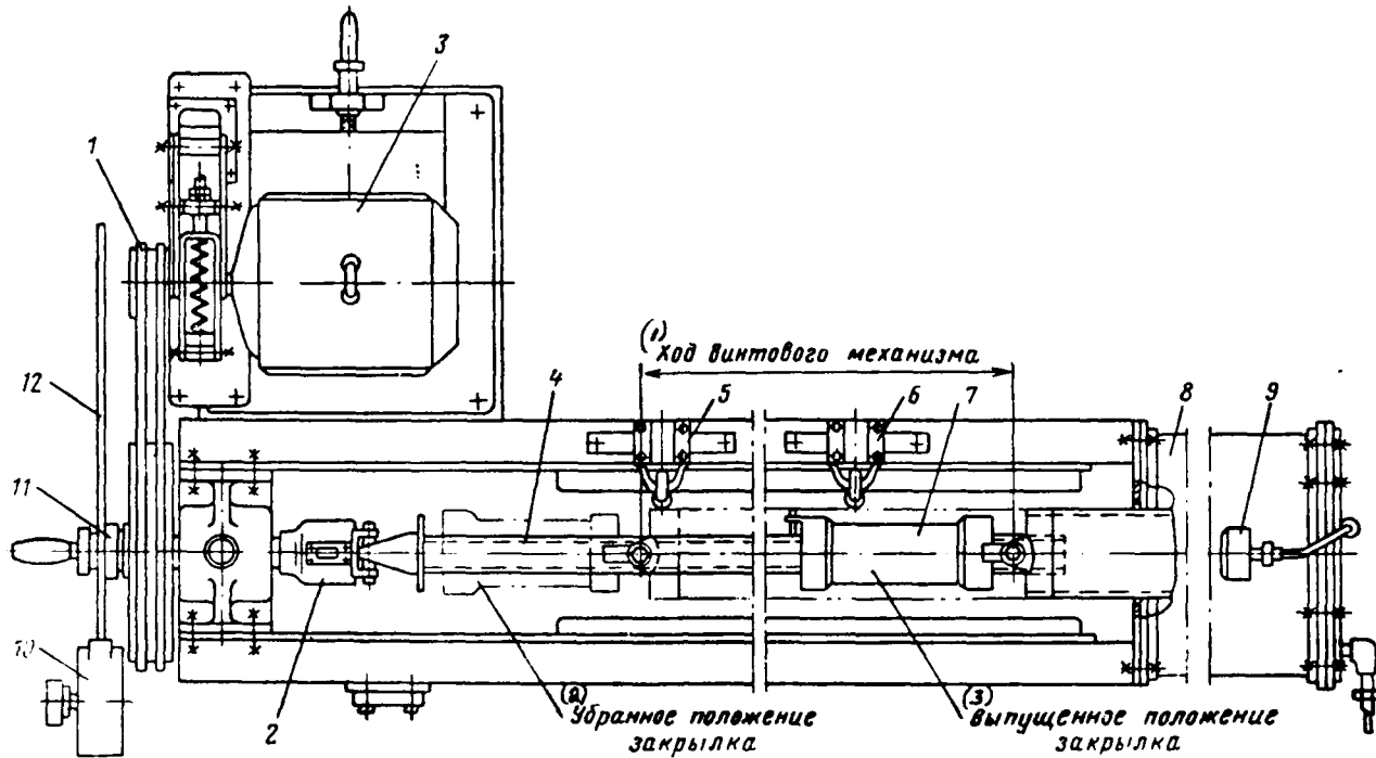
Fig. 24.11. Run-in table and testing screw mechanism of flap control: 1 - belt drive; 2 - universal joint; 3 - electric motor; 4 - screw; 5 and 6 - limit switches; 7 - screw mechanism; 8 -pneumatic cylinder; 9 - manometer; 10 - loads; 11 - drive shaft; 12 - rack. Key: (1). Course of screw mechanism. (2). Flaps up position. (3). Flaps down.
