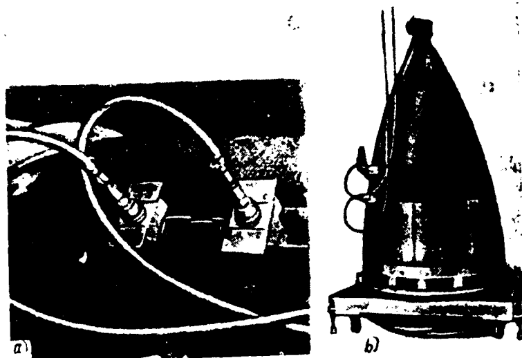
Fig. 23.11. To treatment of light filler of radome: a) pneumatic milling heads; b) general view of milling fixture.
