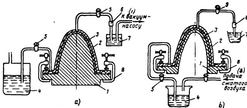
Fig. 23.6. Diagram of impregnation under pressure: a) vacuum (mold, rigid); b) under excess positive pressure [1 - male die/punch, 2 - matrix/die, 3 - filler (fiberglass fabric, fiberglass fabric), 4 - small tank with resin, 5 - stop cock, 6 - inspection window; 7 - small tank for resin, 8 - screw clamp].
