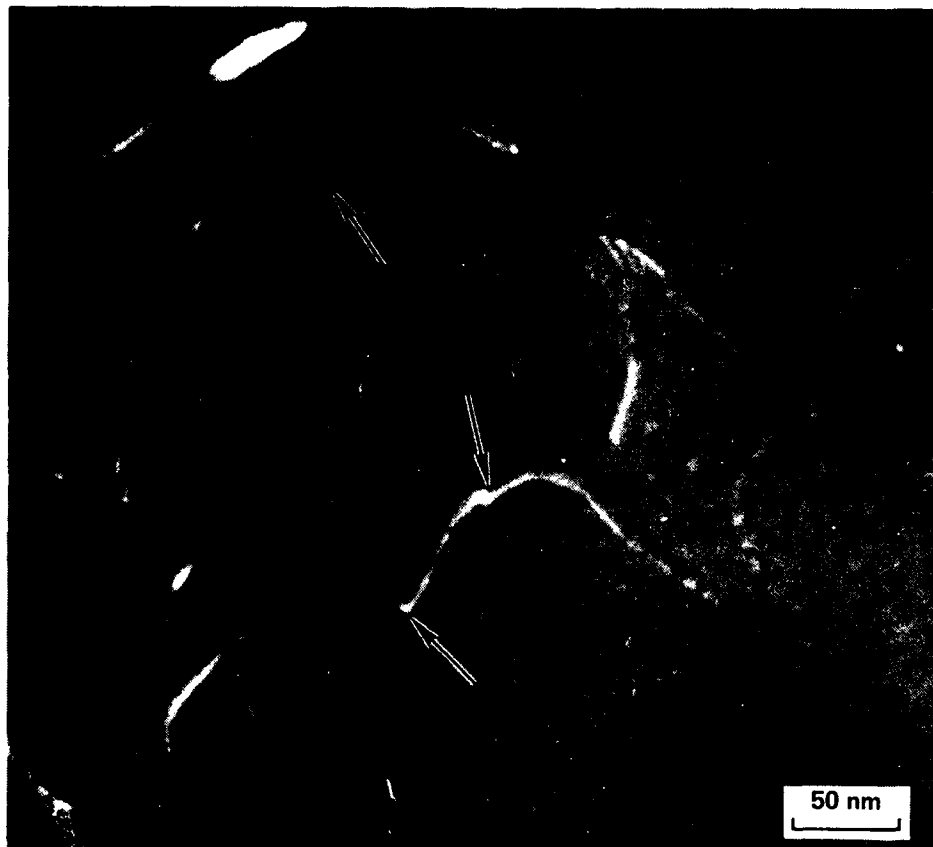
Fig. 19 TEM of creep-tested Alloy 19 illustrating pinned dislocation.
