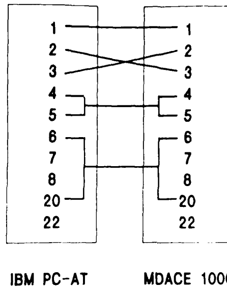
Figure 2 Wiring diagram for the RS-232 asynchronous communication cable used to interface the computer to the stage controller.
