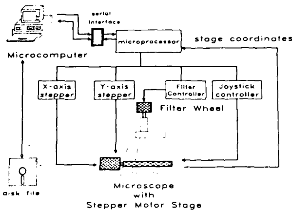
Figure 1 Main components of the MDACE 1000 stage controller. Instruction codes from the computer are sent to the stage controller microprocessor using a serial RS-232 interface.
