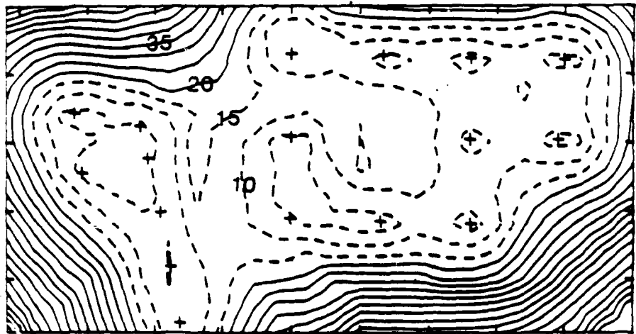
Figure 4.1 The error fields (% standard deviation) on 19 January 1985 for two decimation times: case A (top; \sigma_t = 2 d), with dashed contours indicating <15% error; and case B (bottom; \sigma_t = 1 d), with dashed contours indicating <20% error. Contour intervals are 5%.
