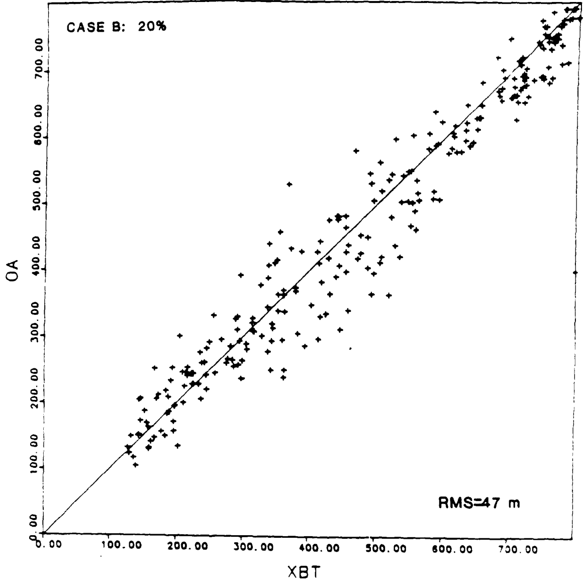
Figure 4.11 Same as in Figure 4.5 except for case B ( \delta t = 1 d) and <20% error.
