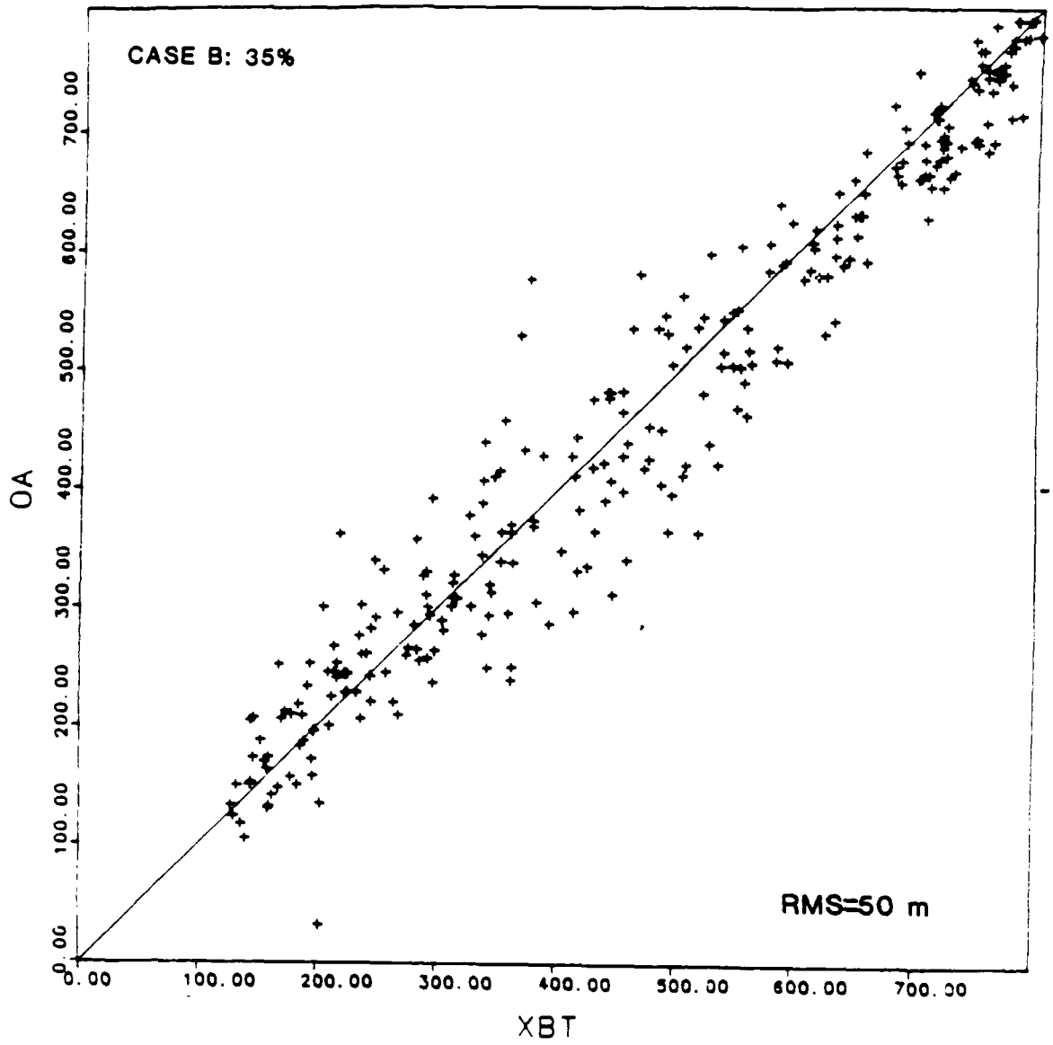
Figure 4.12 Same as Figure 4.6 except for case B.
