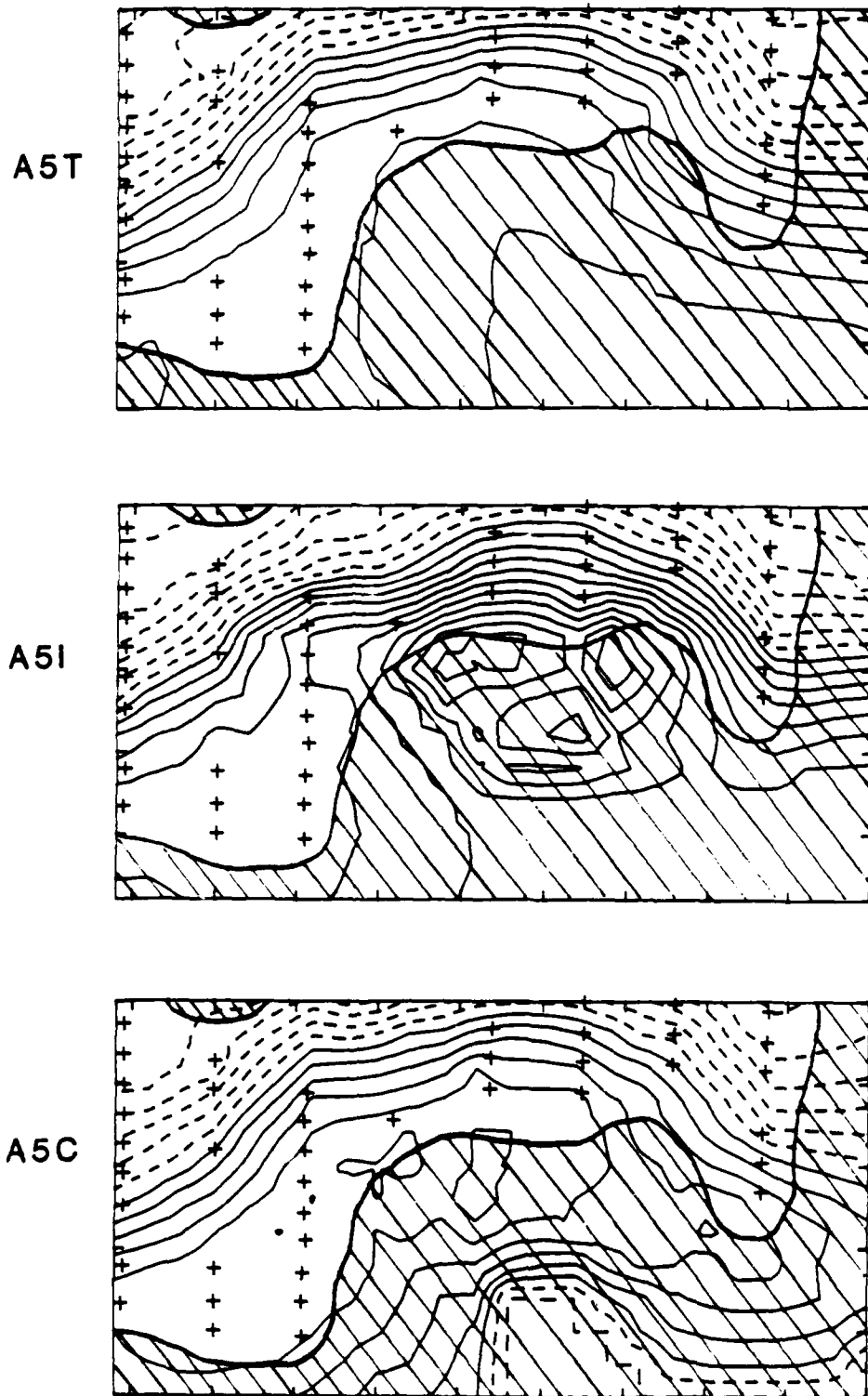
Figure 3.4 AXBT OA maps as in Figure 3.2 except for survey 5 (17 October 1984).
