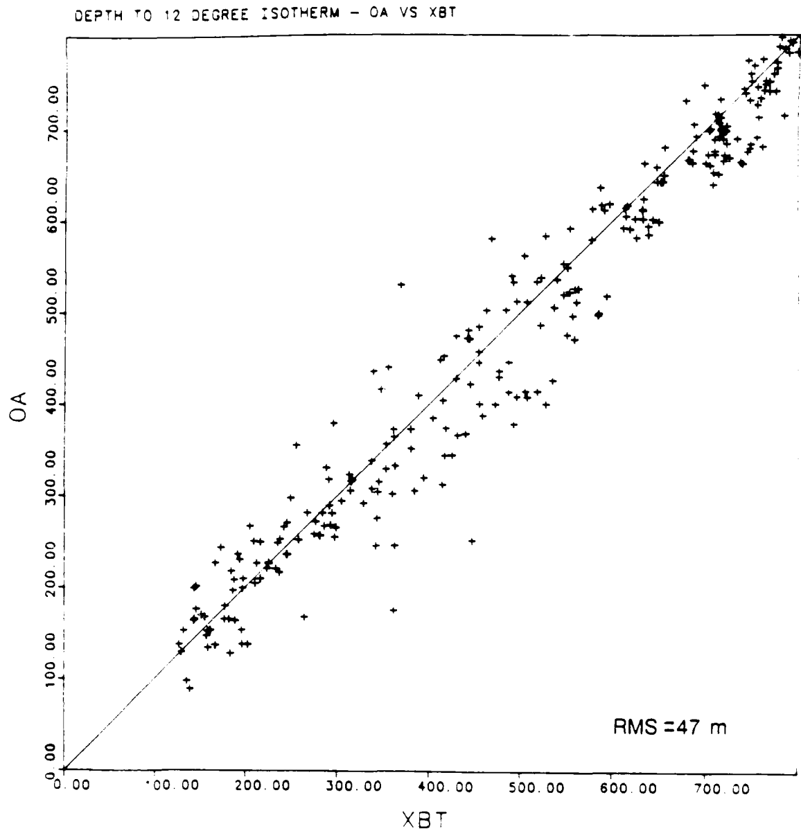
Figure 4.5 Comparison of the Z_{12} from XBTs versus the Z_{12} from 1ES OA maps within the region where mapping error is < 15\% for case A ( \delta t = 2 d). The solid line represents the line of perfect agreement.
