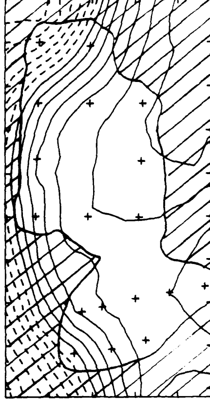
Figure 3.15 IES OA maps as in Figure 3.14 except for survey 5 (17 October 1984).
