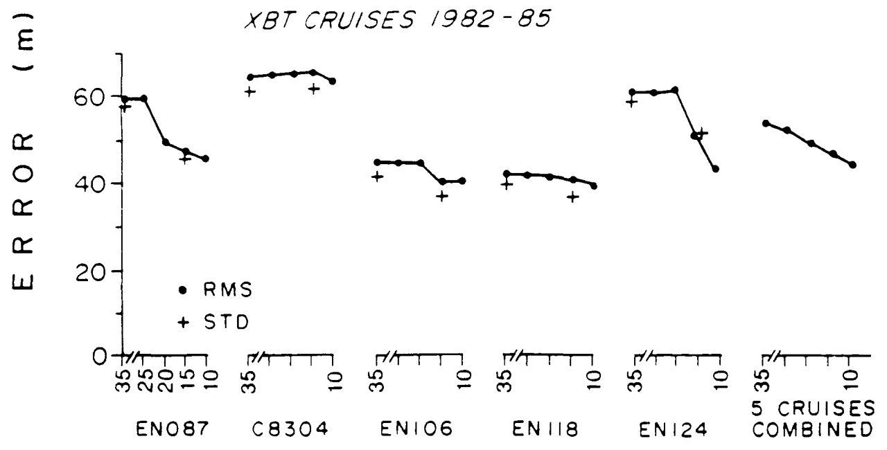
Figure 4.7 The RMS difference (•) and STD difference (+) for Z_{1z} values from IES OA maps compared with Z_{1z} values from XBT's within five levels of estimated error for case A ( \delta t = 2 d) for five cruises individually and for all five cruises combined.
