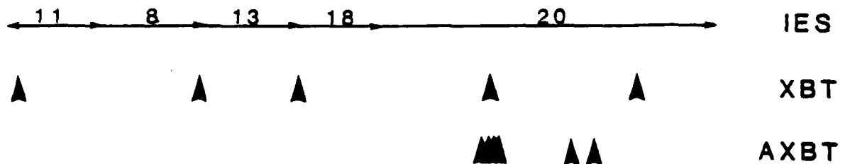
Figure 2.1 Map of IES array (top) and timeline of XBT and AXBT surveys (bottom). IES locations are shown by the solid circles and squares; the box outlines the 240 km by 460 km region mapped by objective analysis. The number of IESs deployed in the study area between July 1982 and May 1985 are indicated on the timeline. The dates of the XBT shipboard surveys and AXBT flight surveys are indicated by the arrows below the timeline.
