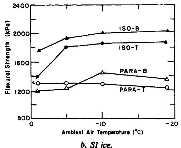
Figure 25. Comparative relationships of flexural strengths of isothermal and parallel simply supported beams, demonstrating temperature gradient effects. Extrapolations of data to 0°C are indicated by dashed lines.
