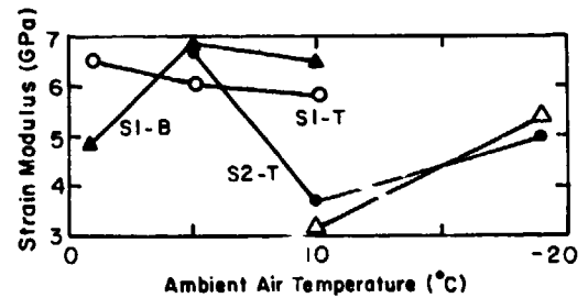
Figure 22. Strain modulus versus temperature of simply supported beams tested in conjunction with cantilever beams. Symbols T and B refer to top and bottom in tension tests respectively.
