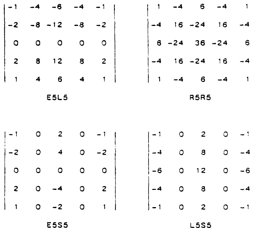
Fig. 5. 5 by 5 center-weighted mask filters.
