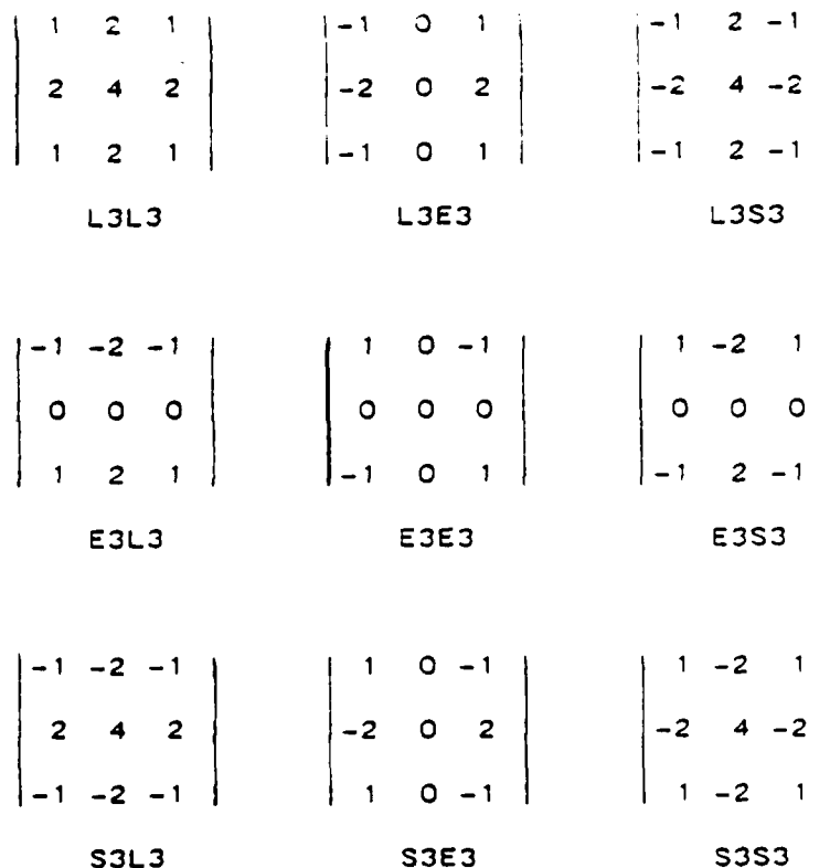
Fig. 4. 3 by 3 center-weighted mask filters.
