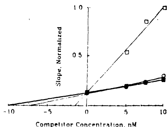
Figure 9. The inhibition of [ ^3\text{H} ]PbTx-3 binding by four brevetoxins: K i determinations. Inhibition constants for each of brevetoxins -1 (□), -2 (■), -3 (●), and -7 (○) were determined by utilizing tritium-labeled PbTx-3 concentrations of 5.0, 7.5, 10.0, and 15.0 nM, and competitor brevetoxin concentrations ranging from 0, 5.0, 7.5, and 10 nM at each labeled toxin concentration. The slopes of the appropriate lines in Figure 8 were determined, and each slope was normalized to the slope of PbTx-1 inhibition at 10.0 nM.
