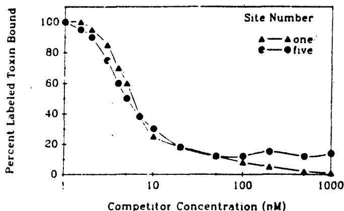
Figure 5. Comparison of specific displacement of 10 nM tritiated saxitoxin (triangles) or 10 nM tritiated PbTx-3 by unlabeled competitor saxitoxin or brevetoxin, respectively in rat brain synaptosomes. ED_{50} in each case is 5-10 nM.
