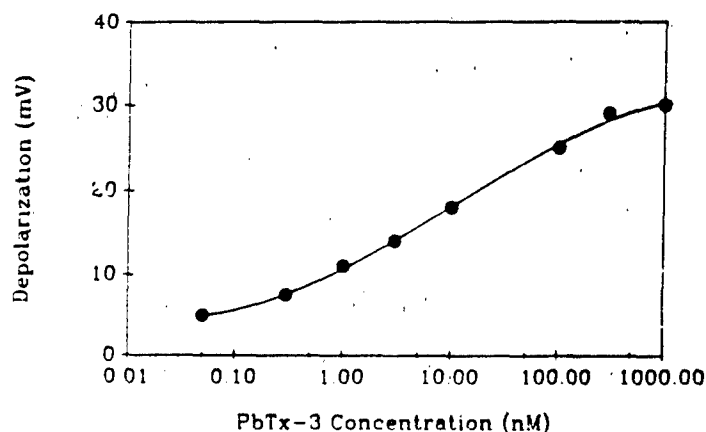
Figure 2. Dose-response curve of membrane depolarization as a function of PbTx-3 concentration. Data from a total of 22 axons were pooled; each axon received only one dose. Data are plotted as means of depolarization amplitudes. The solid line is a theoretical 3rd order fit with an \text{IC}_{50} of 1.5 nM, maximum observed depolarization of 30 mV and a Hill's coefficient of 2 (7).
