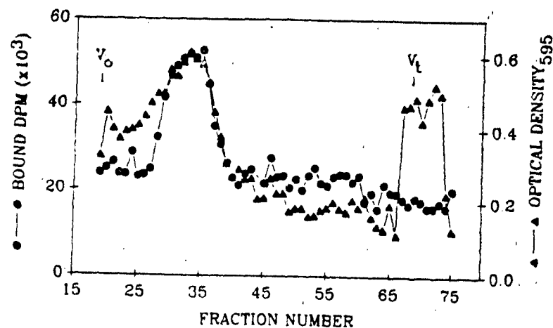
Figure 12. Demonstration of specific tritiated brevetoxin binding in Sephacryl A-300 fractions of solubilized rat brain synaptosomes. Membrane proteins were solubilized using detergents in the presence of protease inhibitors. Solubilized proteins were chromatographed on a Sephacryl A-300 size partition column. Eluted fractions were assayed for both specific brevetoxin binding (circles) and protein (triangles).
