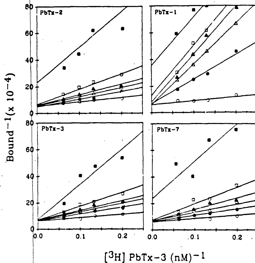
Figure 8. Inhibition of [^3\text{H}] PbTx-3 specific binding by unlabeled brevetoxins. Specific binding of tritiated brevetoxin PbTx-3 was measured to intact rat brain synaptosomes at 4°C in standard binding medium at four different concentrations of labeled toxins-- 5.0, 7.5, 10.0, and 15.0 nM-- in the presence of unlabeled brevetoxins at 0 (○), 5.0 (●), 7.5 (△), 10.0 (▲), 25.0 (□), 50.0 (■), or 100.0 (data not shown) nM. Each concentration point was determined in triplicate. The results are representative of three separate experiments. All competition experiments were performed on a single pooled brain synaptosome preparation, three separate preparations utilized to obtain the three experimental replicates.
