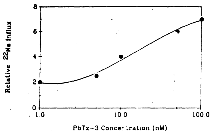
Figure 3. Concentration dependence of the stimulation of ^{22}\text{Na}^+ influx by PbTx-3. Synaptosomes were pre-incubated for 30 min with indicated concentrations of PbTx-3 in the presence of aconitine. Influx is plotted as specific influx, points representing means of triplicate determinations (4).
