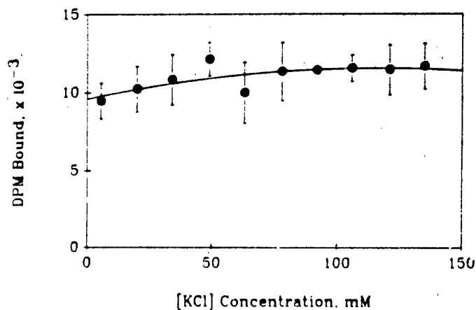
Figure 11. Voltage dependence of binding of [ 3 H]PbTx-3 to synaptosomes was measured at 4°C at the indicated concentrations of potassium ion, as described in experimental. KCl was exchanged for choline chloride to maintain iso-osmolarity. The membrane potential varies from -55 mV in standard binding medium to 0 mV at 135 mM KCl. The figure represents a composite of four experiments, triplicate determination in each. Error bars represent 95% confidence limits.
