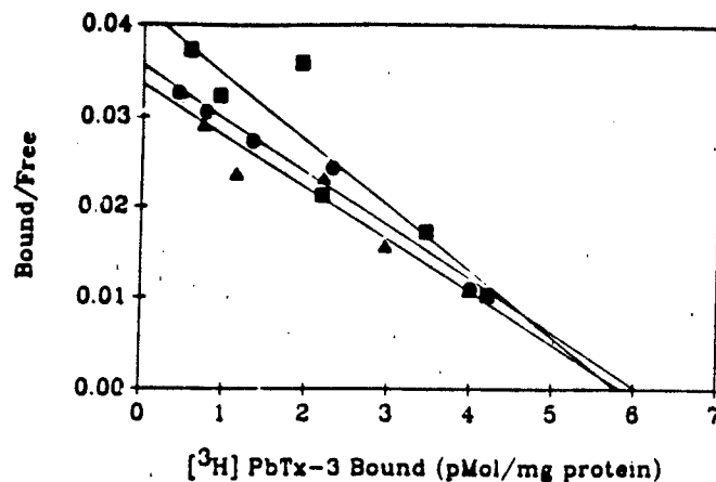
Figure 10. Rosenthal analysis of specific [ 3 H] PbTx-3 binding to intact (●), lysed (▲), and depolarized (■) synaptosomes. Binding was measured at 4°C in rat brain synaptosomes or lysed synaptosomes according to protocols explained in the text. These results are representative of four separate experiments, each done in triplicate.
