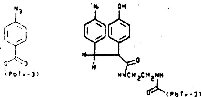
Figure 6. Photoaffinity Probes Constructed Using Brevetoxin PbTx-3. PbTx-3- p -azidobenzoyl ester (left) and PbTx-3- p -azidophenyl propionyl ethylene diamine monoamide (right).
