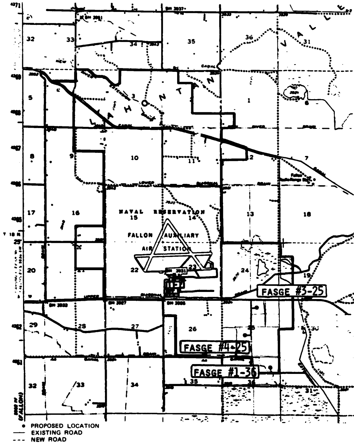
FIGURE 12. Proposed Locations for Mainside Geothermal Exploration Wells. Modified from Helioscience General Joint Venture (1985). FASGE #1-36 is location for FOH-2.
