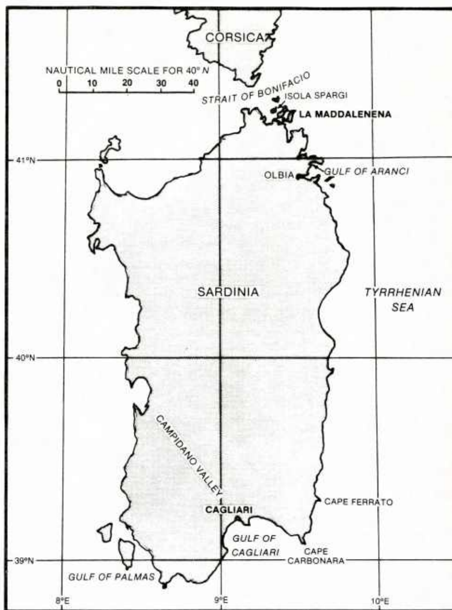
Figure 3-2. Gulf of Cagliari
