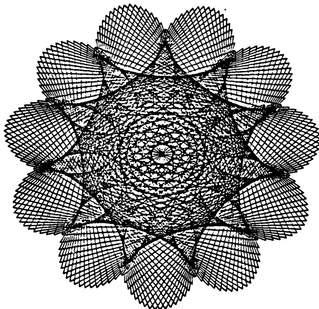
Figure 2.7 Symmetry: D_{11}
