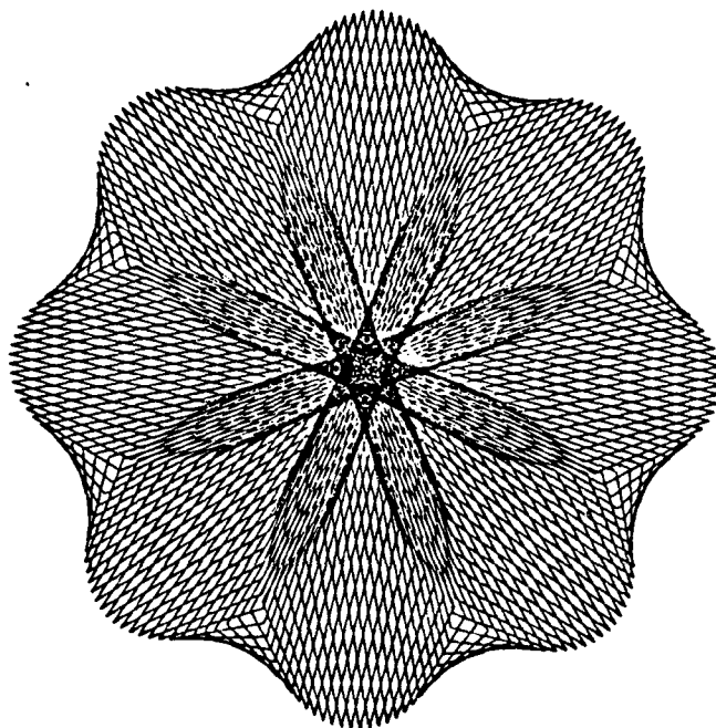
Figure 2.6 Symmetry: D_8
