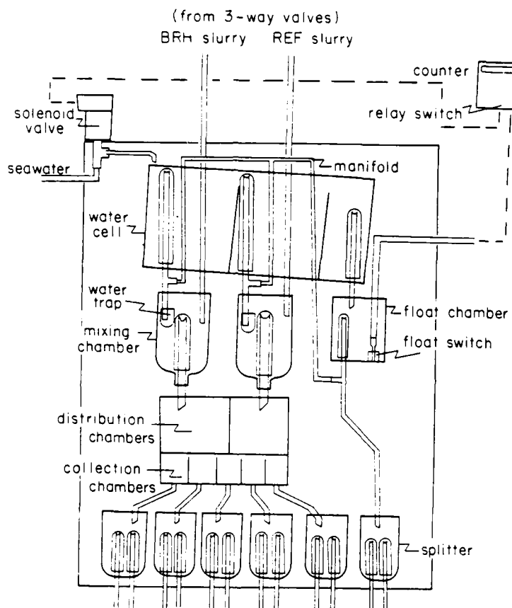
Figure 6. Proportional diluter used to deliver suspended sediment to the N. incisa exposure chambers
