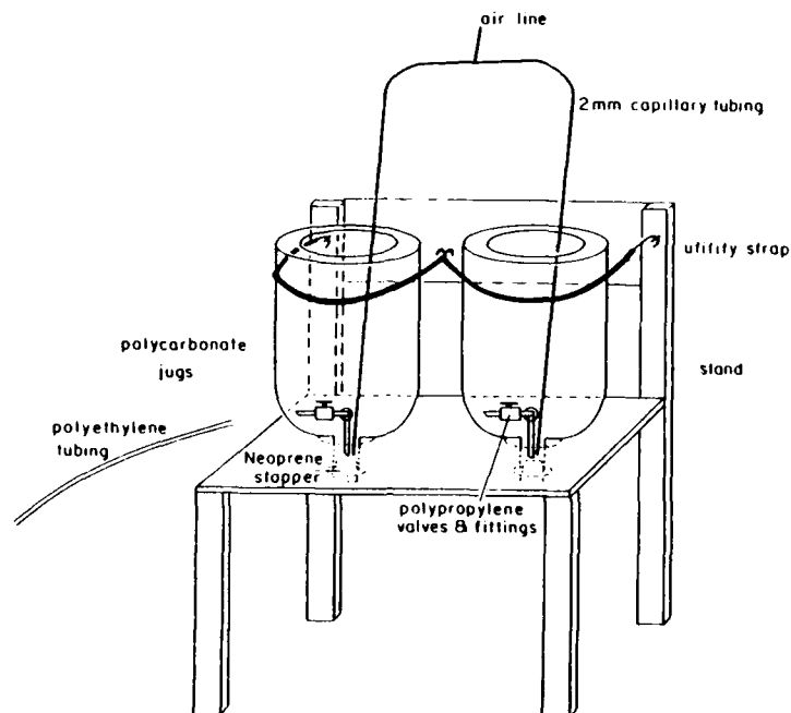
Figure 4. Suspended sediment oxidation system
