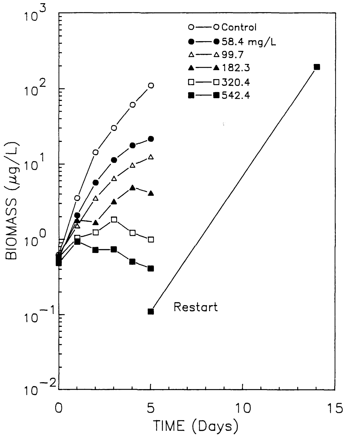
Figure 2. The effects of DEGDN on the growth of Selenastrum capricornutum as measured by biomass ( \mu\text{g/L} Chlorophylla). Restart was of rinsed cells in uncontaminated media.
