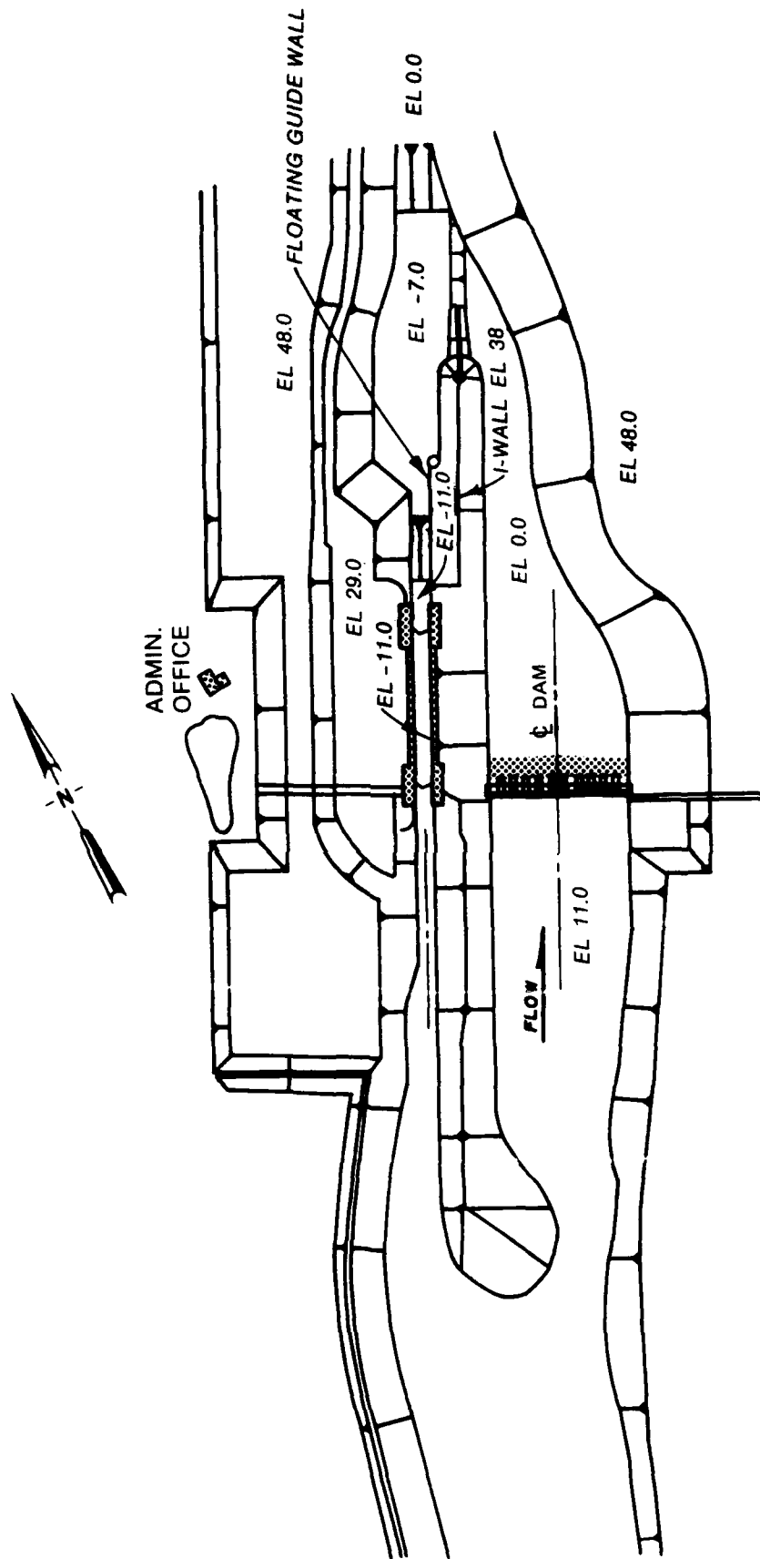
Figure 2. Red River Waterway Lock and Dam No. 1, as constructed
