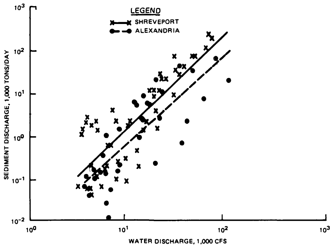
Figure 7. Suspended sand measurement at Alexandria and Shreveport, 1977-1978
