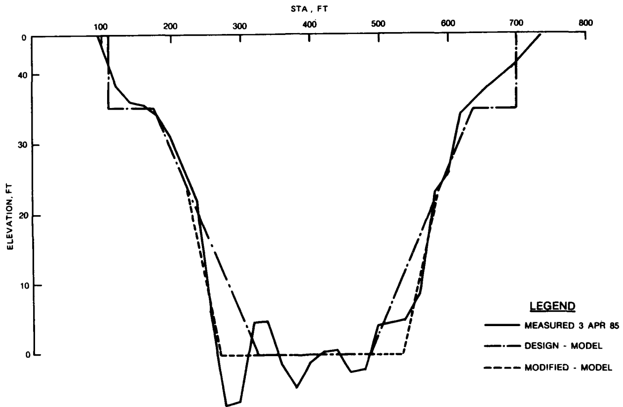
Figure 17. Exit channel cross section
