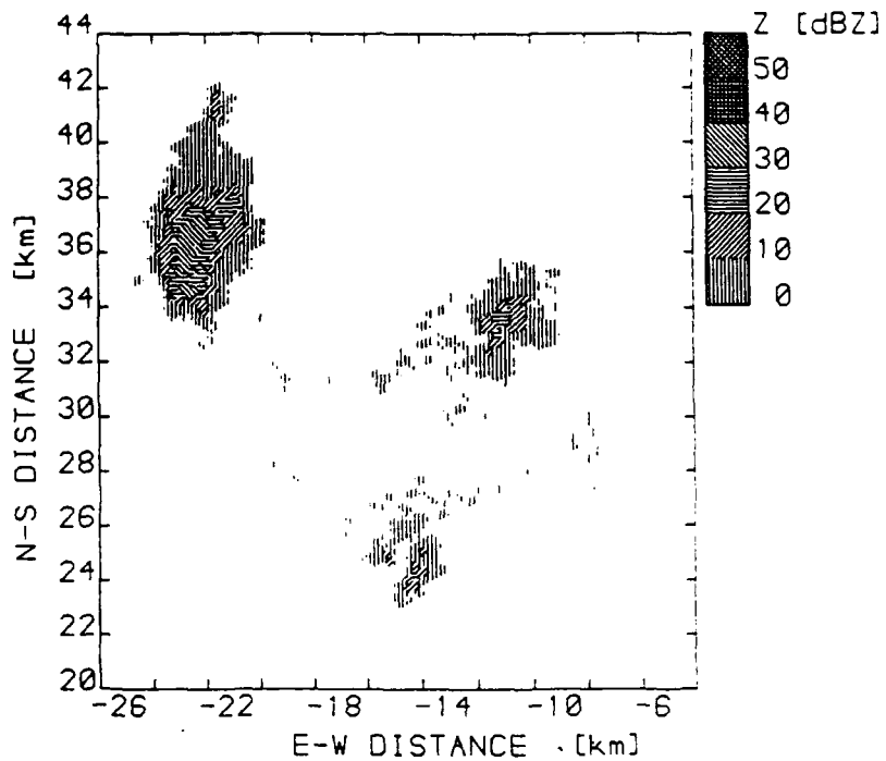
Figure 5 A 1° elevation PPI radar scan on 20 June 1984 at 1743 GMT showing various weak isolated echoes, two having anomalously high values of Z_{DR} .
