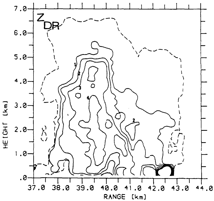
Figure 7 An RHI at 1641-10 through the cell in Figure 5 at azimuth 95° showing the development of a narrow column of positive ZDR above 4dB which extends almost 2km above the freezing level.
