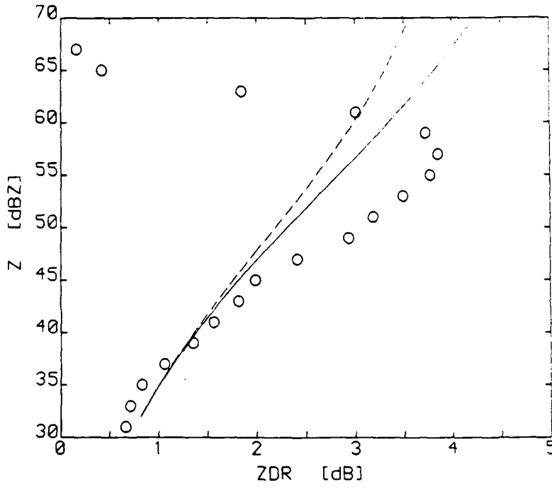
Figure 2. An example of the effect due to hail showing the significant decrease in ZDR at high Z values. The circles are averaged Chilbolton data from a storm on 6 July 1983 where a hail shaft was identified. The two lines are theoretical Z-ZDR relationships and are identical to those in Figure 1.
