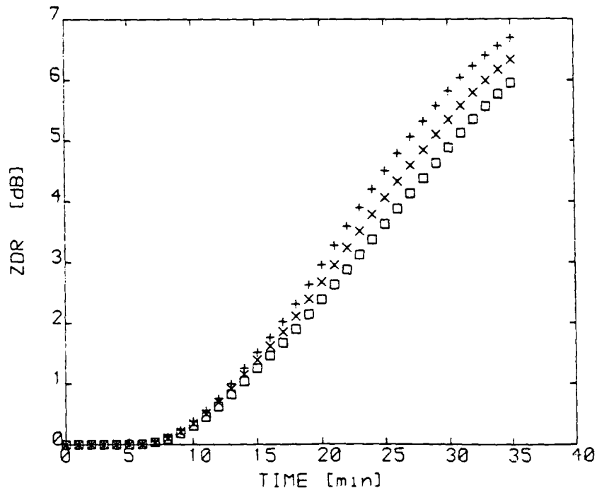
Figure 12 The growth of Z and Z DR with time as the three nucleus spectra capture cloud droplets of radius 6 μm and LWC 2 g m -3 . □, spectrum H; X, spectrum J; +, spectrum L.
