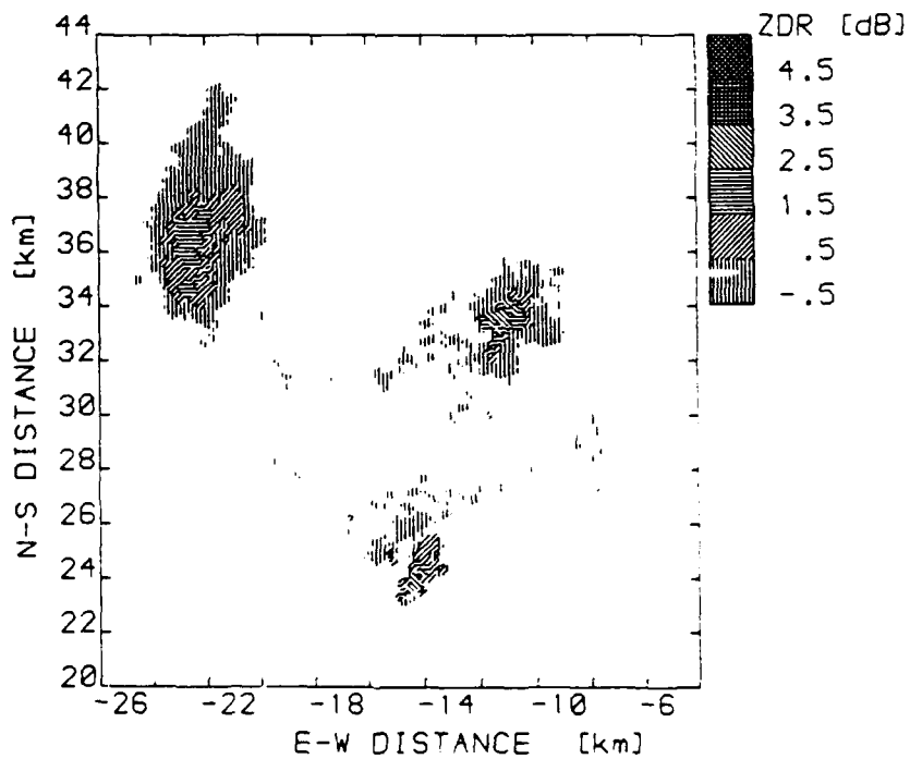
Figure 5 A 1° elevation PPI radar scan on 20 June 1984 at 1743 GMT showing various weak isolated echoes, two having anomalously high values of Z_{DR} .
