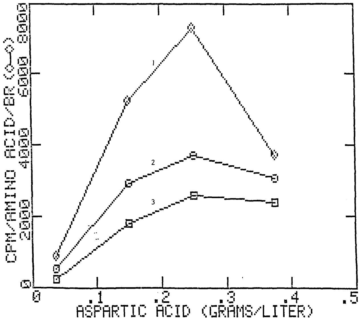
Figure 1. Incorporation of isotopic label derived from externally added 14 C-aspartic acid into the amino acid residues of bacteriorhodopsin. Uniformly labeled 14 C-asp was added to the synthetic growth medium of H. halobium JW-3 at the concentrations indicated. The cultures were grown for five days and the purple membrane fraction prepared by standard techniques. After delipidation of the isolated purple membrane, the bacteriorhodopsin was hydrolyzed in 6 N HCl at 110°C for 48 hr. The resulting amino acid mixture was derivatized with phenylisothiocyanate and separated using a reverse phase HPLC column. Fractions were collected and counted for radioactivity. The counts were corrected for the initial specific activity of the added aspartic acid, and normalized to the relative amount of each amino acid found both in the HPLC chromatogram and in the known amino acid content of bacteriorhodopsin. Radioactivity was found only in the fractions corresponding to aspartic acid (1), glutamic acid (2) and threonine (3).
