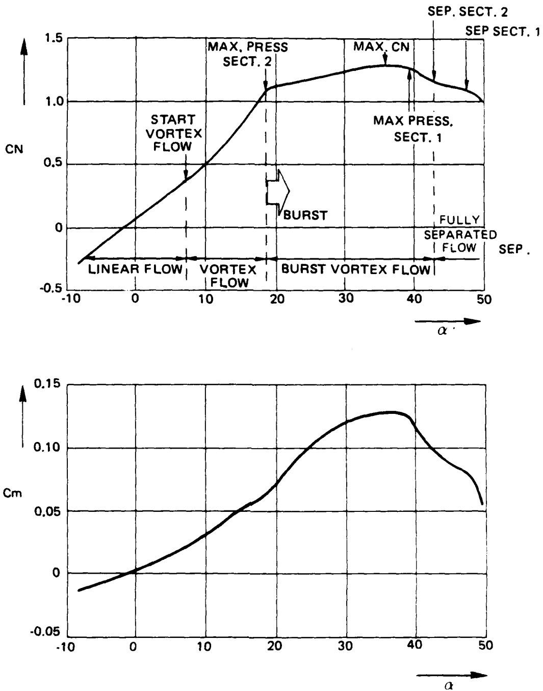
Fig. 11 Steady normal force and pitching moment coefficient vs. incidence
