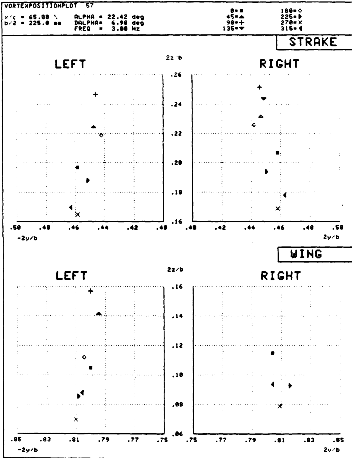
Fig. 40 Time history of the vortex core positions at section 2 ( \alpha = 22.42 \text{ deg} , d\alpha = 6.98 \text{ deg} , f = 3 \text{ Hz} )
