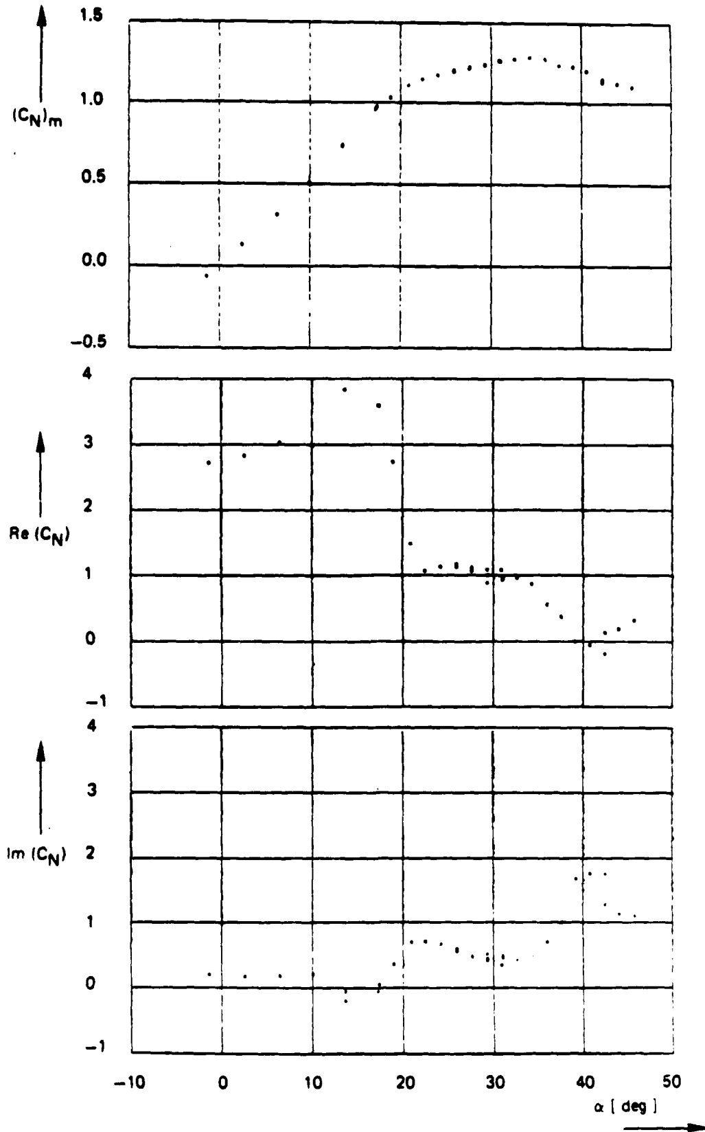
Fig. 17 Zeroth and first order harmonic components of unsteady normal force coefficient ( da \approx 3.5 deg, f = 3 Hz, \beta = 0 deg, V \approx 80 m/s)
