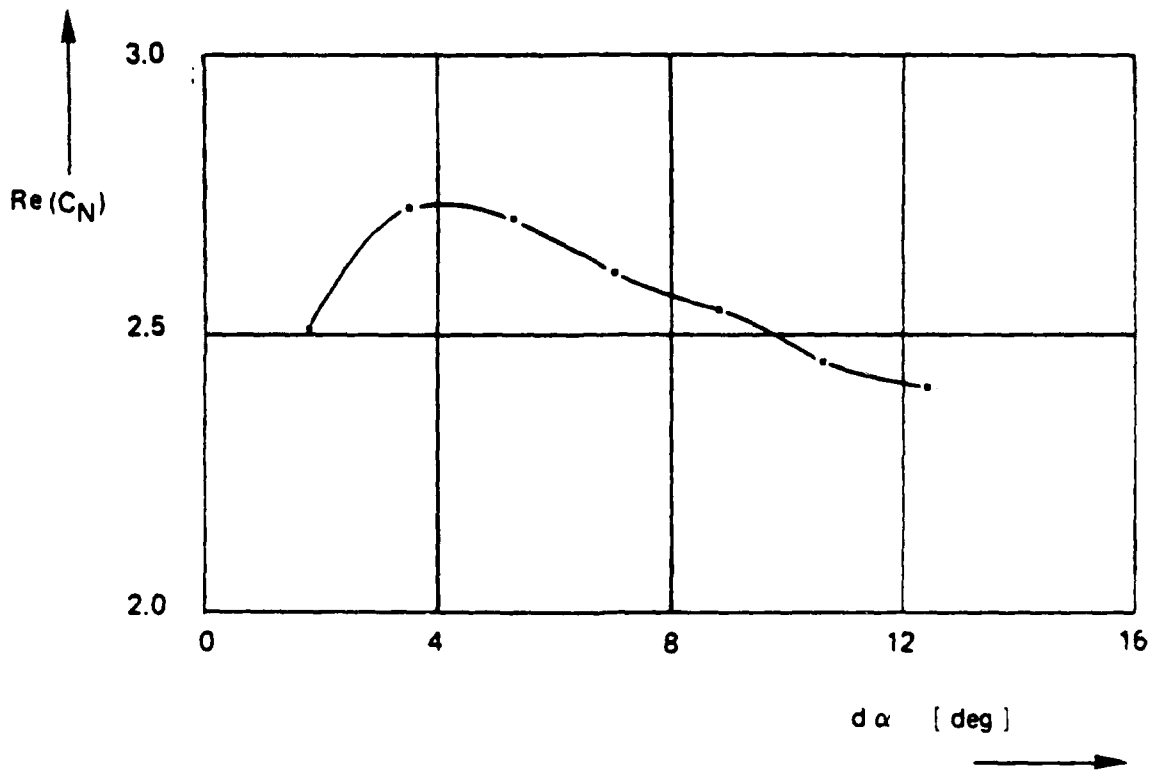
Fig. 22 Zeroth order harmonic component and real part of first order harmonic component of unsteady normal force coefficient vs. amplitude ( \alpha \approx 18.9 deg, f = 3 Hz, \beta = 0 deg, V \approx 80 m/s)
