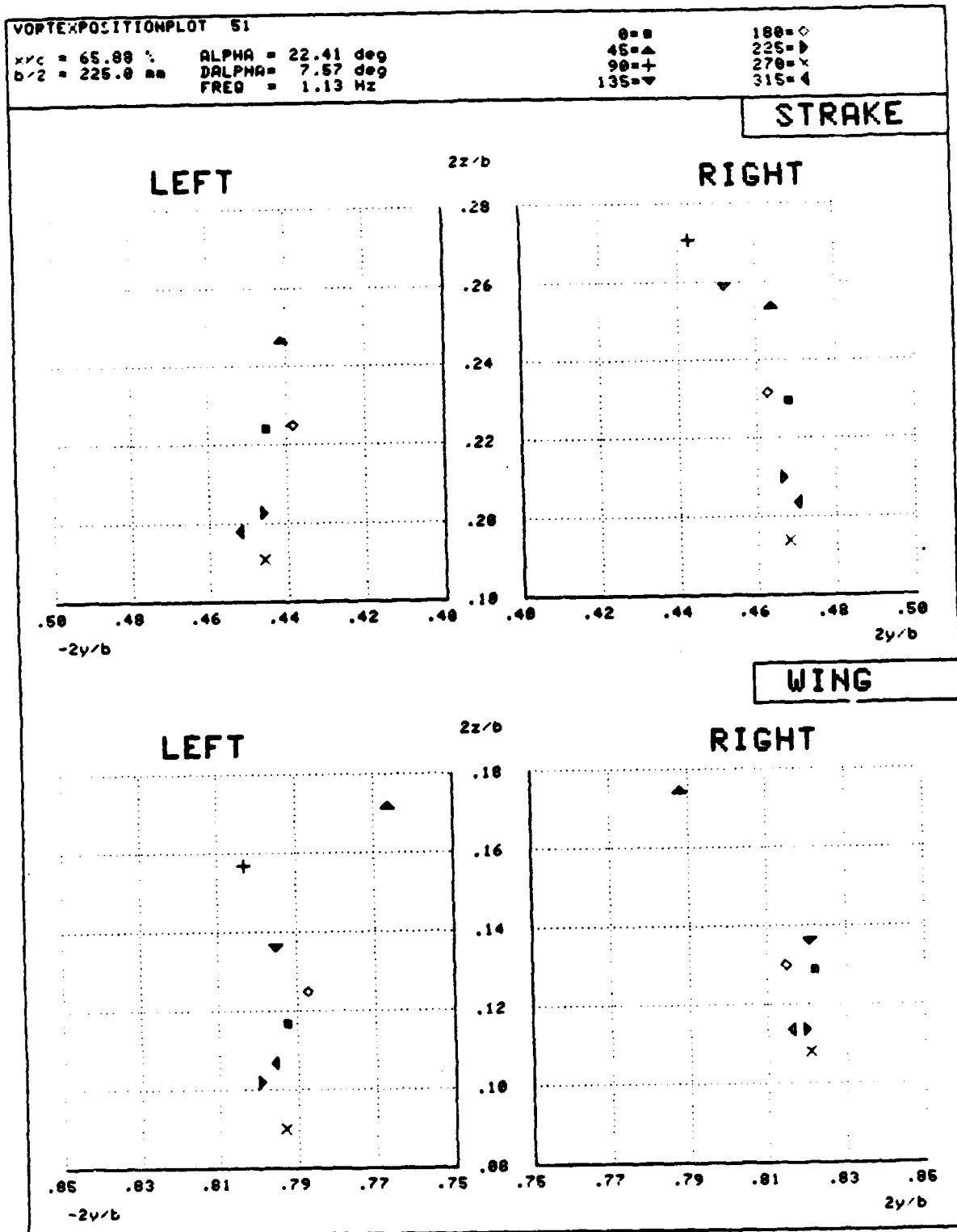
Fig. 38 Time history of the vortex core positions at section 2 ( \alpha = 22.41 deg, \delta\alpha = 7.57 deg, f = 1.13 Hz)
