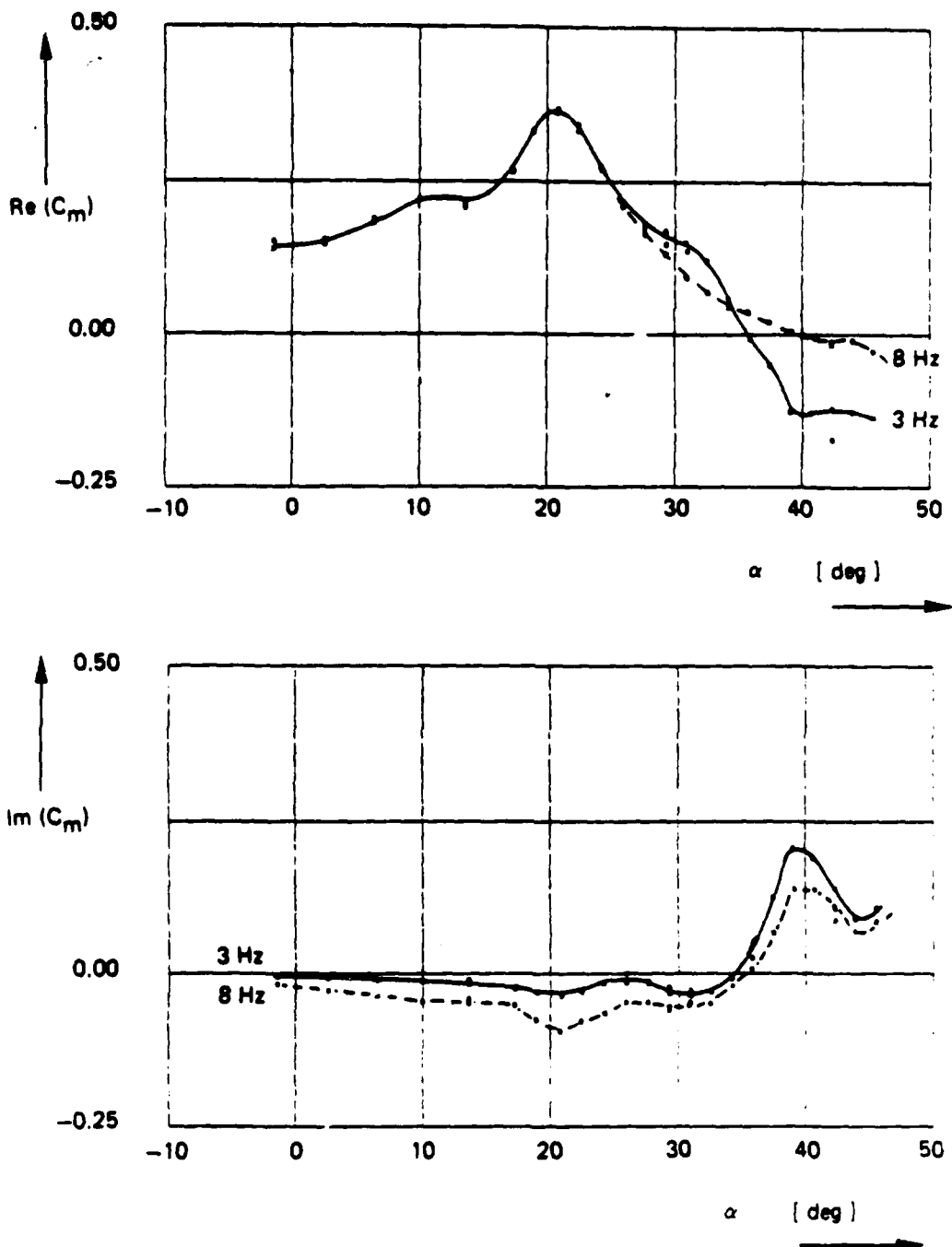
Fig. 19 First order harmonic components of unsteady pitching moment coefficients at 3 and 8 Hz ( da \approx 3.5 deg, \beta = 0 deg, V \approx 80 m/s)
