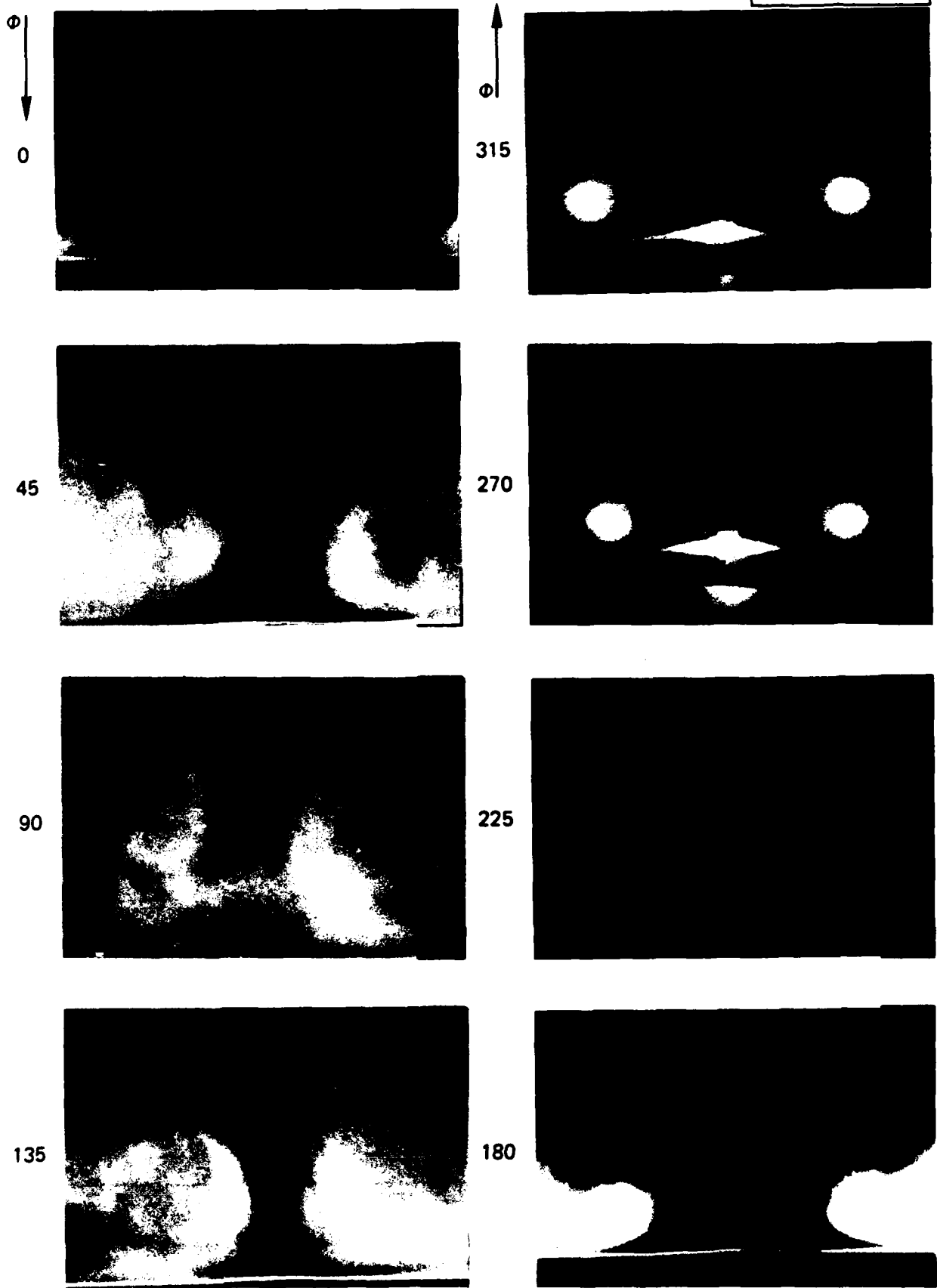
Fig. 43 Photographs showing the time history of the flow at section 3 ( \alpha = 22.29 \text{ deg} , d\alpha = 15.19 \text{ deg} , f = 1.13 \text{ Hz} )
