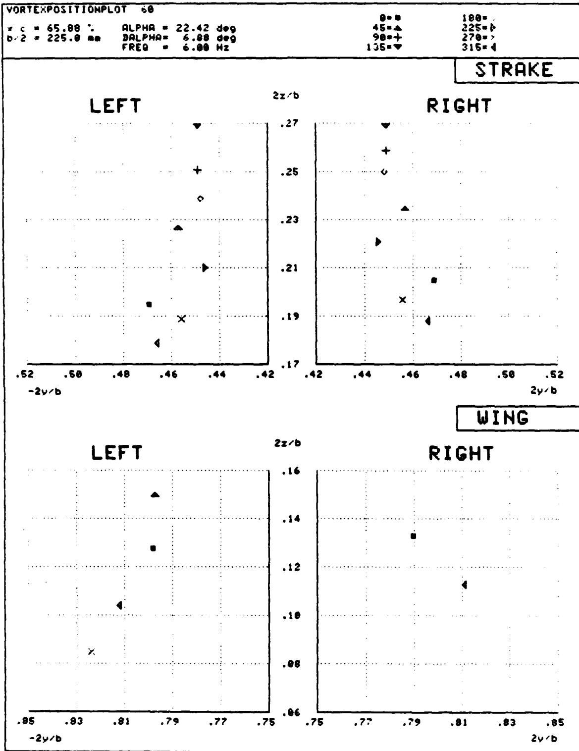
Fig. 42 Time history of the vortex core positions at section 2 ( \alpha = 22.42 deg, d_\alpha = 6.88 deg, f = 6 Hz)
