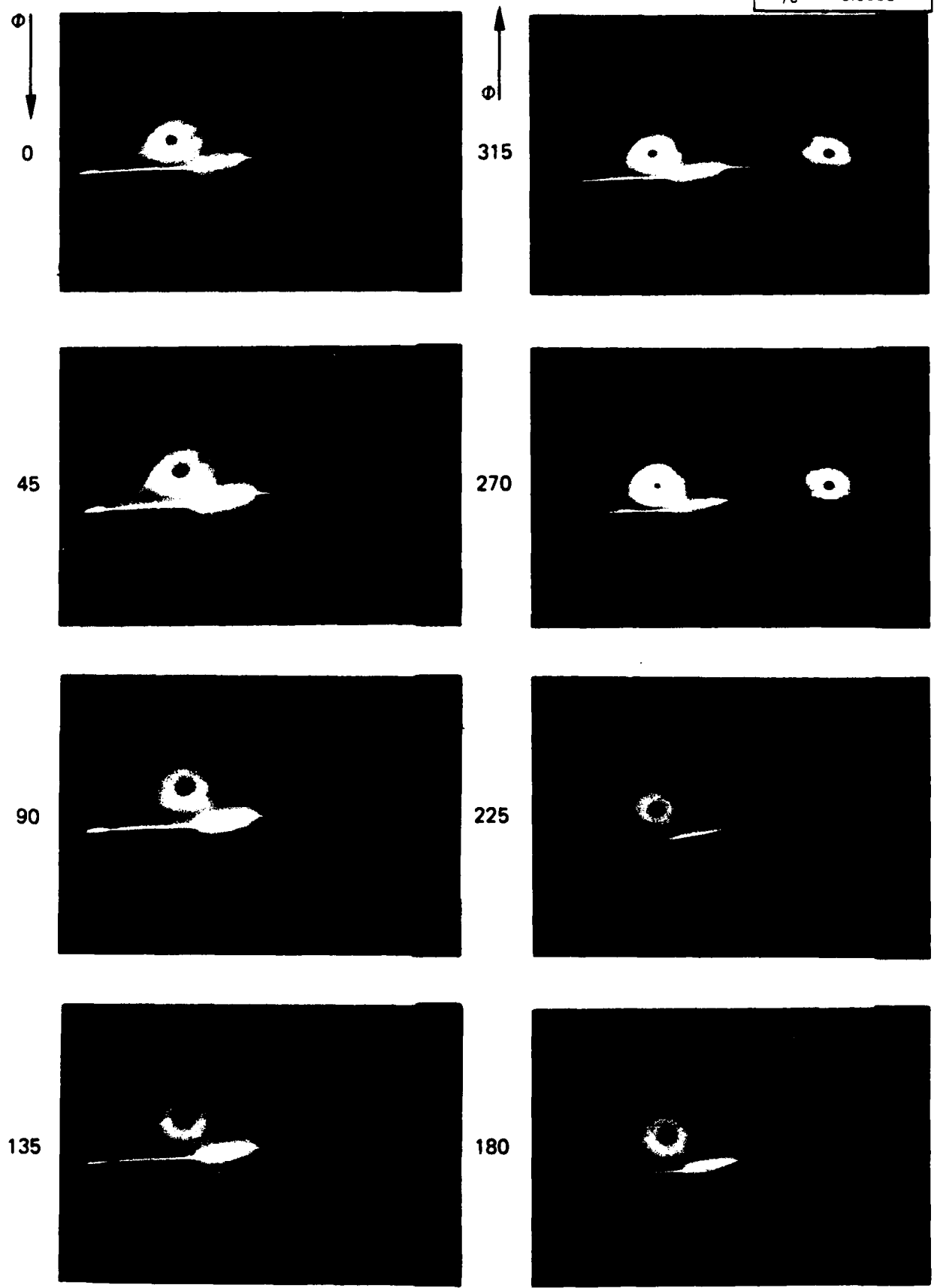
Fig. 41 Photographs showing the time history of the flow at section 2 ( \alpha = 22.42 \text{ deg} , d\alpha = 6.88 \text{ deg} , f = 6 \text{ Hz} )
