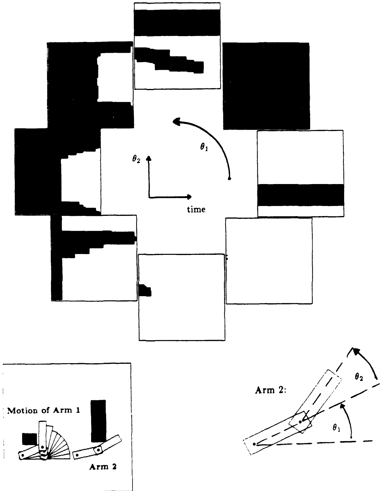
Figure 28 Several slices of the configuration space-time representing the constraints imposed on the right arm by the motion of the left arm and by the stationary obstacles in the environment. Each slice depicts the constraints imposed on Link 2 for a fixed orientation of Link 1.
