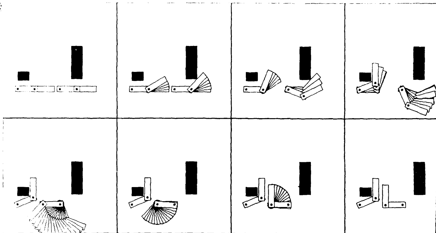
Figure 26. Some sample snapshots of the motions determined by the planner while solving the problem of Figure 25.
