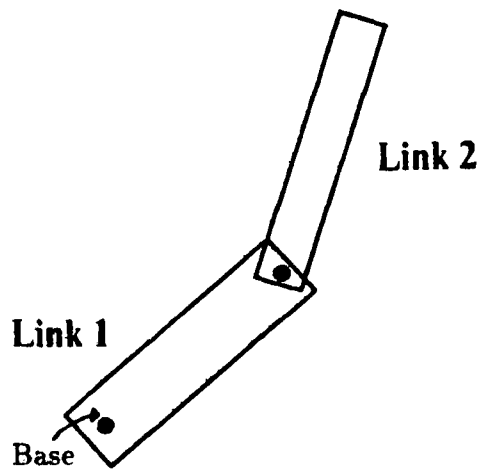
Figure 21. A two-link arm. The arm has two rotational degrees of freedom. The arm's base is fixed in the plane.
