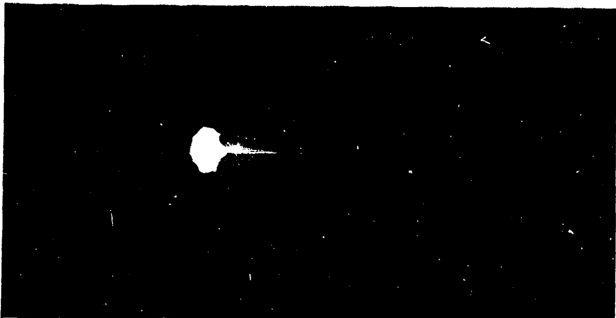
Figure 19. Ball, Tracer Flash Geometry, Short Burst
