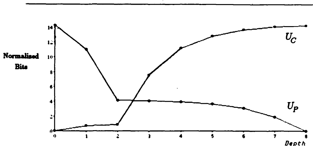
Figure 4.14: The evaluation curves for the ordered taxonomy. Plotted are U_P and the normalized U_C as a function depth. For the structured case of the ordered taxonomy the level at which the species of leaves are separated — level 2 — shows a marked break in both U_P and U_C .
