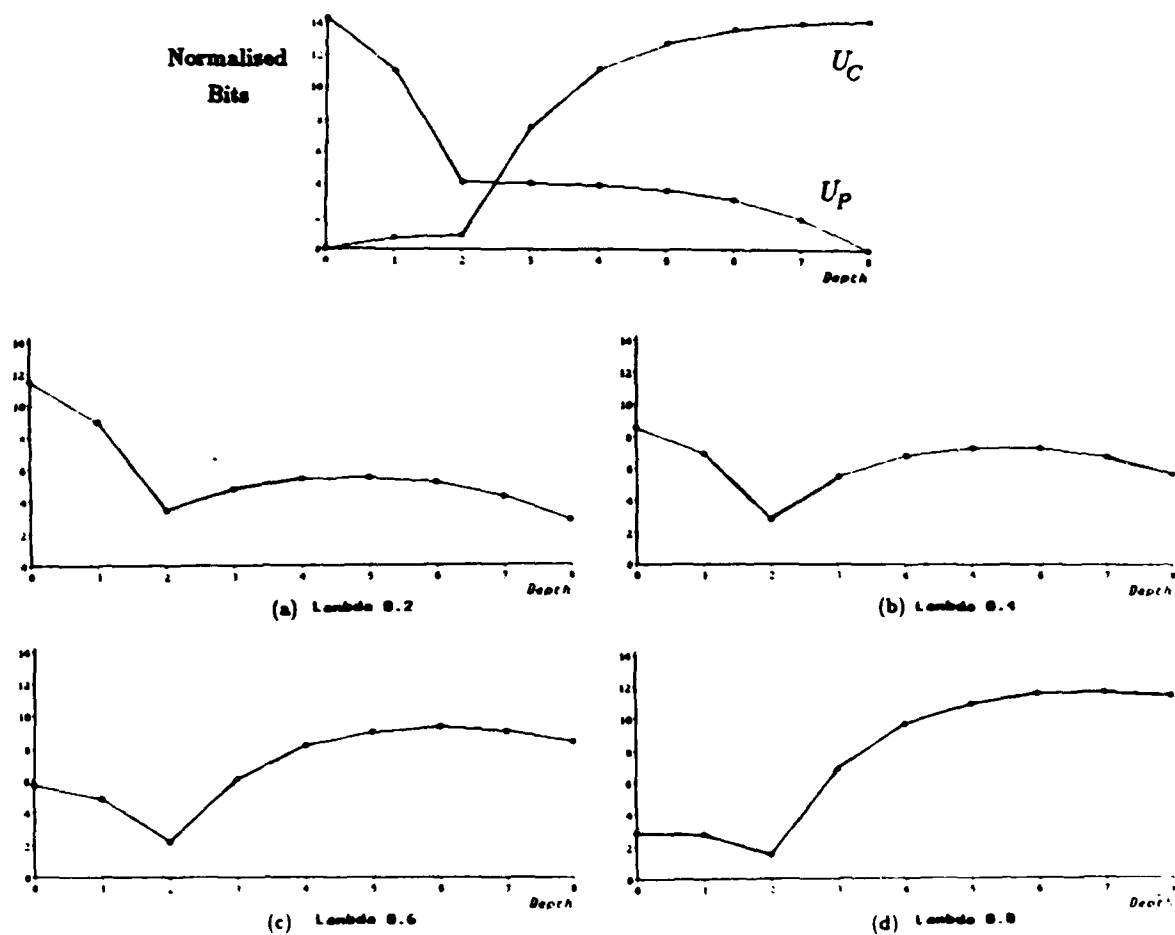
Figure 4.18: Graphs of U = (1 - \lambda)U_P + \lambda U_C for the ordered taxonomy. Top plot is original vales of U_P and normalized U_C . The four panels a-d are for \lambda of .2, .4, .6, and .8 respectively.
