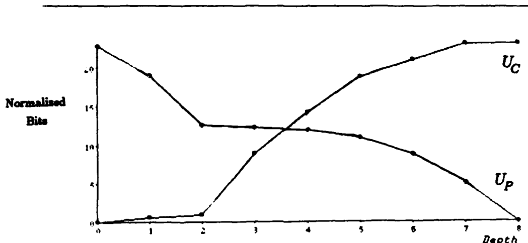
Figure 4.15: The evaluation curves for the ordered taxonomy, but with the addition of four noise features. Both U_P and the normalized U_C show a definite break at level 2 — the level corresponding to the separate species — but the curves are becoming more like those of the jumbled evaluation.
